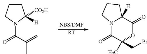
(3R,8aR)-3-Bromomethyl-3-methyl-tetrahydro-pyrrolo[2,1-c][1,4]oxazine-1,4-dione
