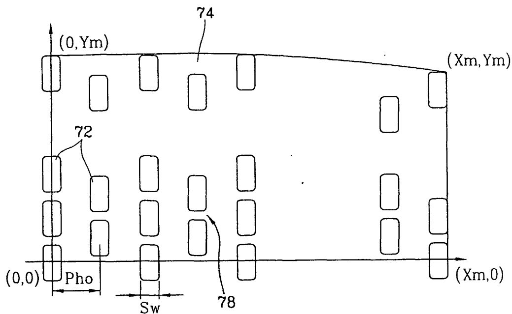
FIG. 3 CONVENTIONAL ART
