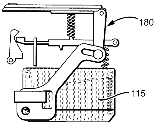
REST POSITION
