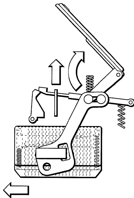
LEVER PULLED TO COCK HAMMER AND ADVANCE CASSETTE TO NEXT LANCET
