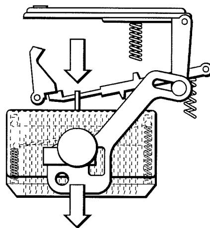
BUTTON IS PRESSED TO RELEASE HAMMER AND PROJECT LANCET
