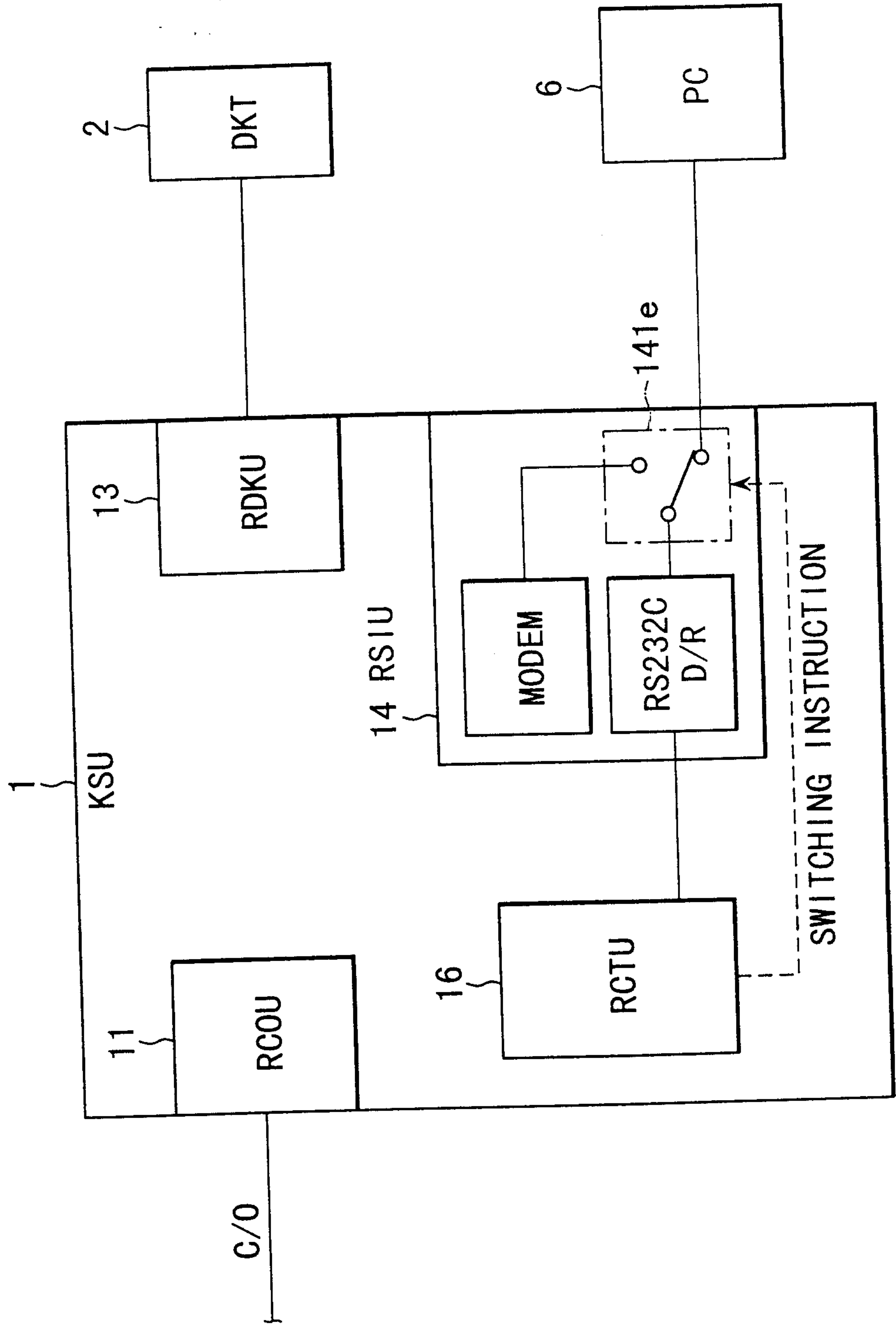
CONNECTION USING RS232C INTERFACE
