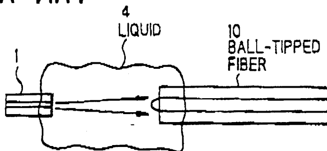
FIG. 1C PRIOR ART
