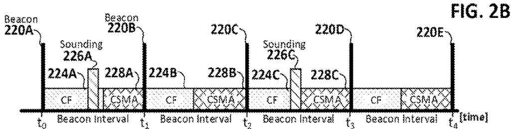
PRIOR ART WLAN Activity
