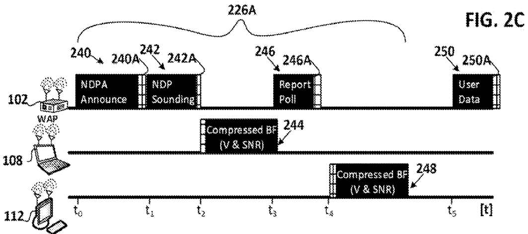
PRIOR ART WLAN Sounding
