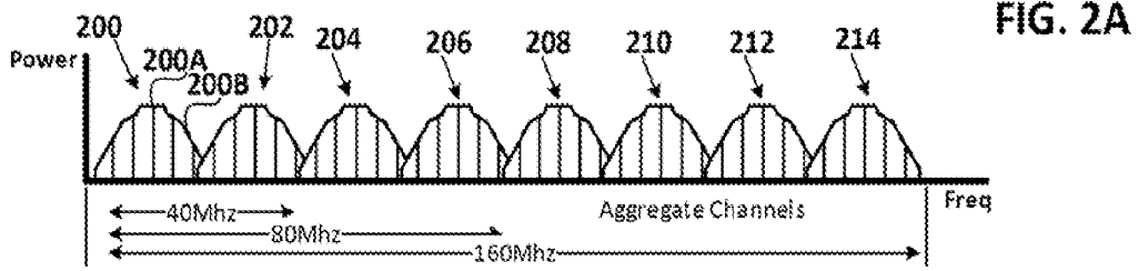
PRIOR ART WLAN Channels
