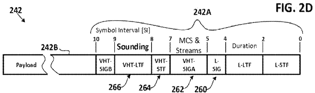
PRIOR ART WLAN Packet Header
