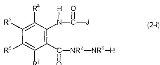
[Chemical Formula 17]
