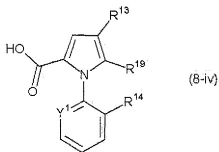
[Chemical Formula 35]
