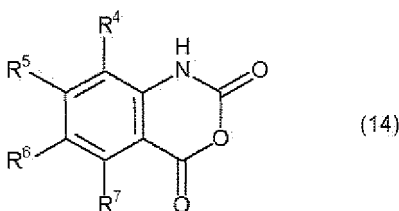
[Chemical Formula 20]
