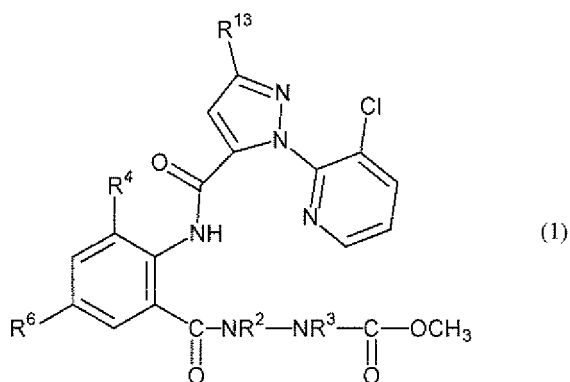
[Chemical Formula 168]
