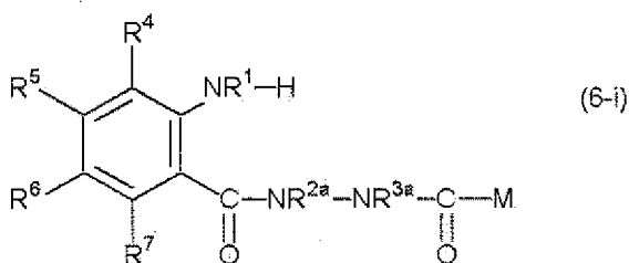
[Chemical Formula 9]
