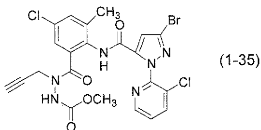
[Chemical Formula 151]
