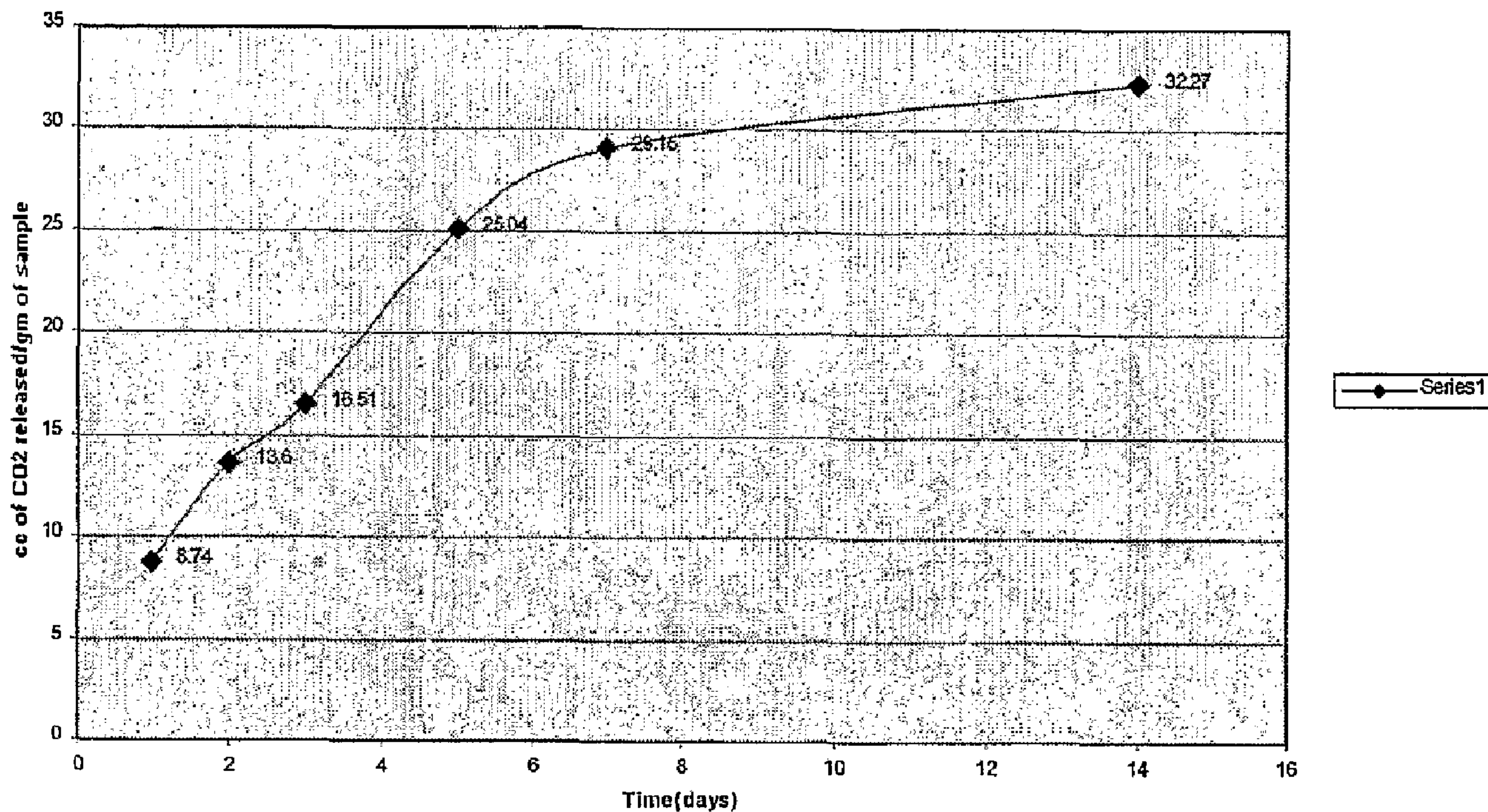
cc of CO2 released / gm of sample Vs Time (days)
