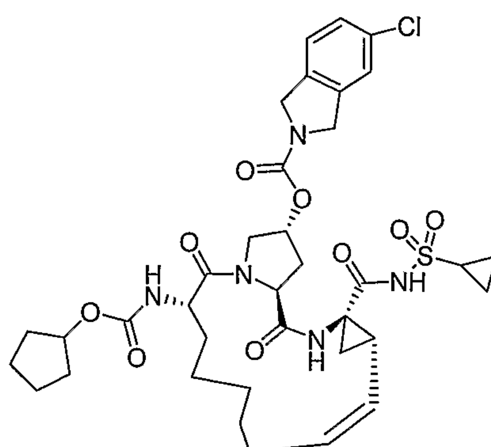
Compound AR00334218
