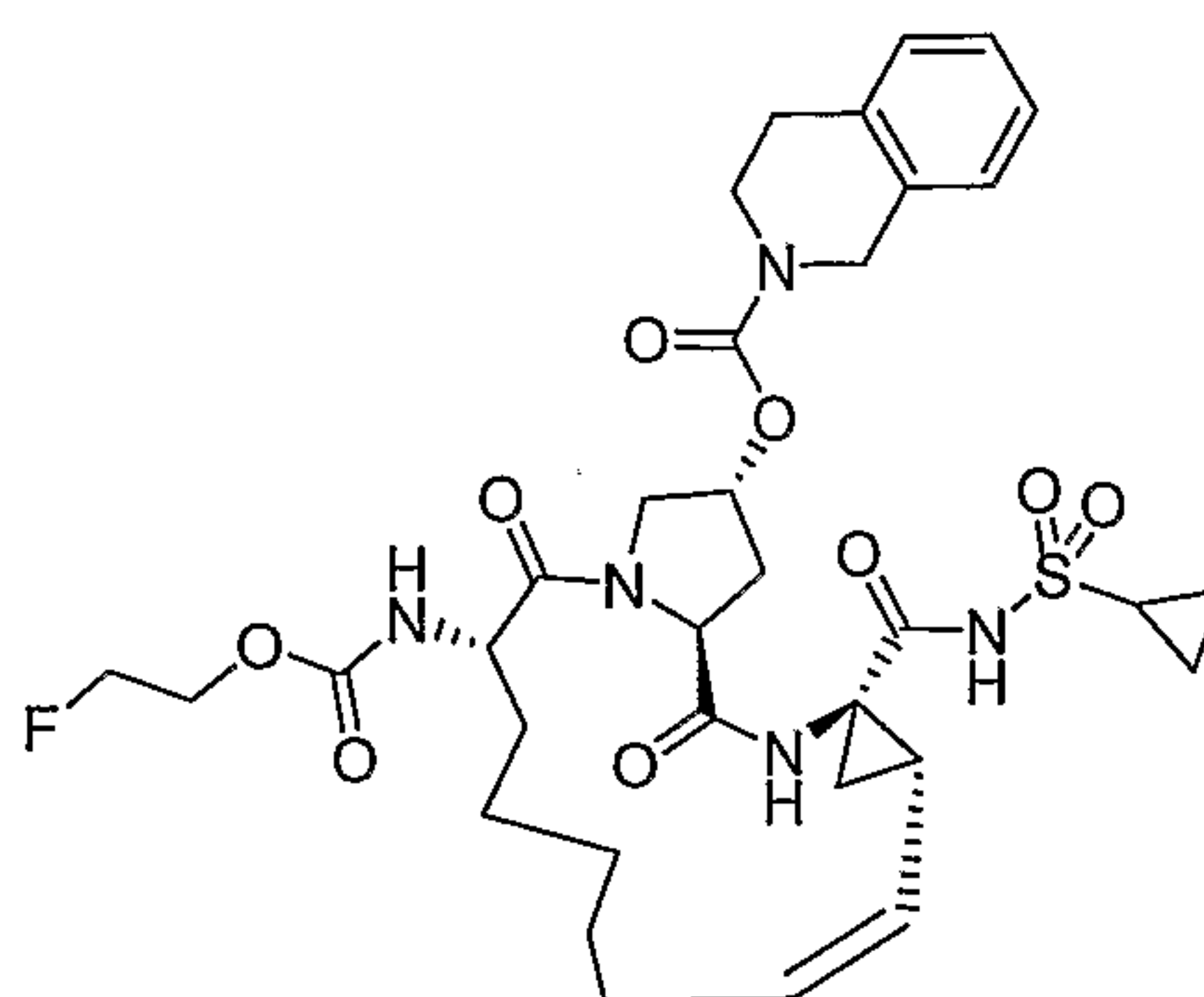
Compound AR00304161
