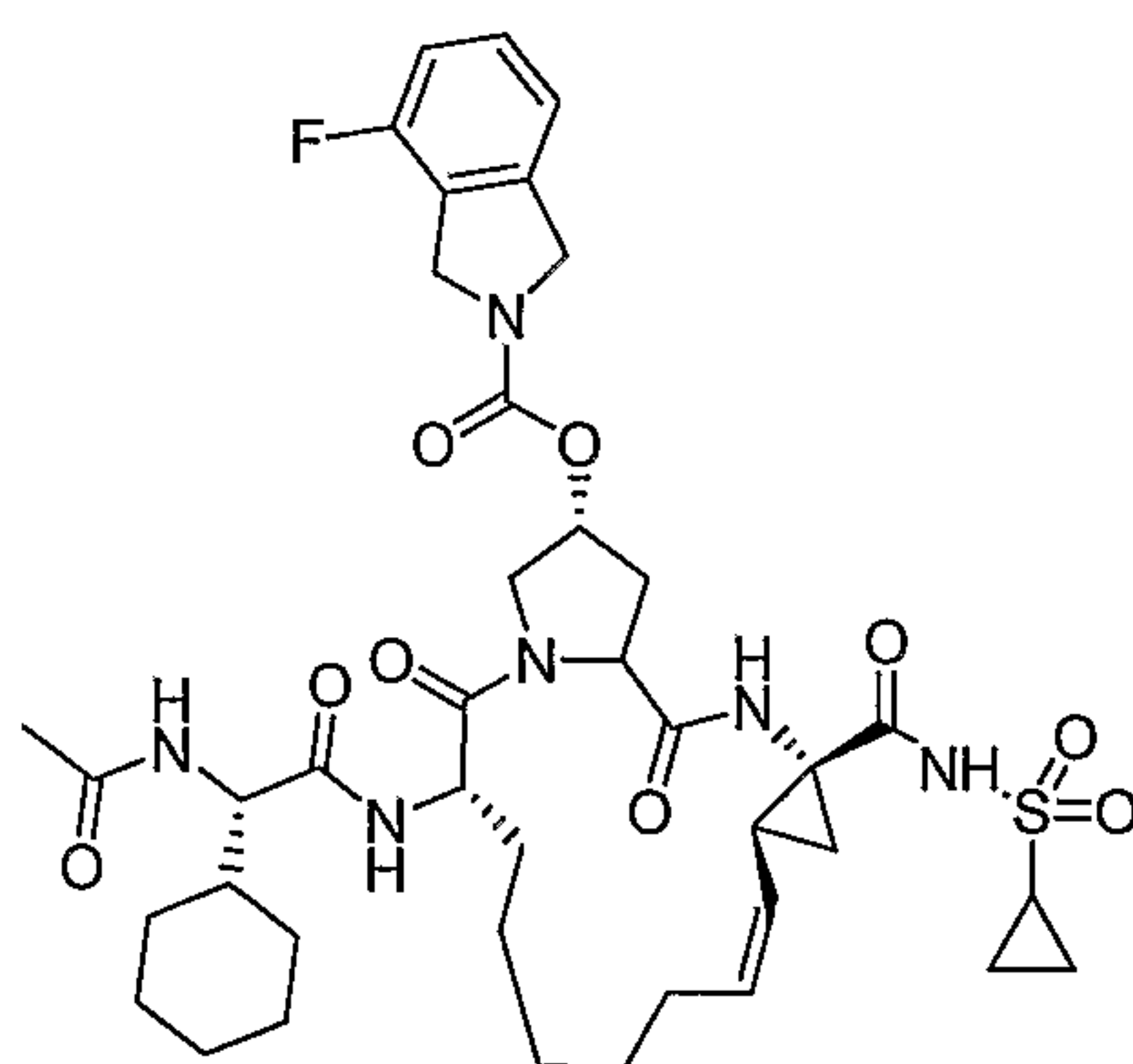
Compound AR00340122
