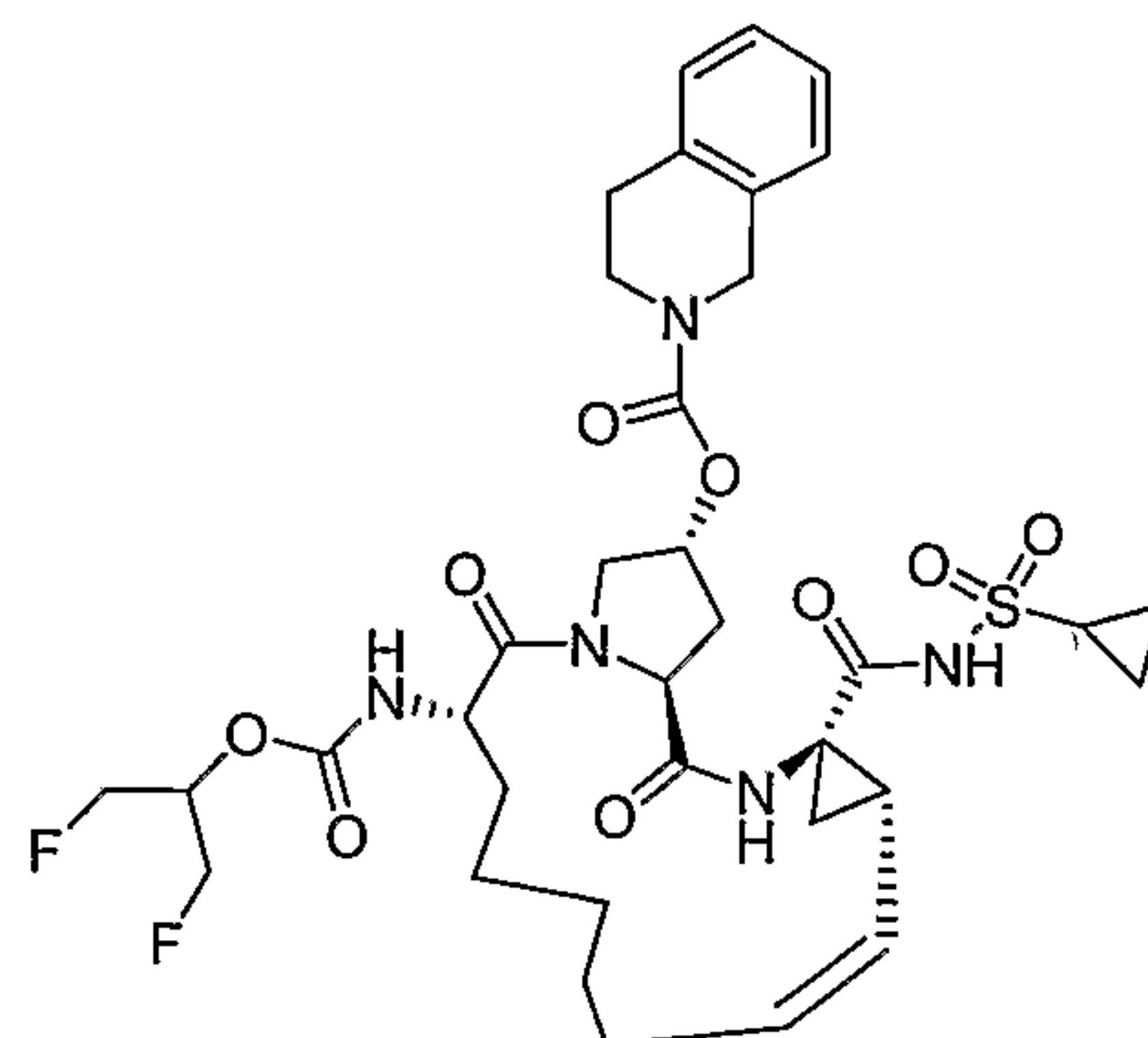
Compound AR00320580
