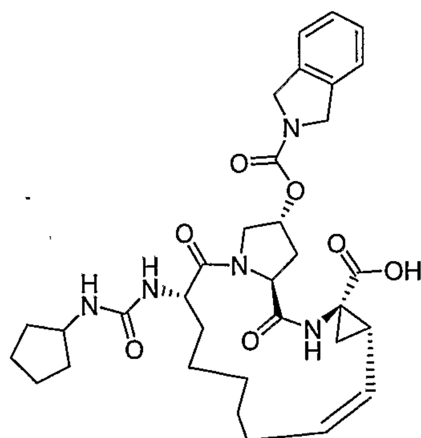
Compound AR00304079
