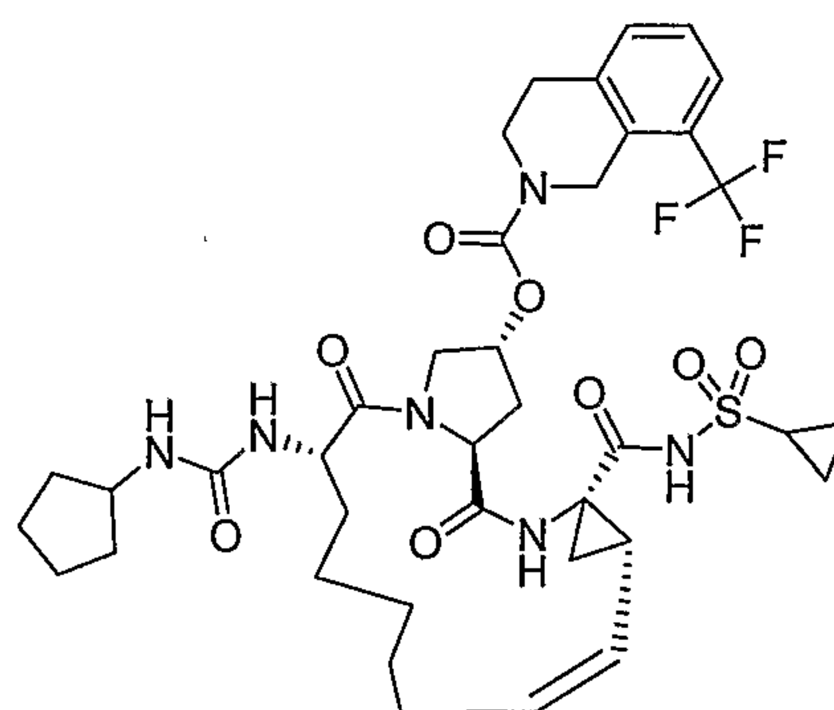
Compound AR00304081
