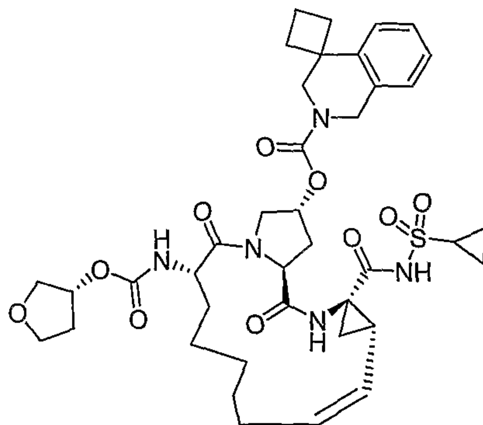
Compound AR00314635
