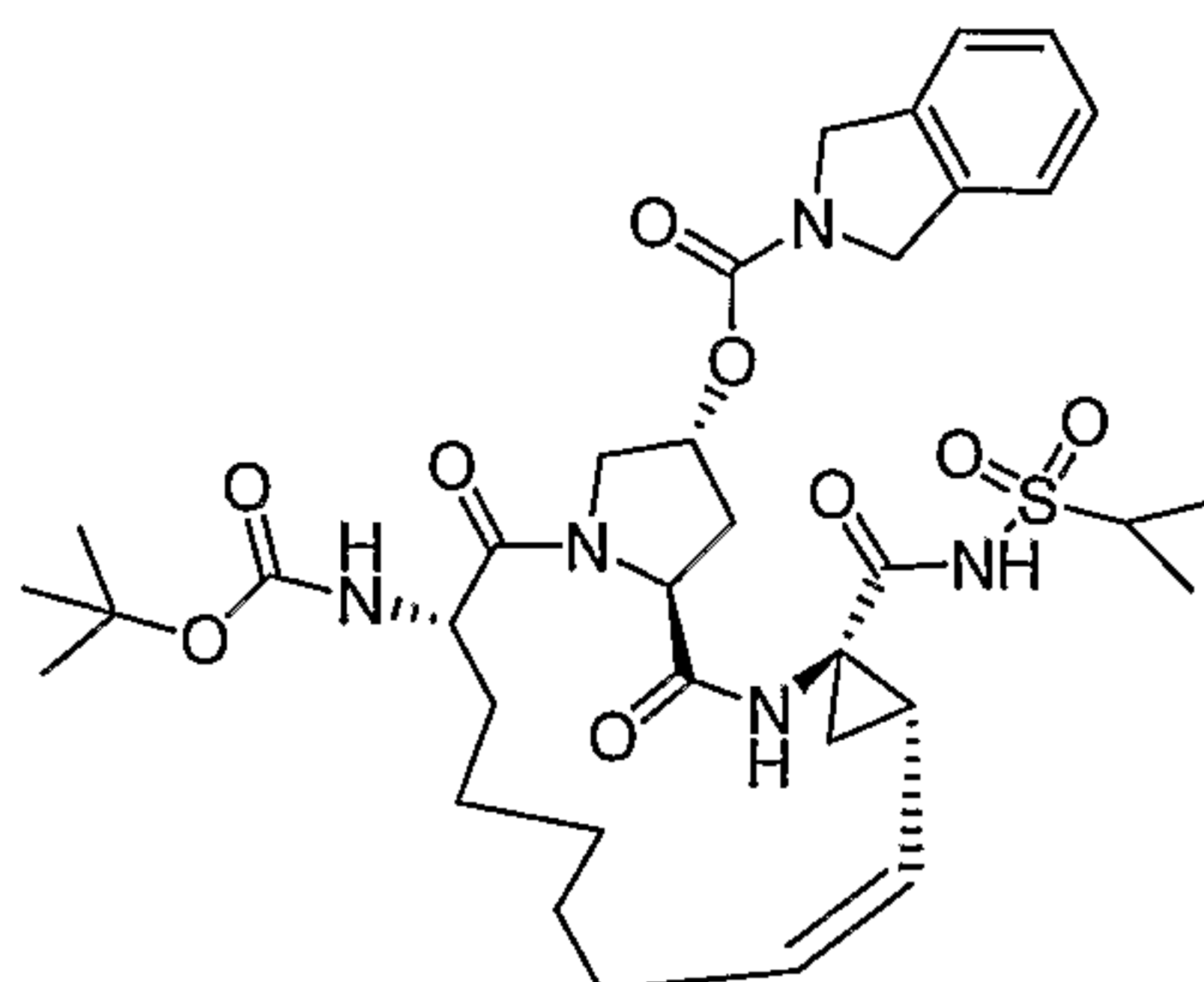
Compound AR00333801
