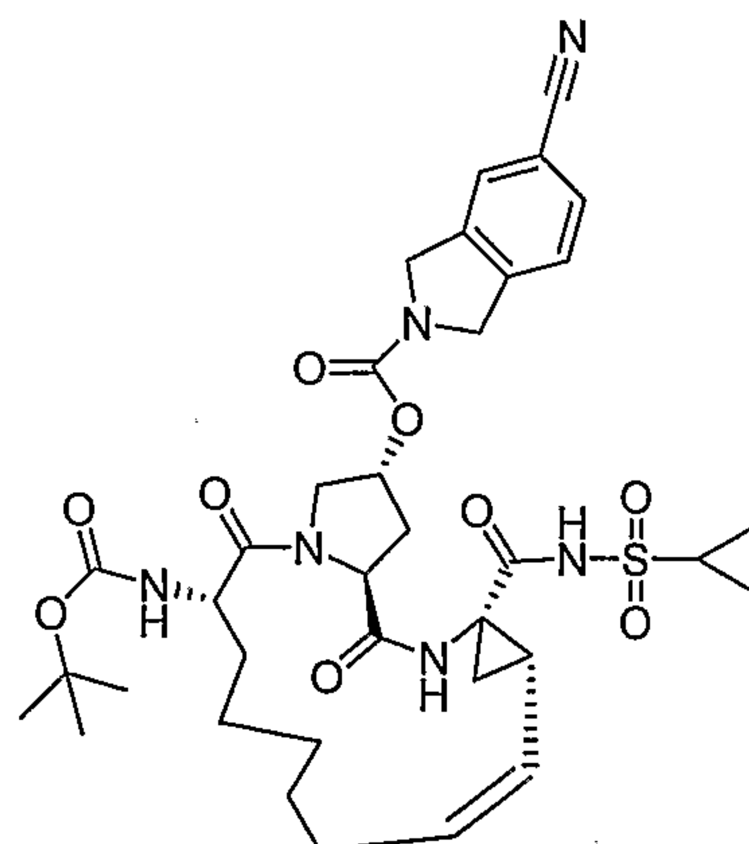
Compound AR00365082
