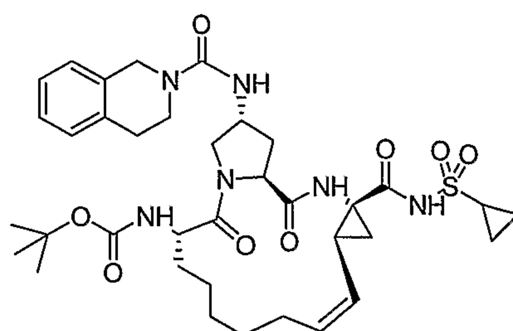
Compound AR00287266
