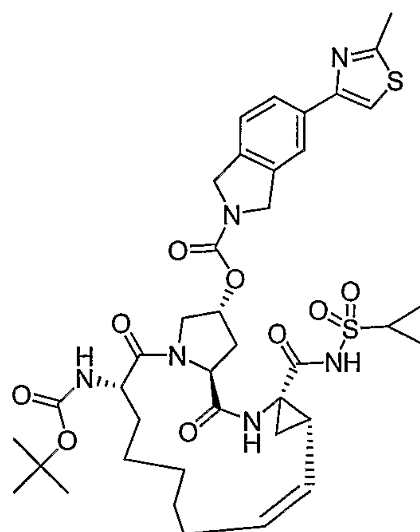
Compound AR00364989
