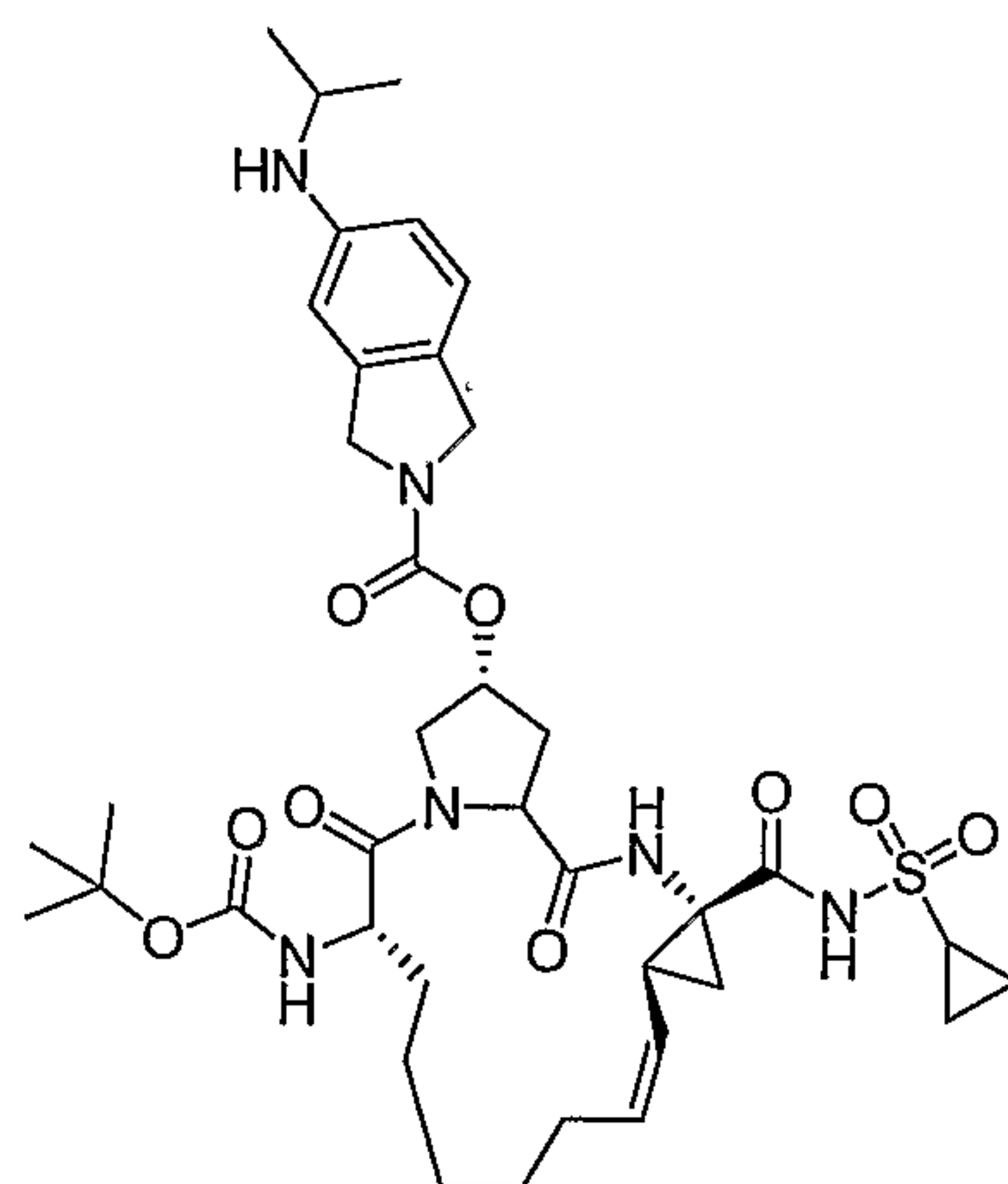
Compound AR00341649
