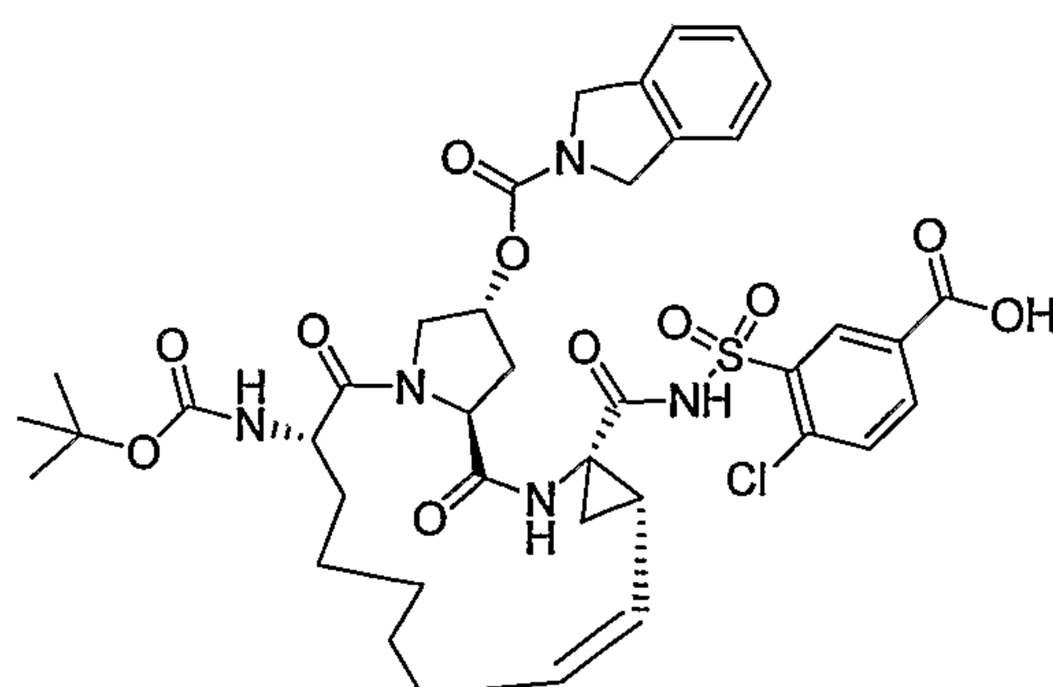
Compound AR00365388
