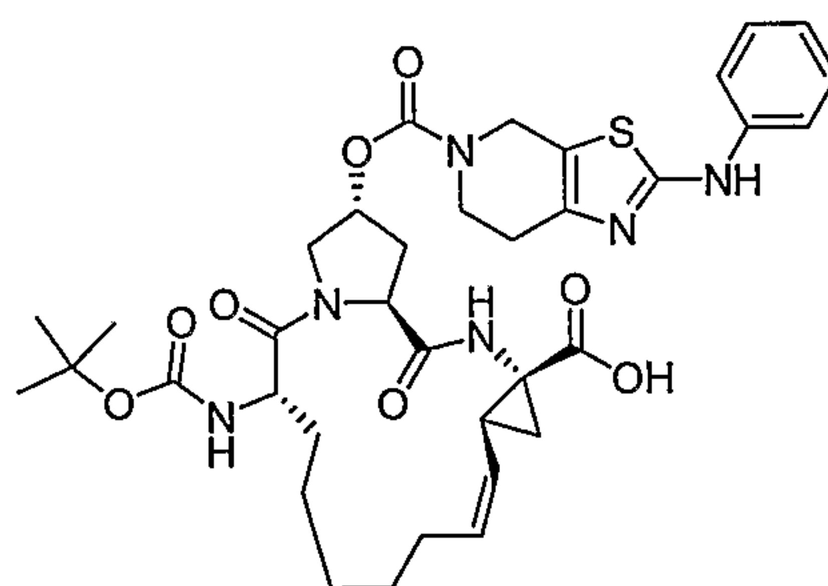
Compound AR00304000
