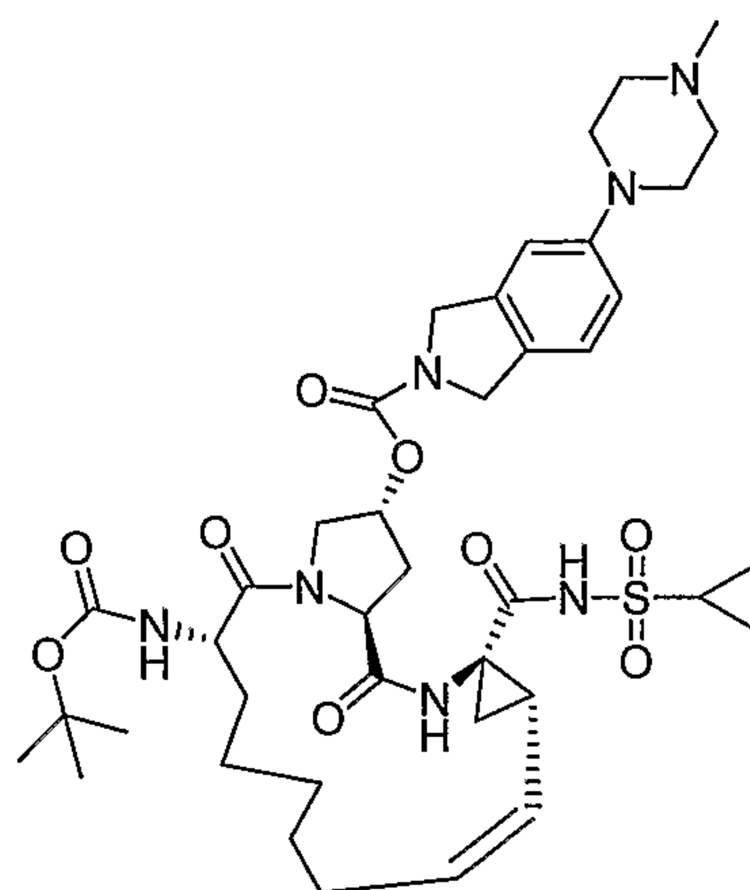
Compound AR00340495
