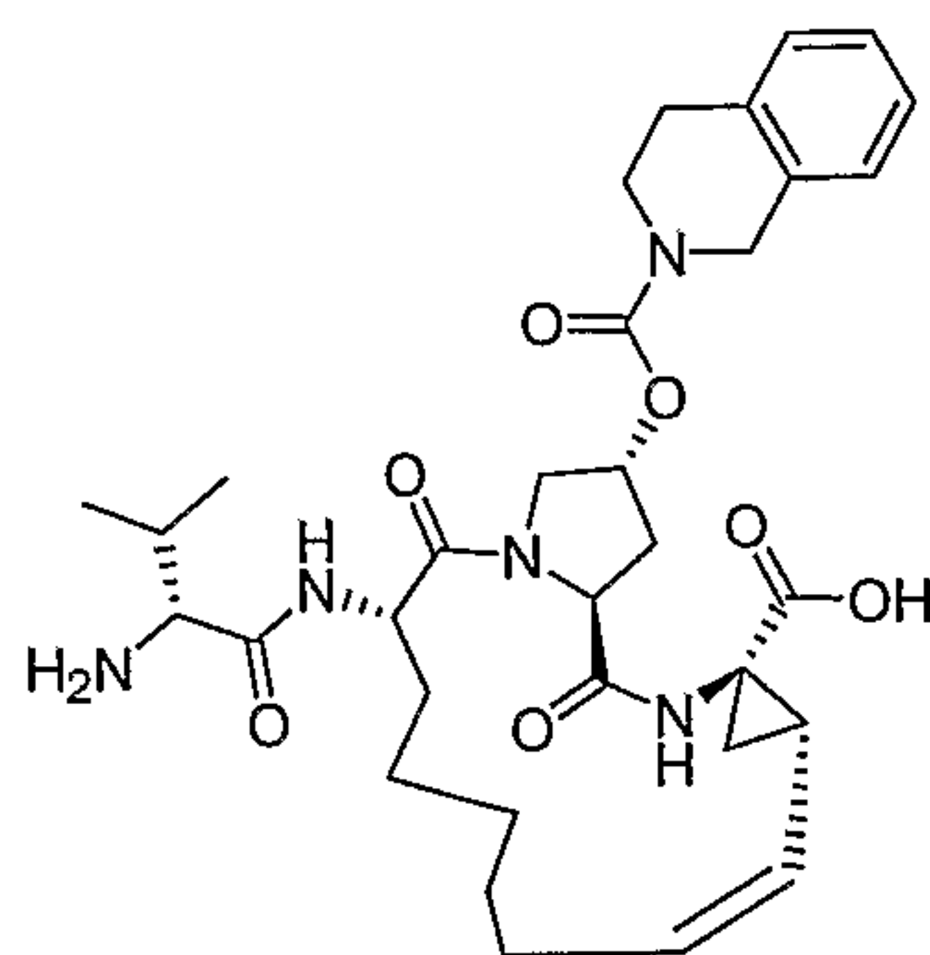
Compound AR00298990
