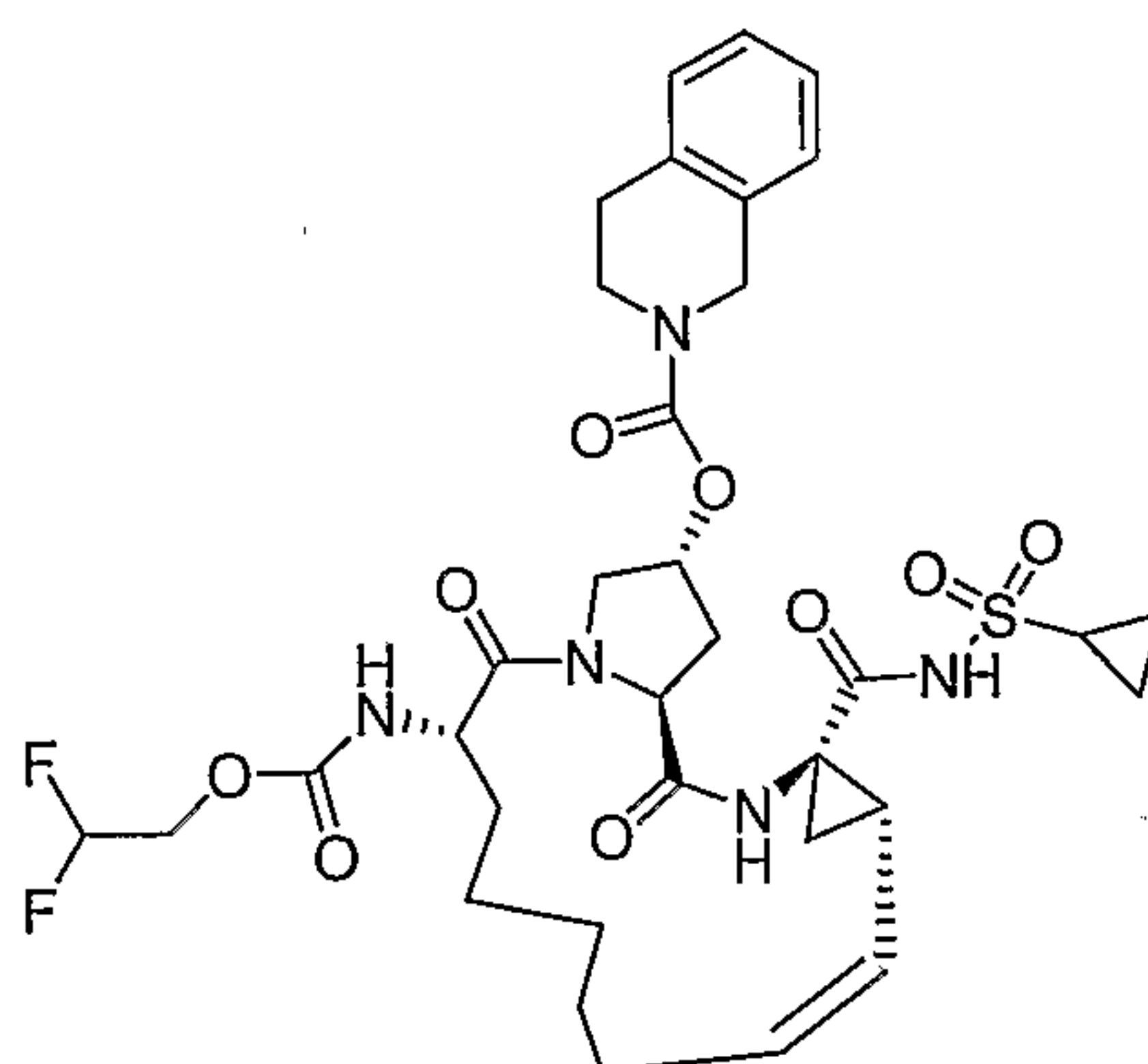
Compound AR00320579
