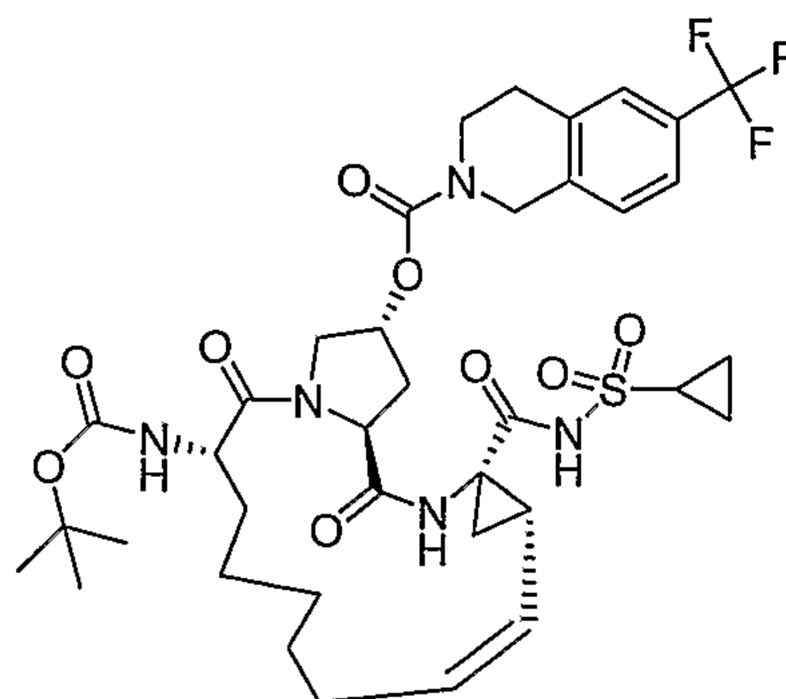
Compound AR00301747
