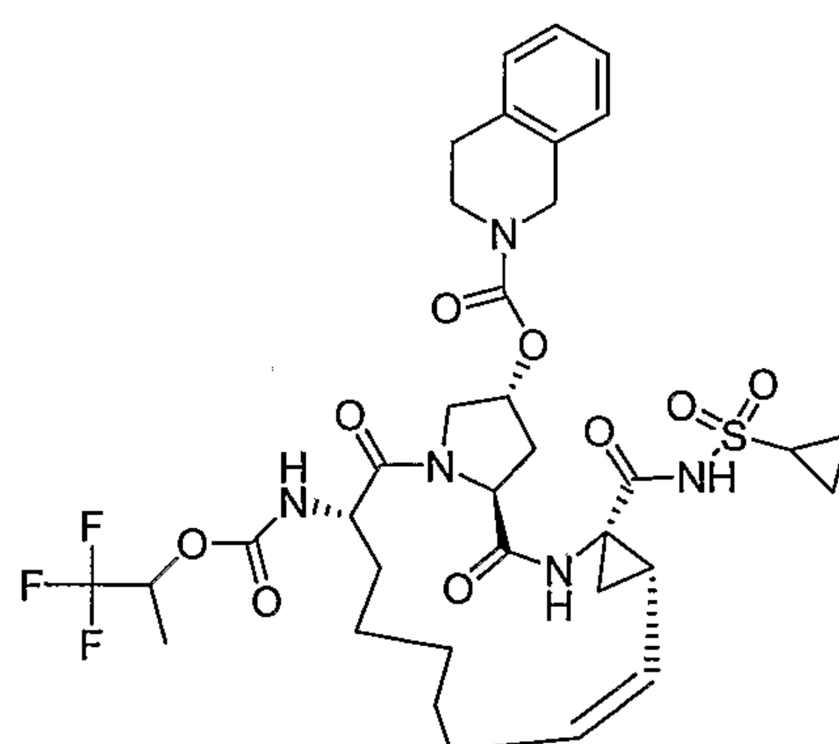
Compound AR00320581
