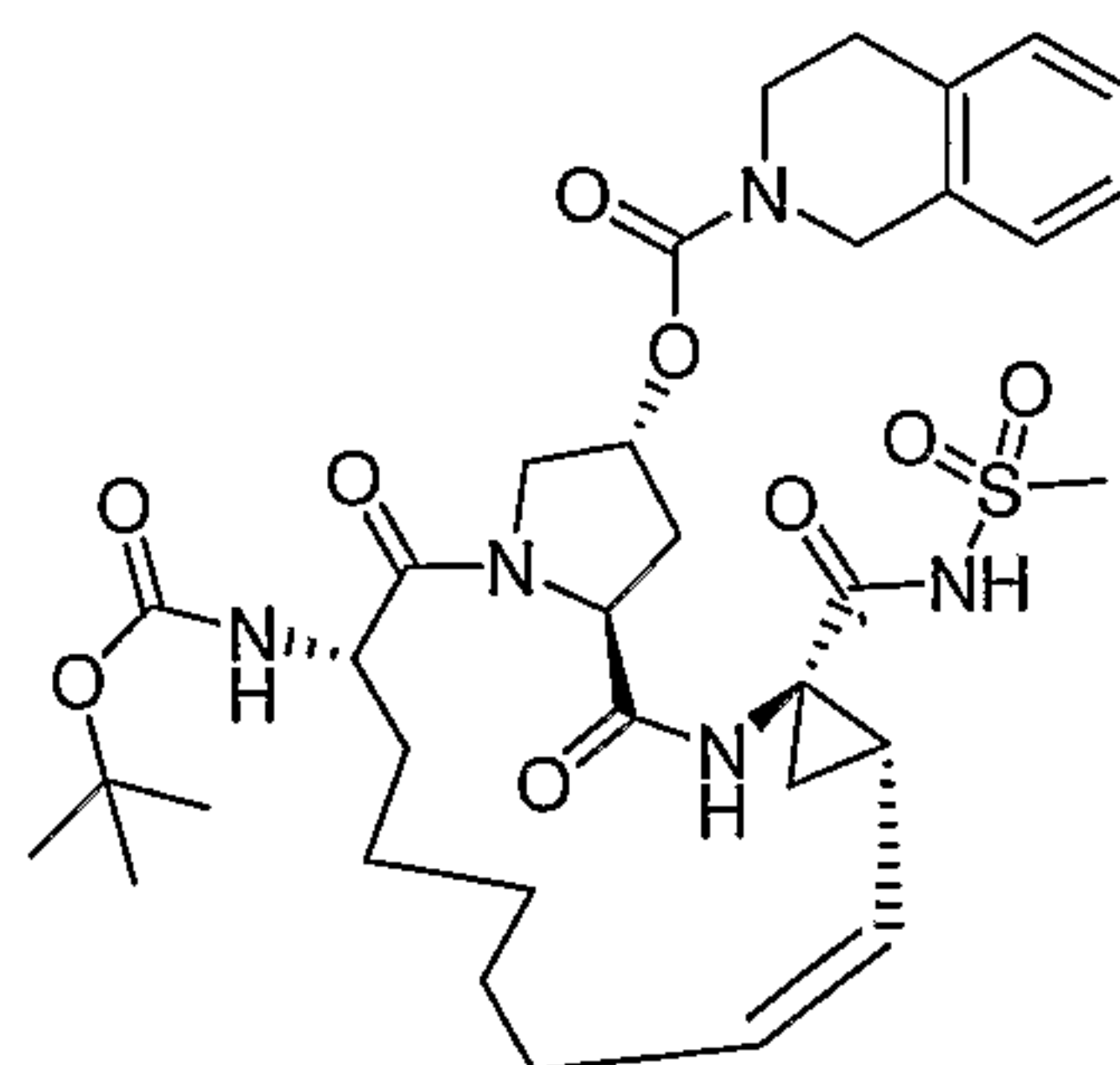
Compound AR00254906
