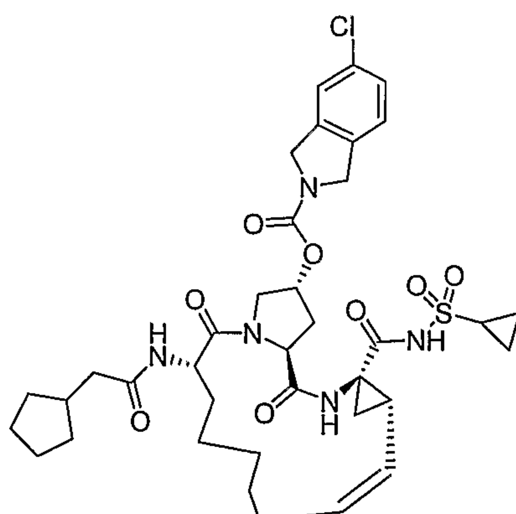
Compound AR00334226
