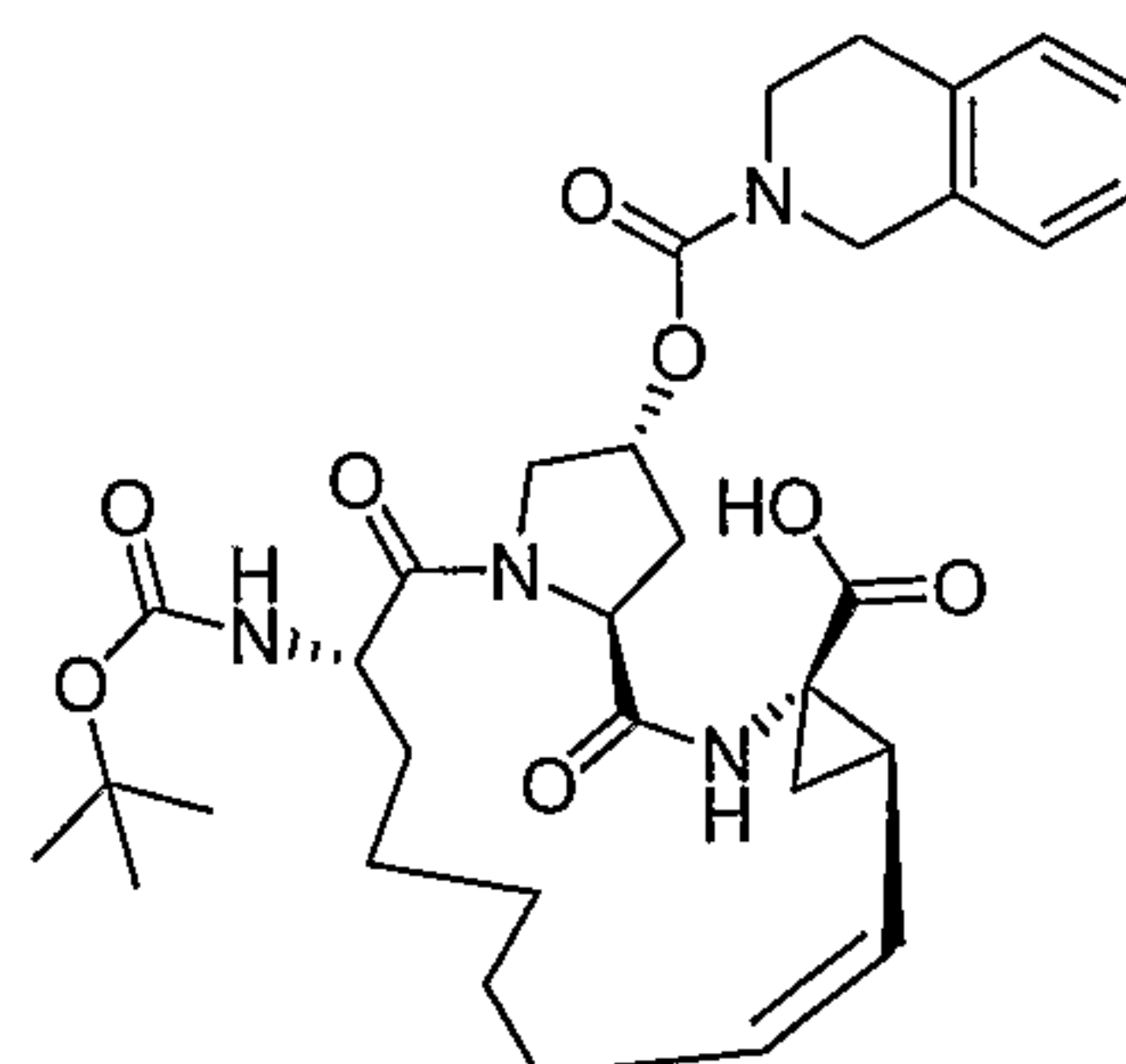
Compound AR00220122
