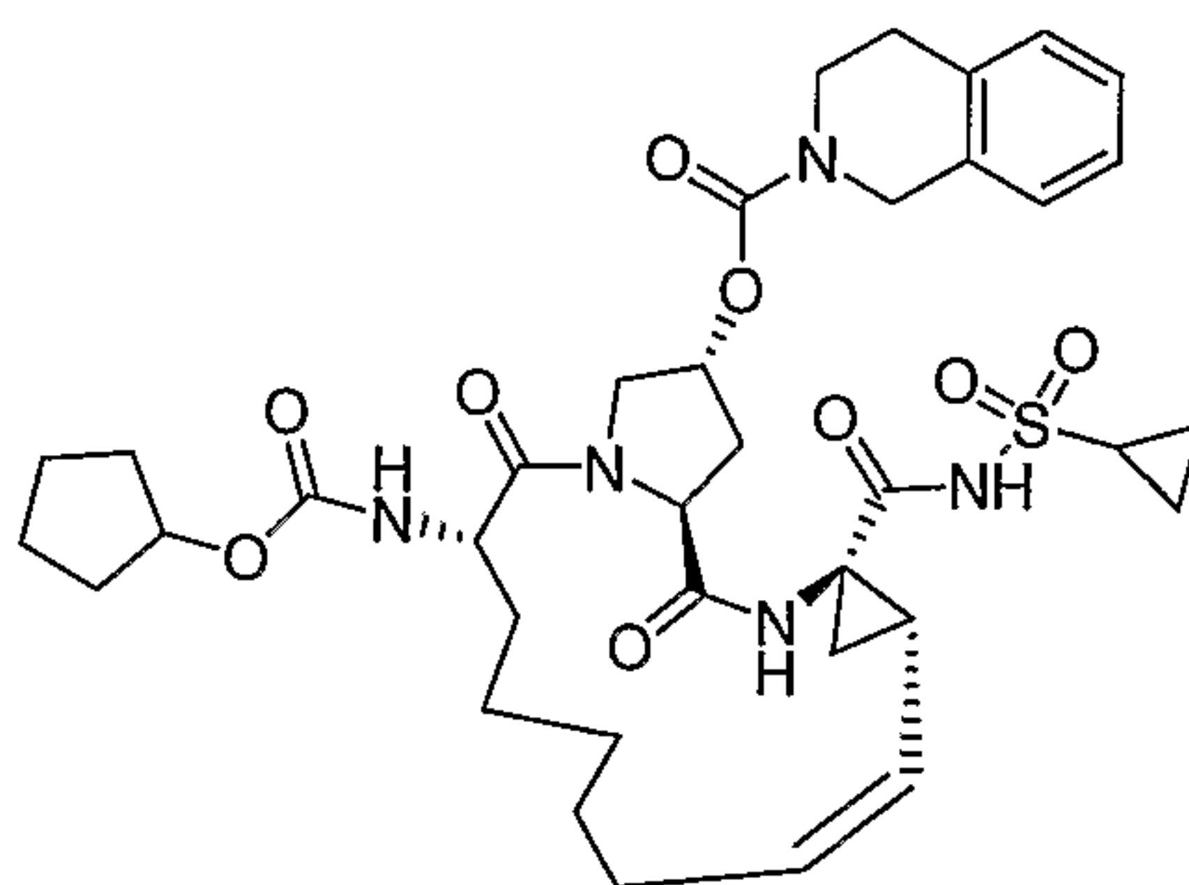
Compound AR00282131
