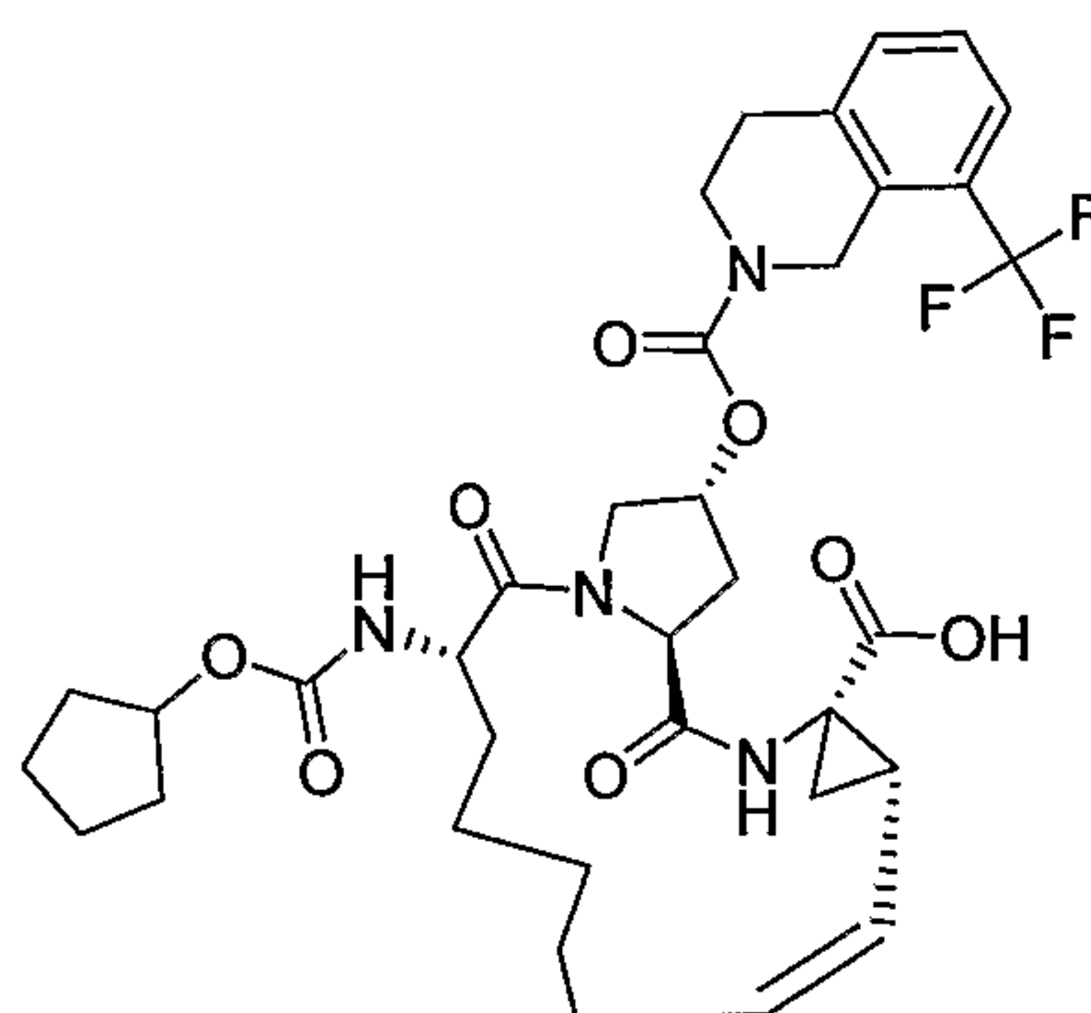
Compound AR00304075
