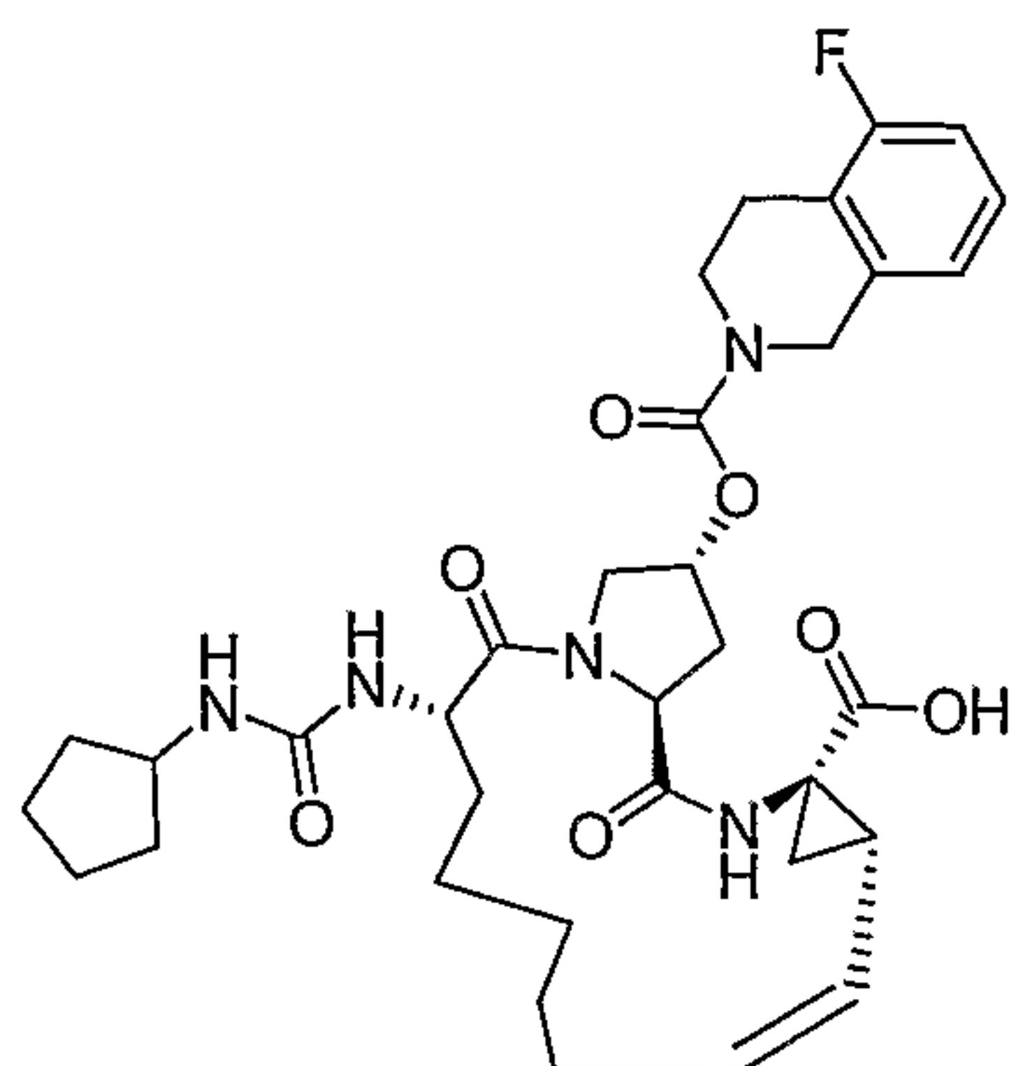
Compound AR00304077
