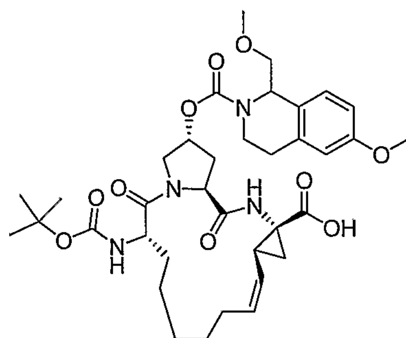
Compound AR00333842
