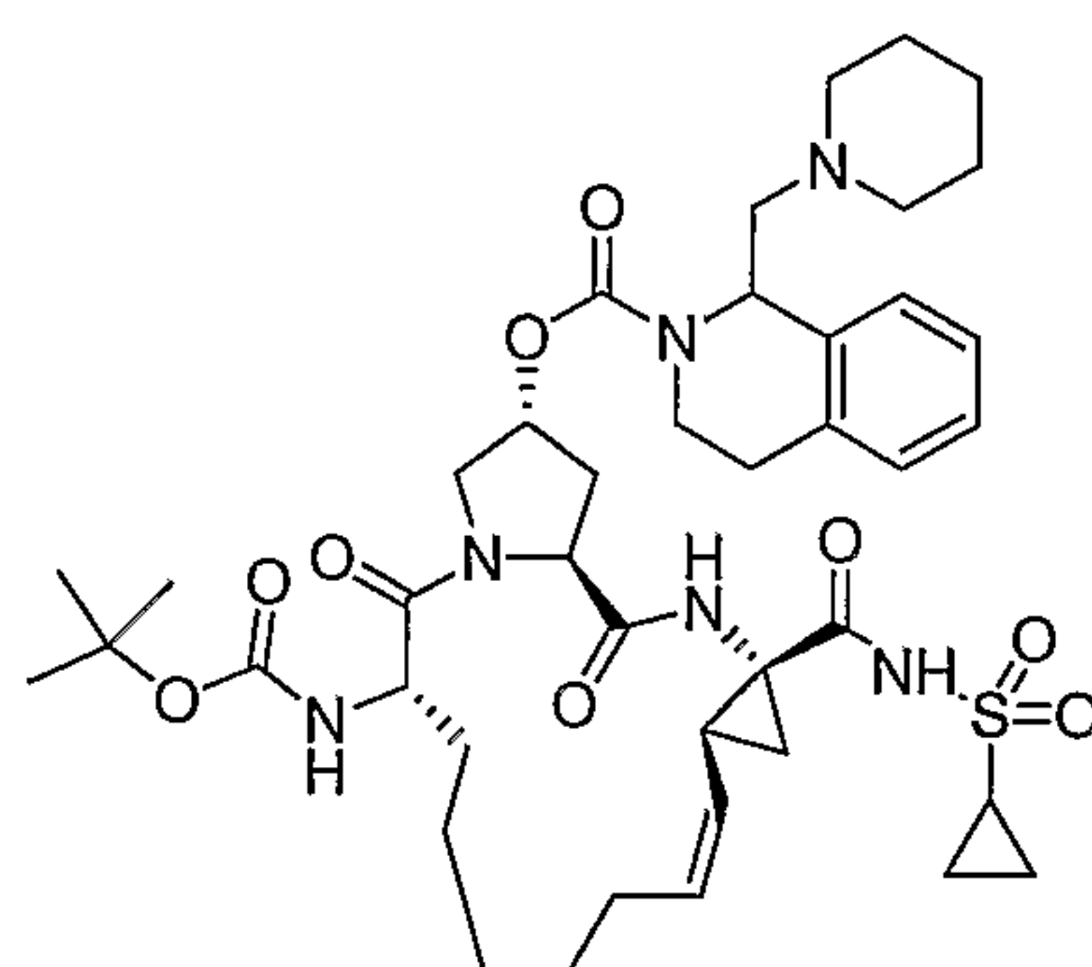
Compound AR00311815
