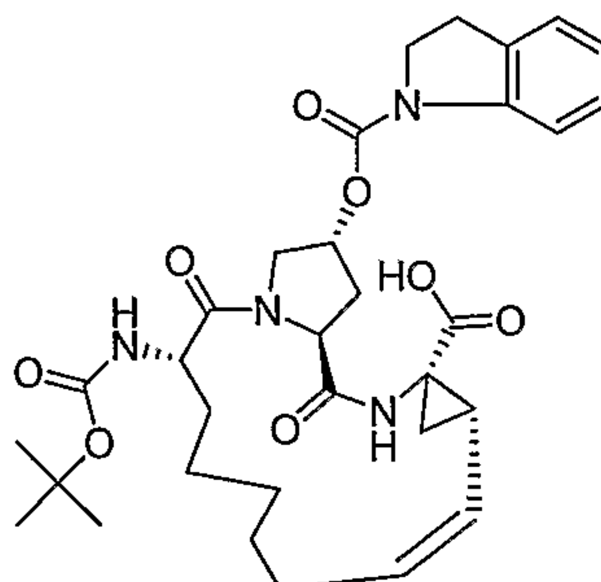
Compound AR00291875
