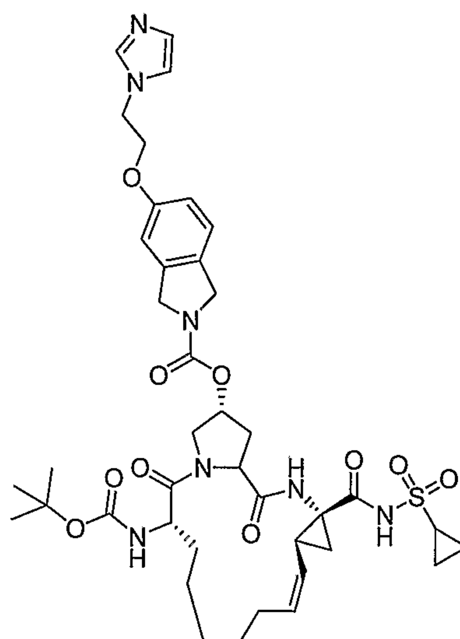
Compound AR00345096
