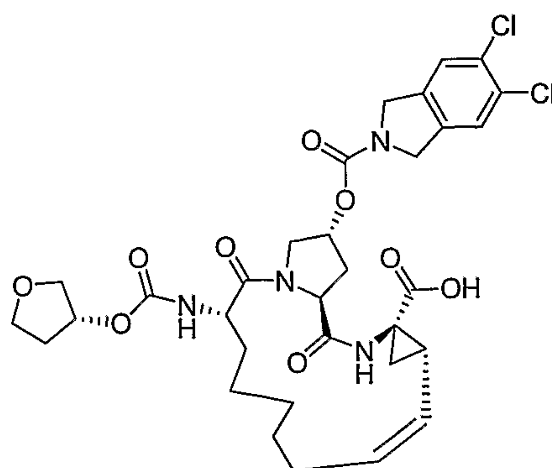
Compound AR00320445
