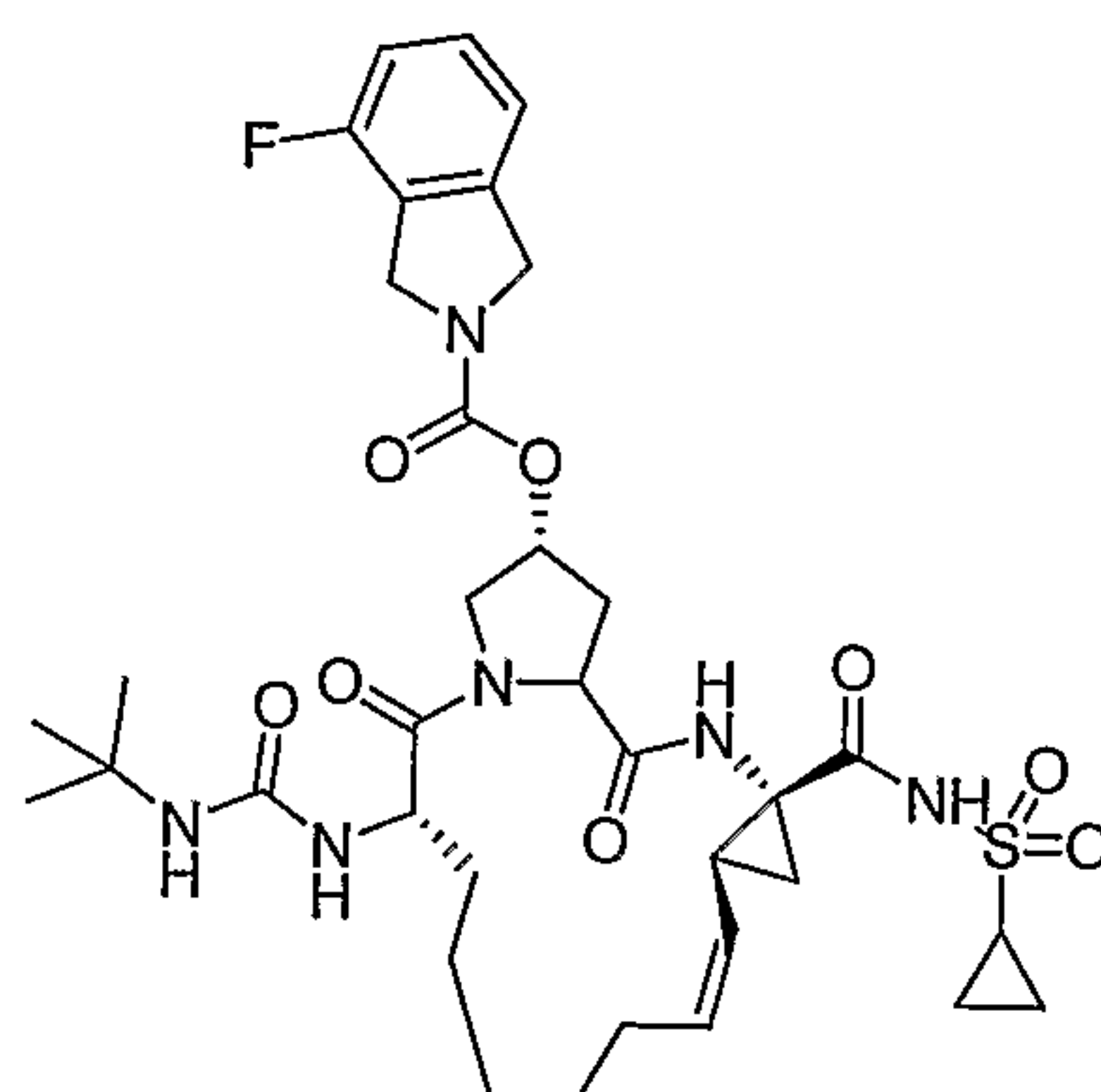
Compound AR00338066
