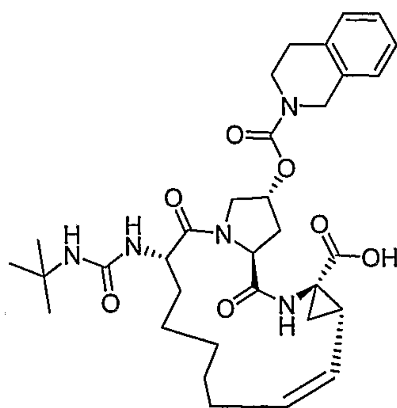
Compound AR00294377
