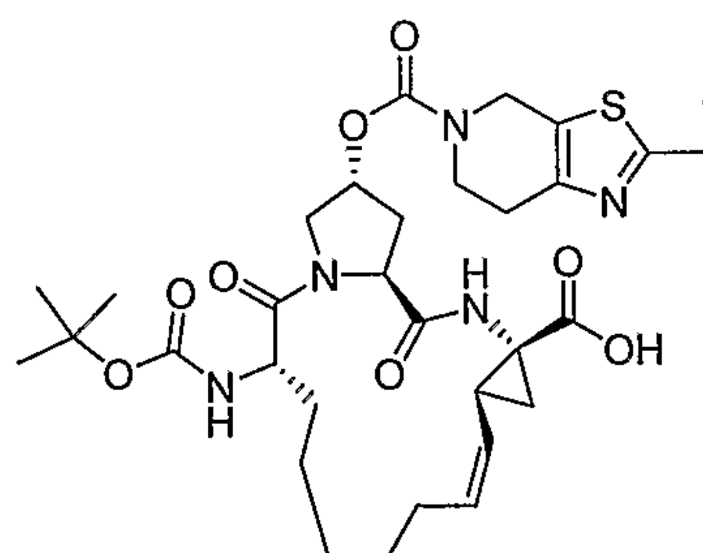
Compound AR00304158
