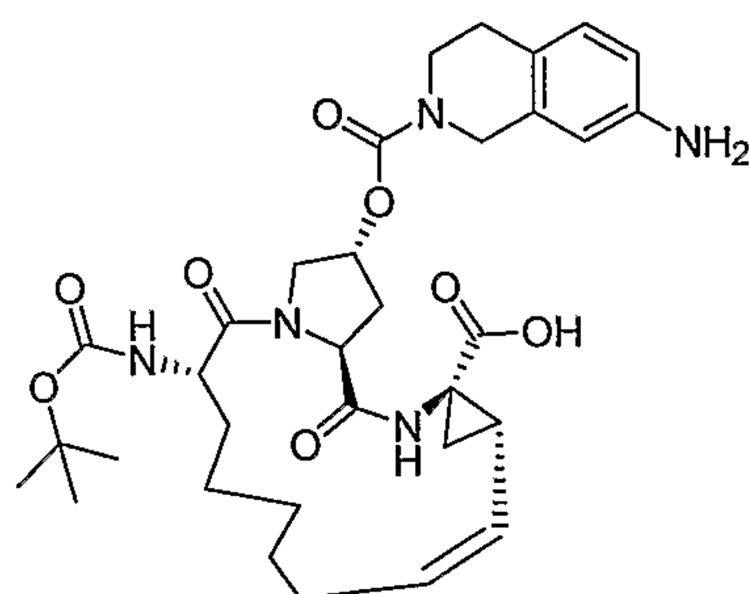
Compound AR00301749
