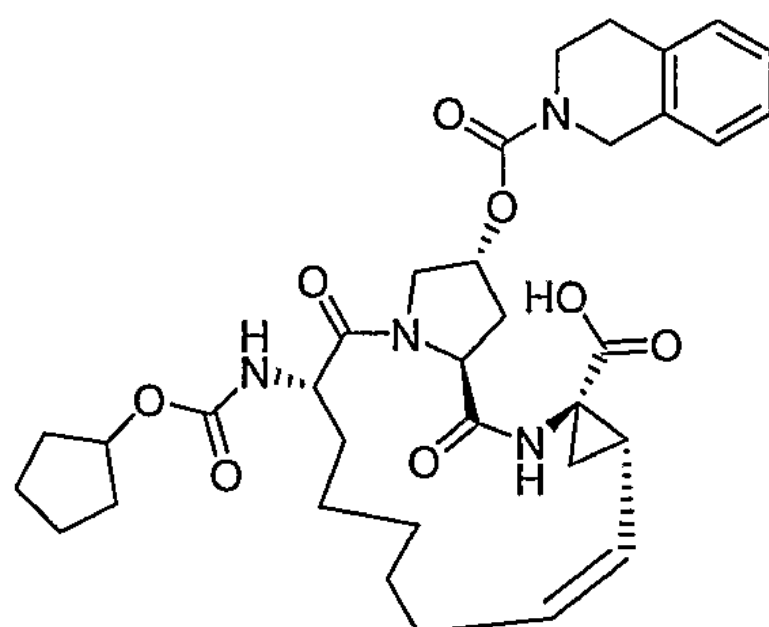
Compound AR00247310
