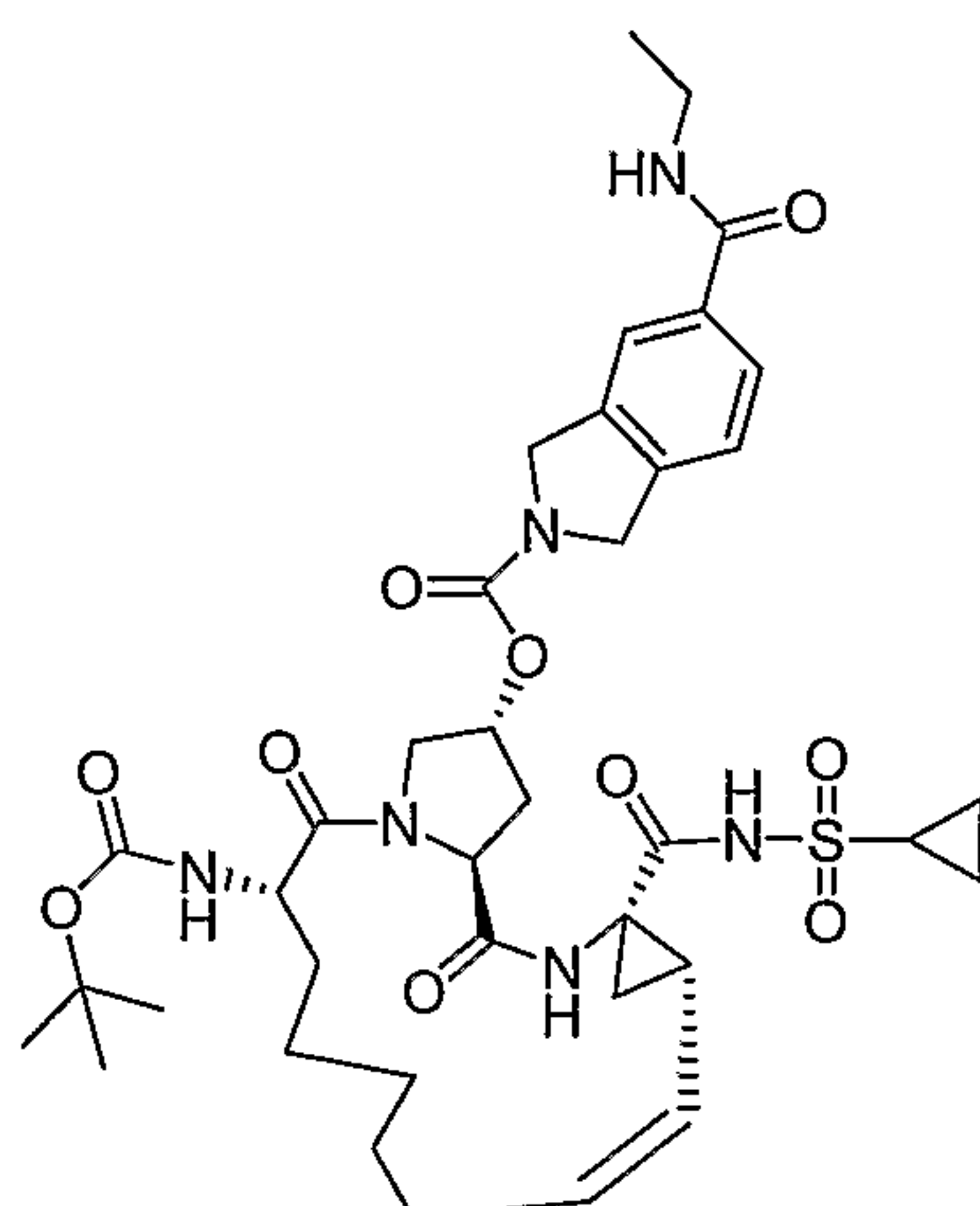
Compound AR00365252
