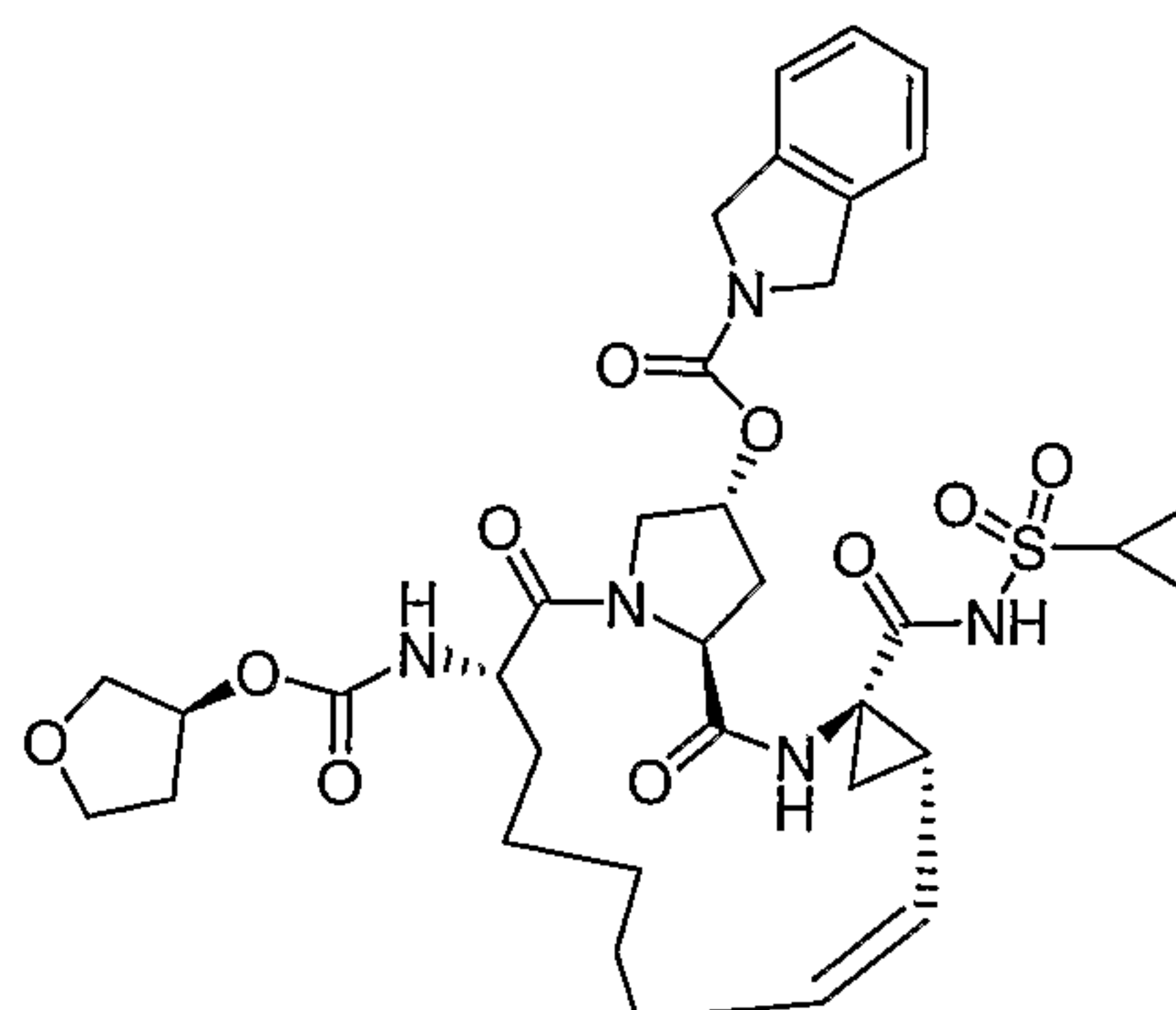
Compound AR00320080
