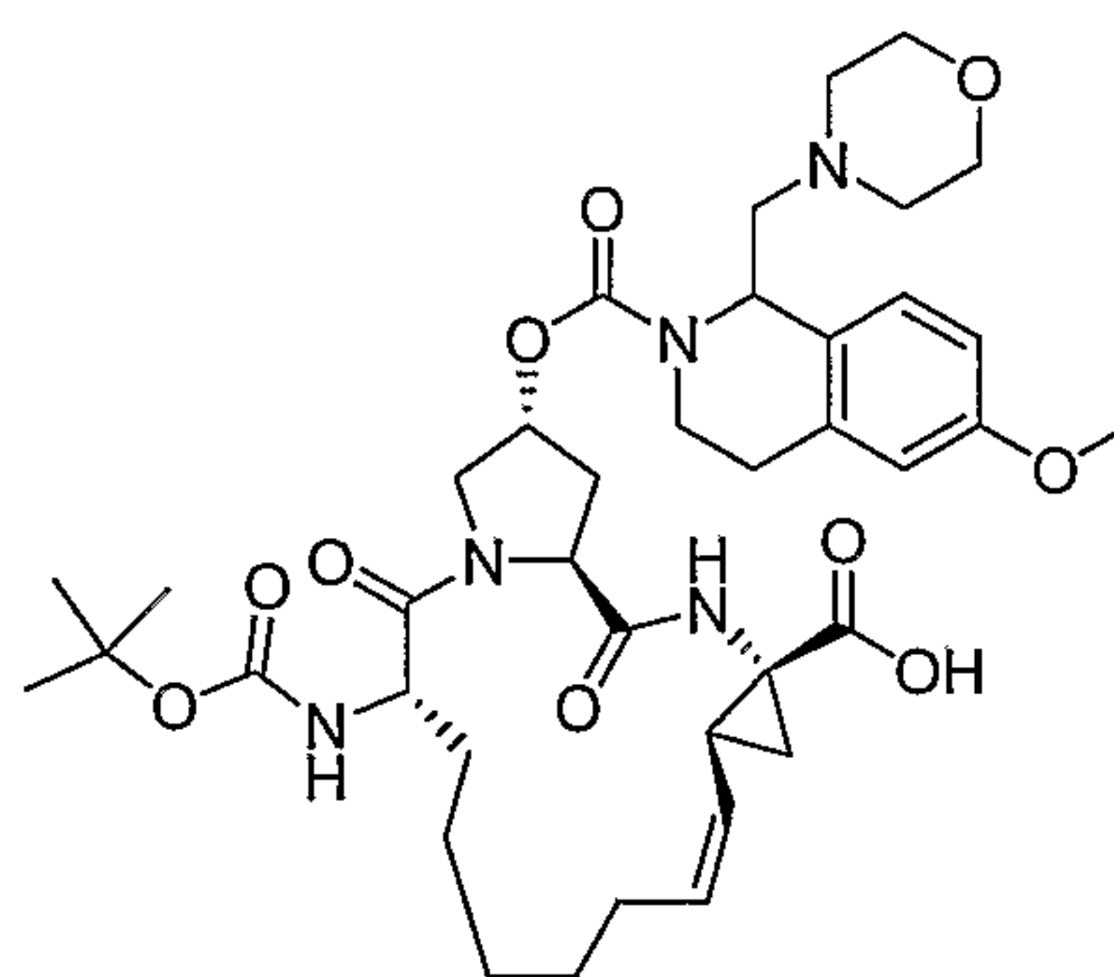
Compound AR00333276
