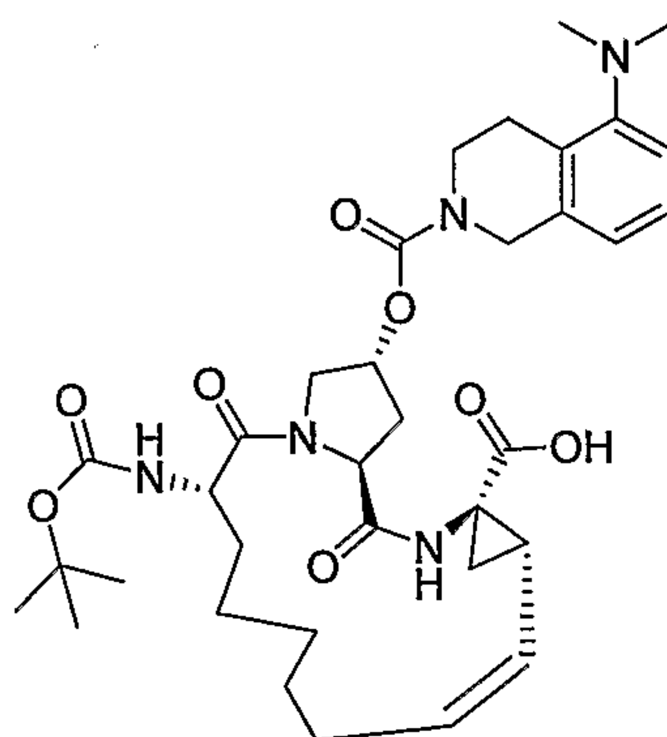
Compound AR00315997
