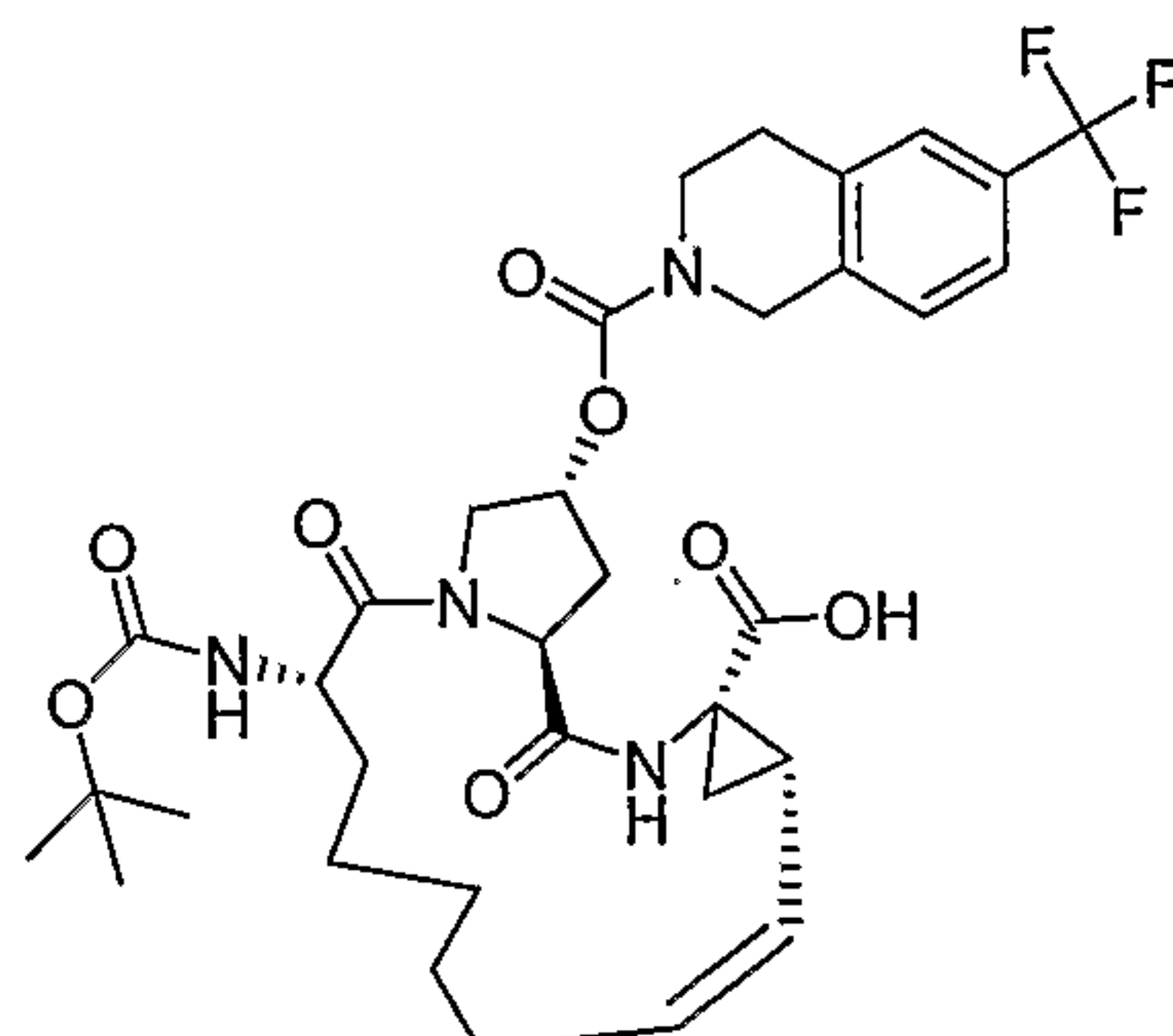
Compound AR00294383
