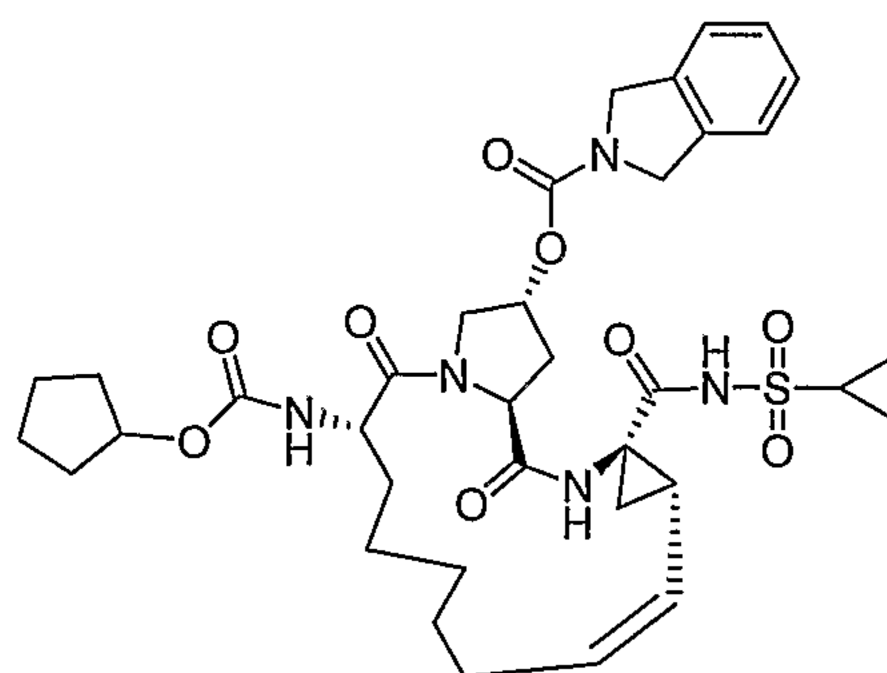
Compound AR00333831
