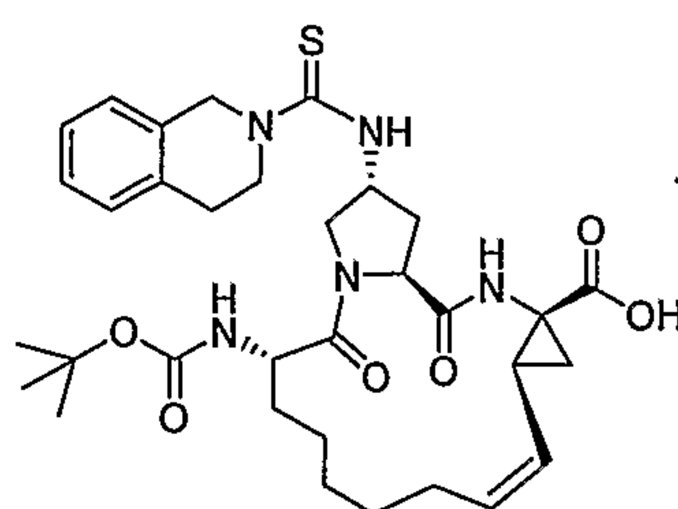
Compound AR00304010
