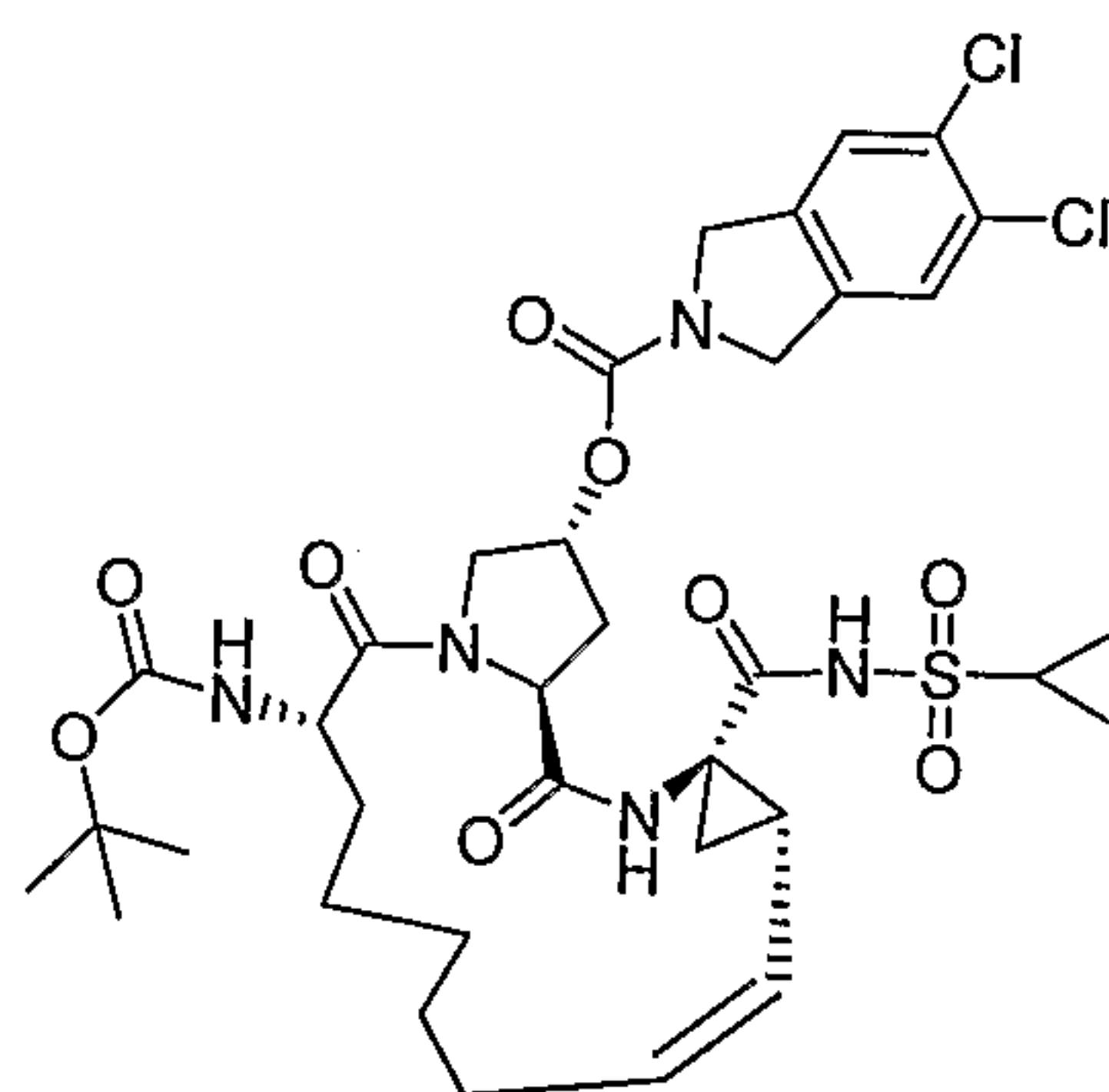
Compound AR00320121
