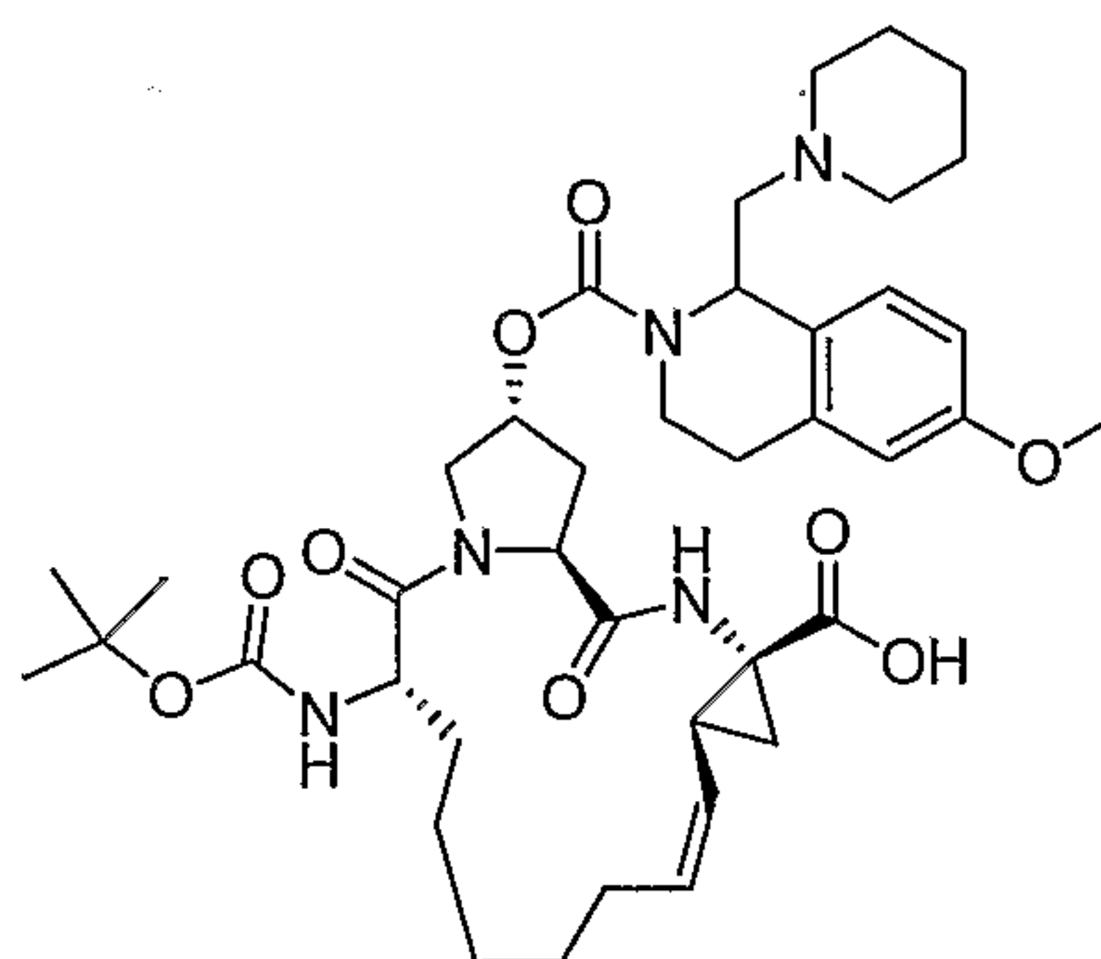
Compound AR00333248
