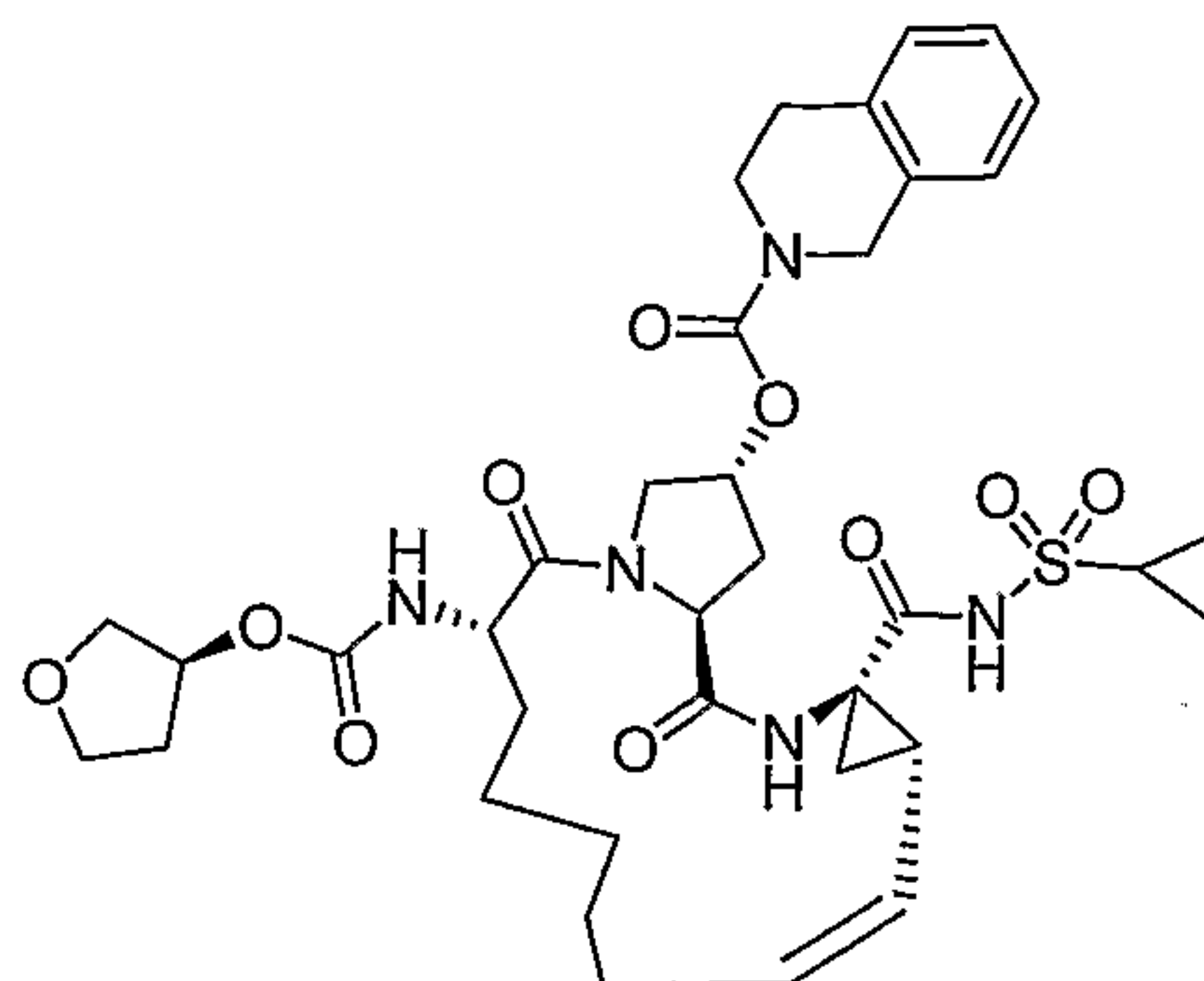
Compound AR00304162
