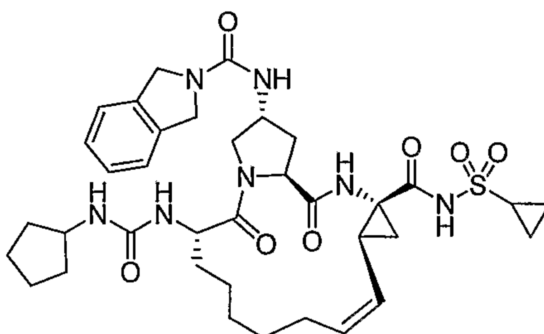
Compound AR00304014
