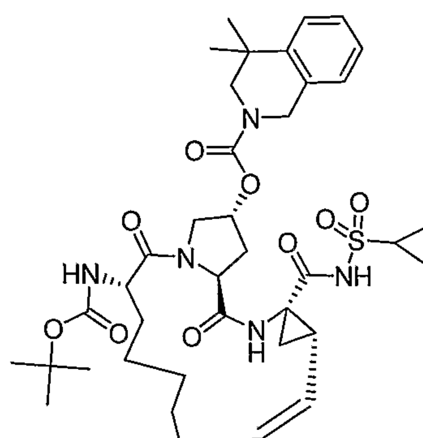
Compound AR00312025
