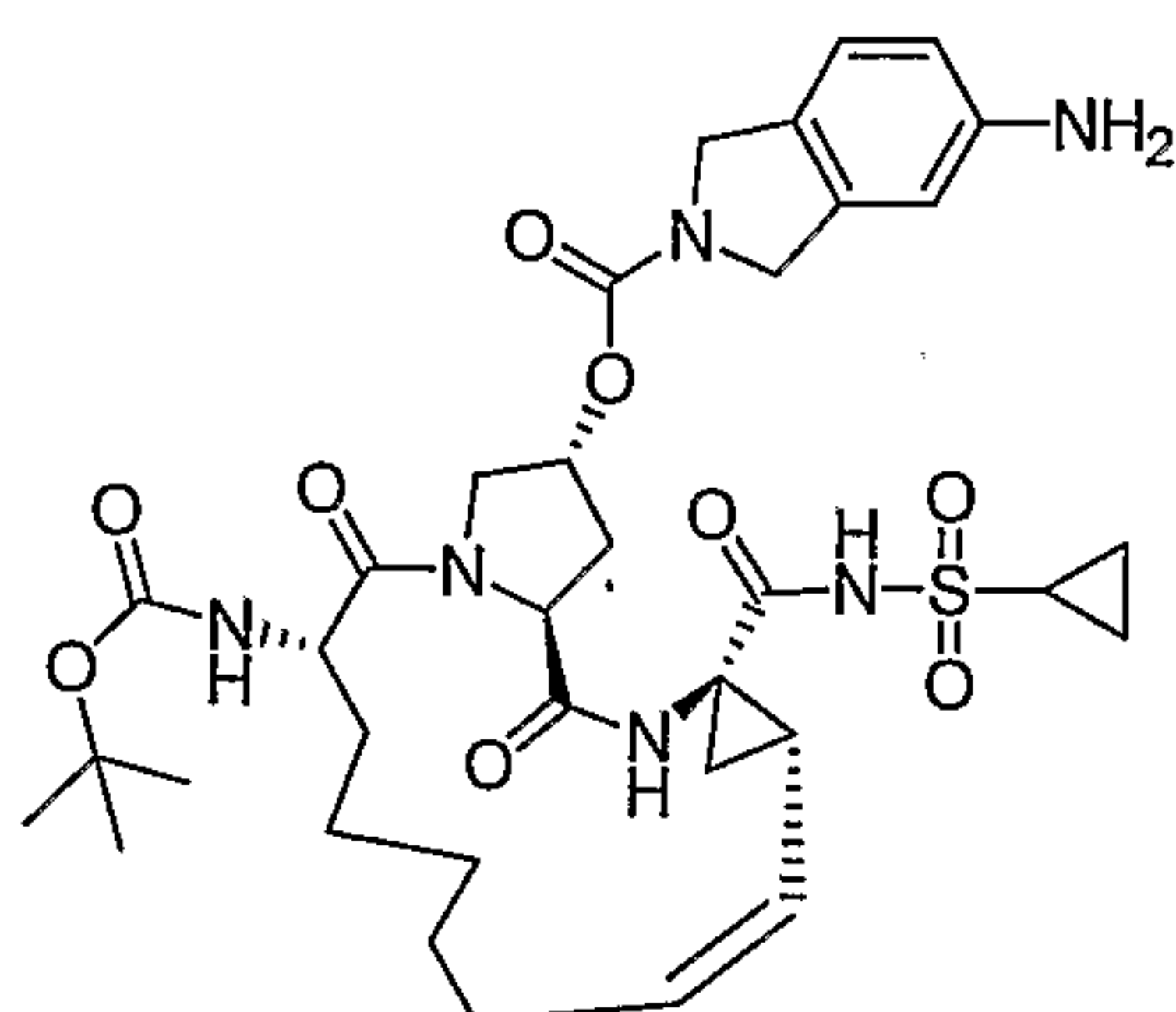
Compound AR00334286
