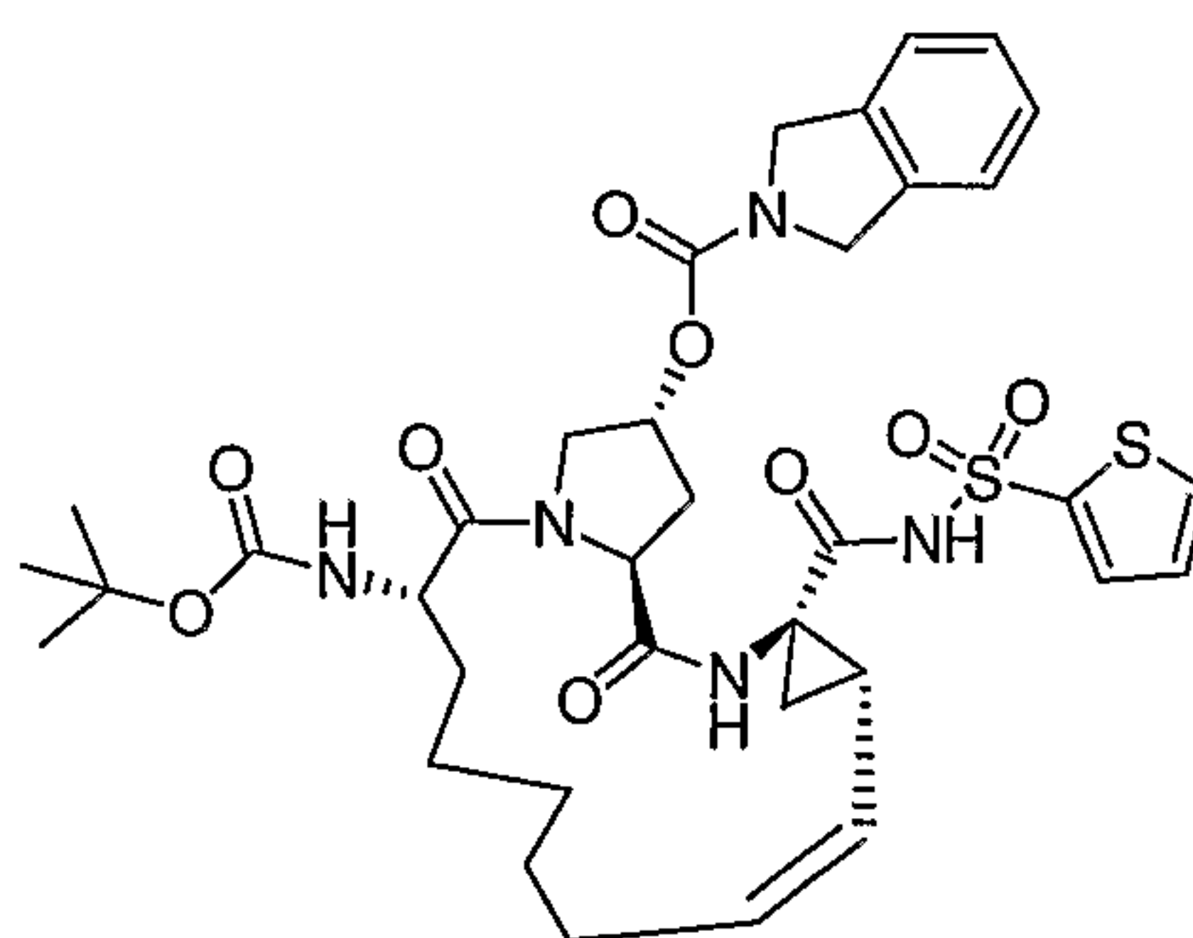
Compound AR00365427
