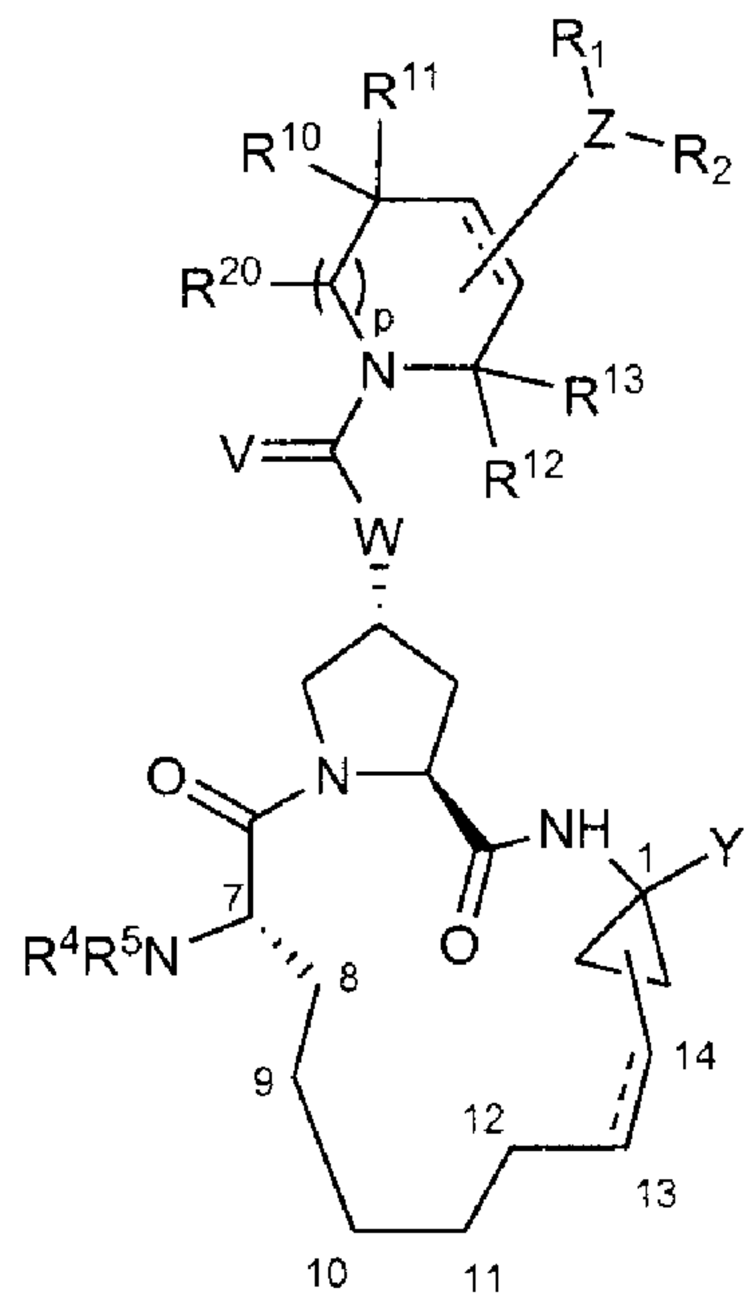
IX
