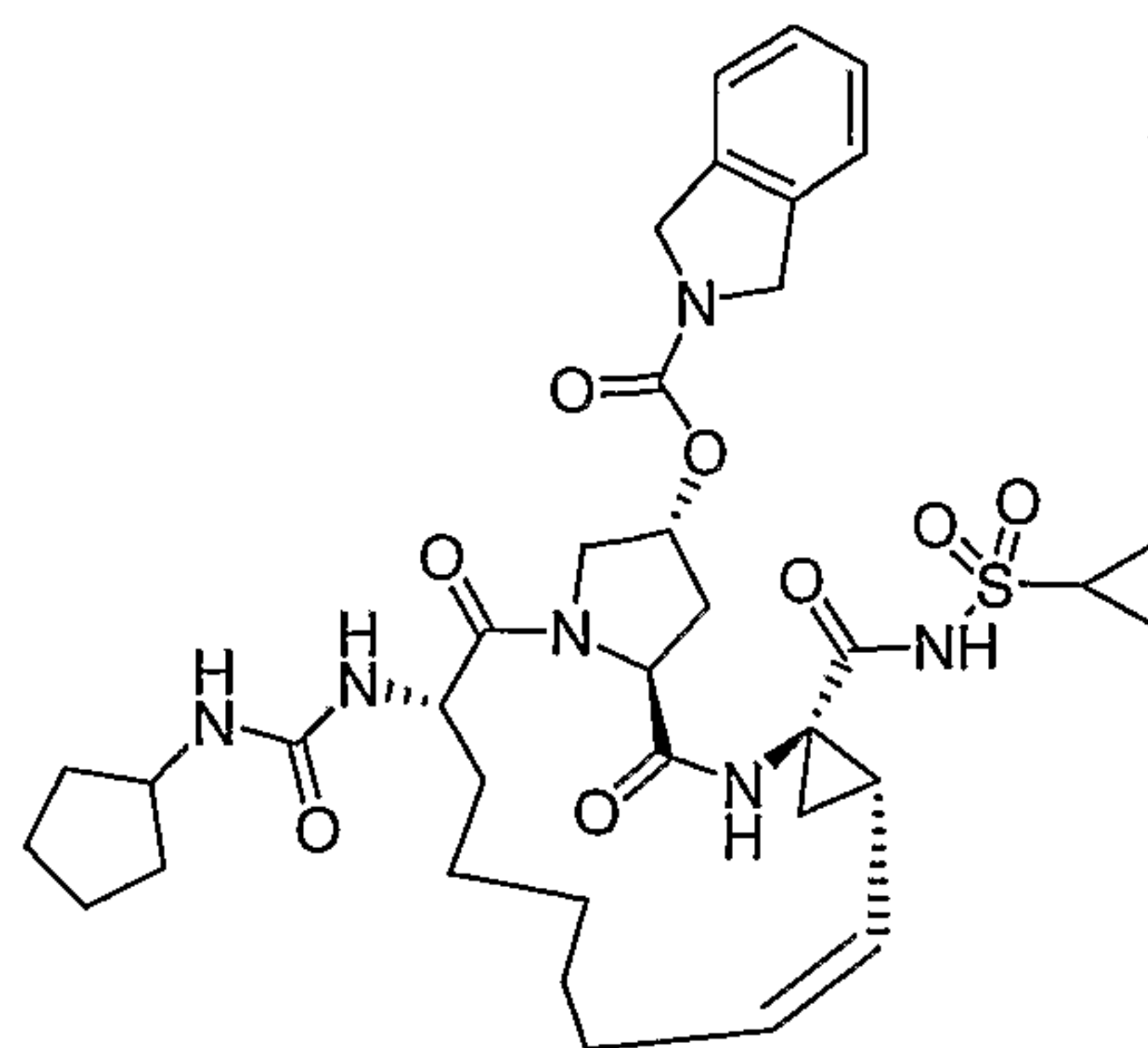
Compound AR00304082
