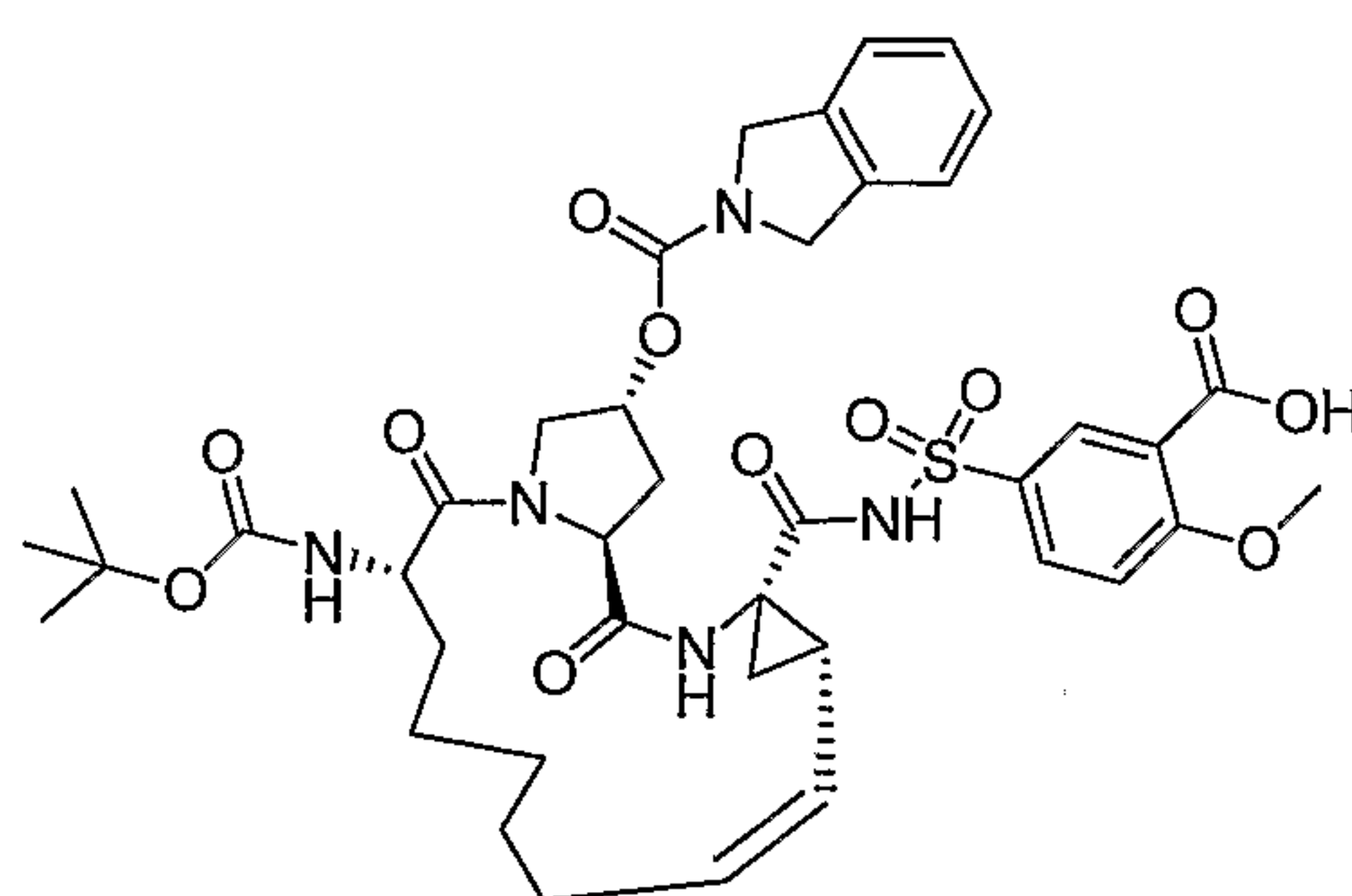
Compound AR00365425
