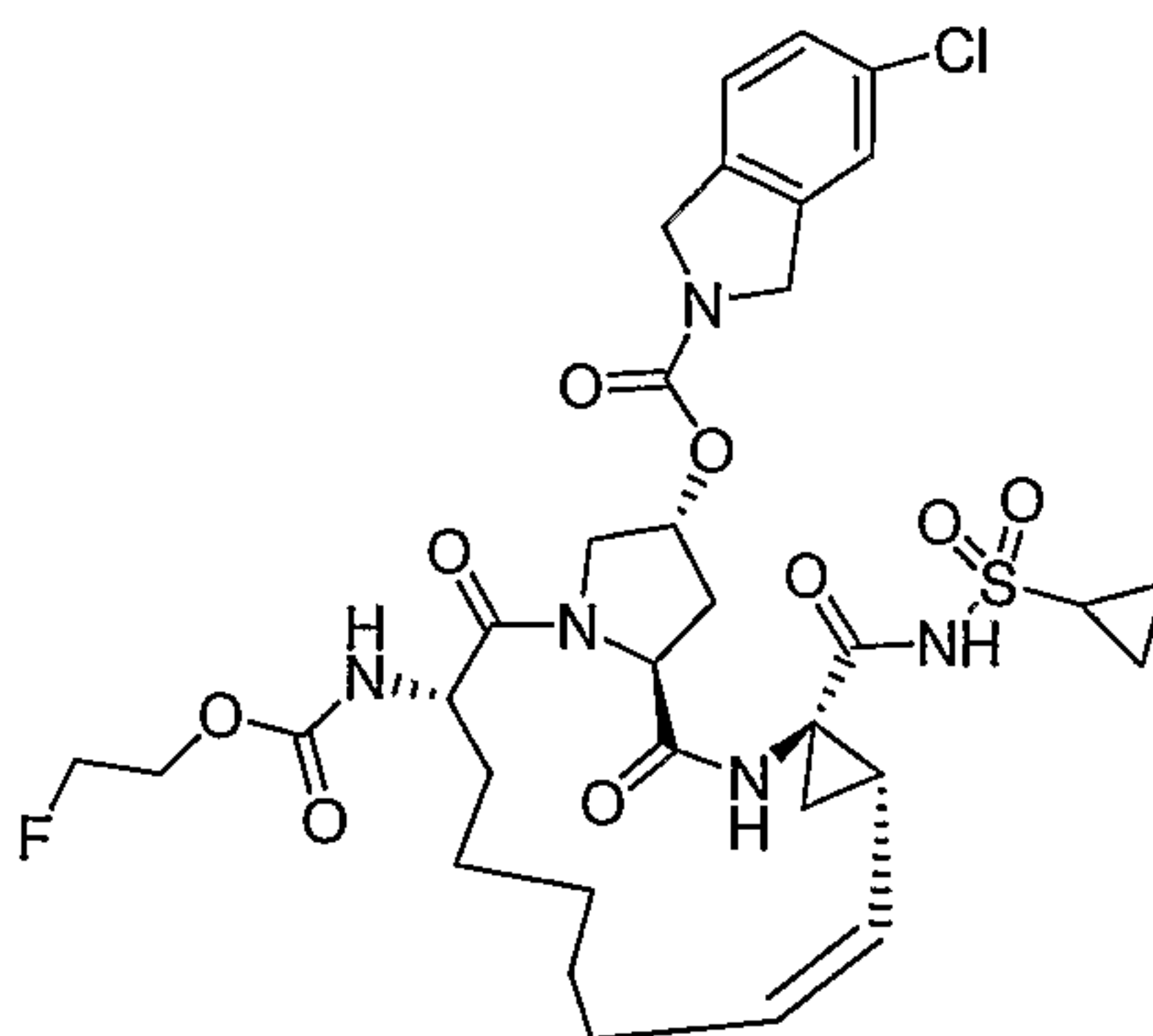
Compound AR00334222
