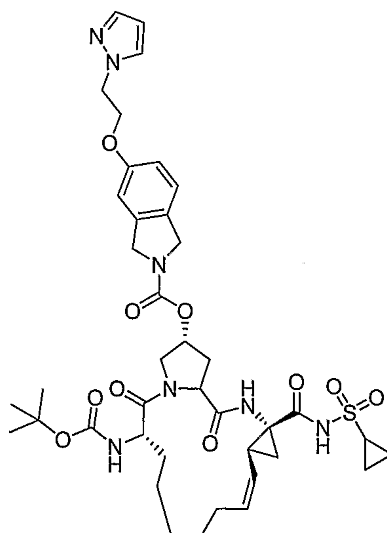
Compound AR00364924
