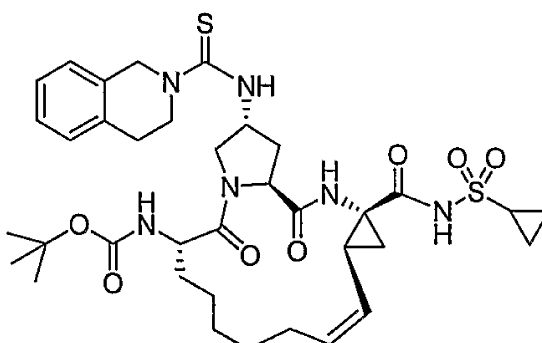
Compound AR00304012
