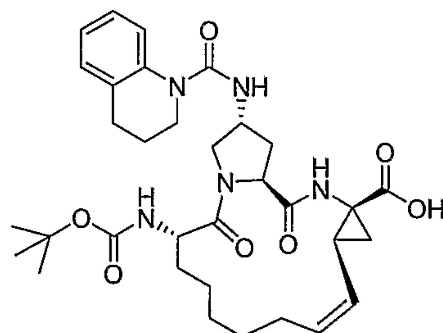
Compound AR00304160
