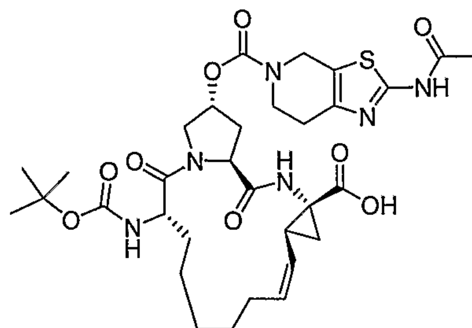
Compound AR00314685
