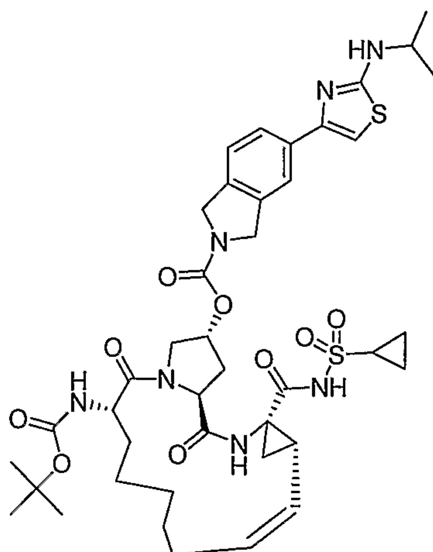
Compound AR00365019
