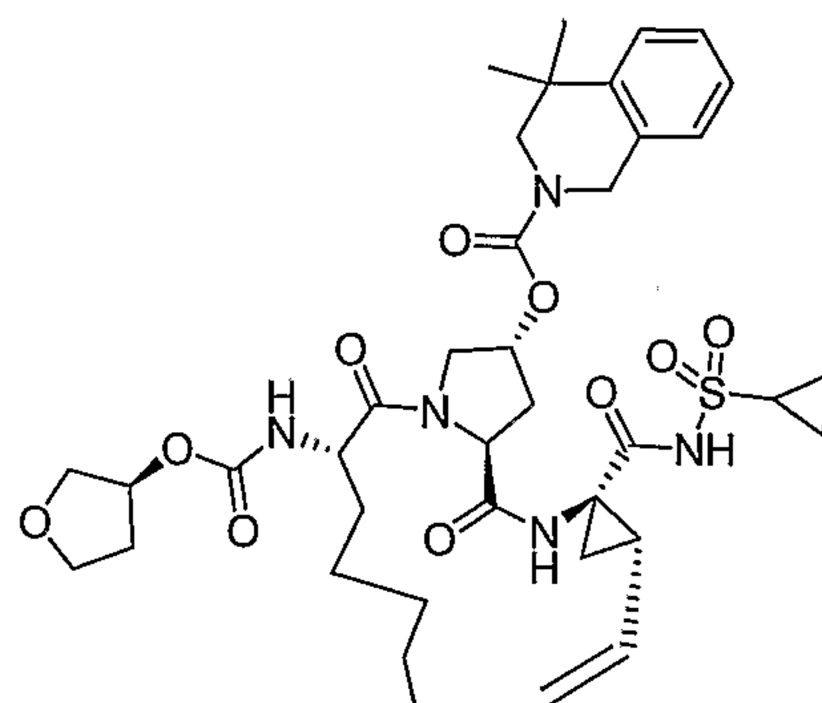
Compound AR00314654
