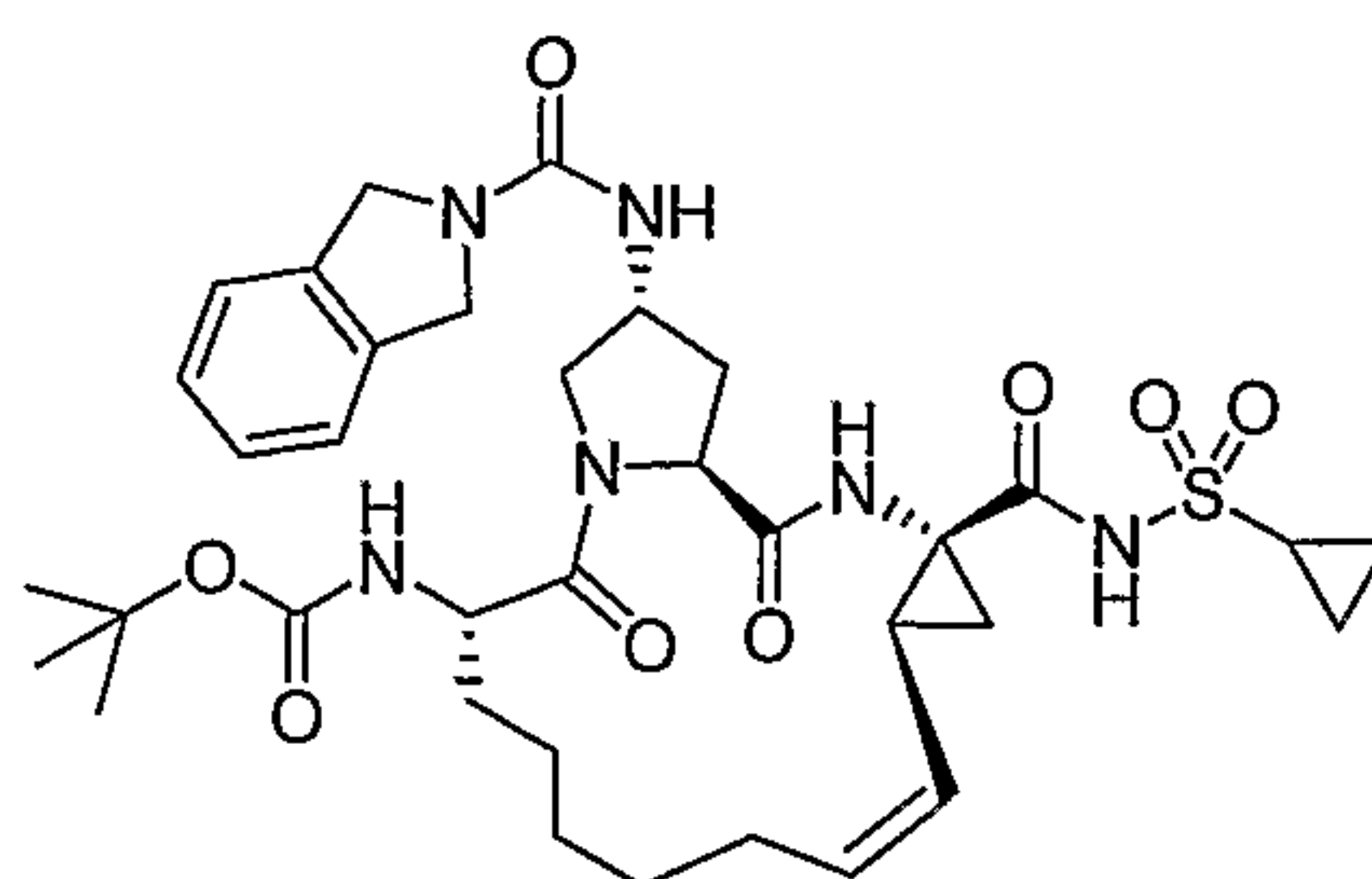
Compound AR00304008
