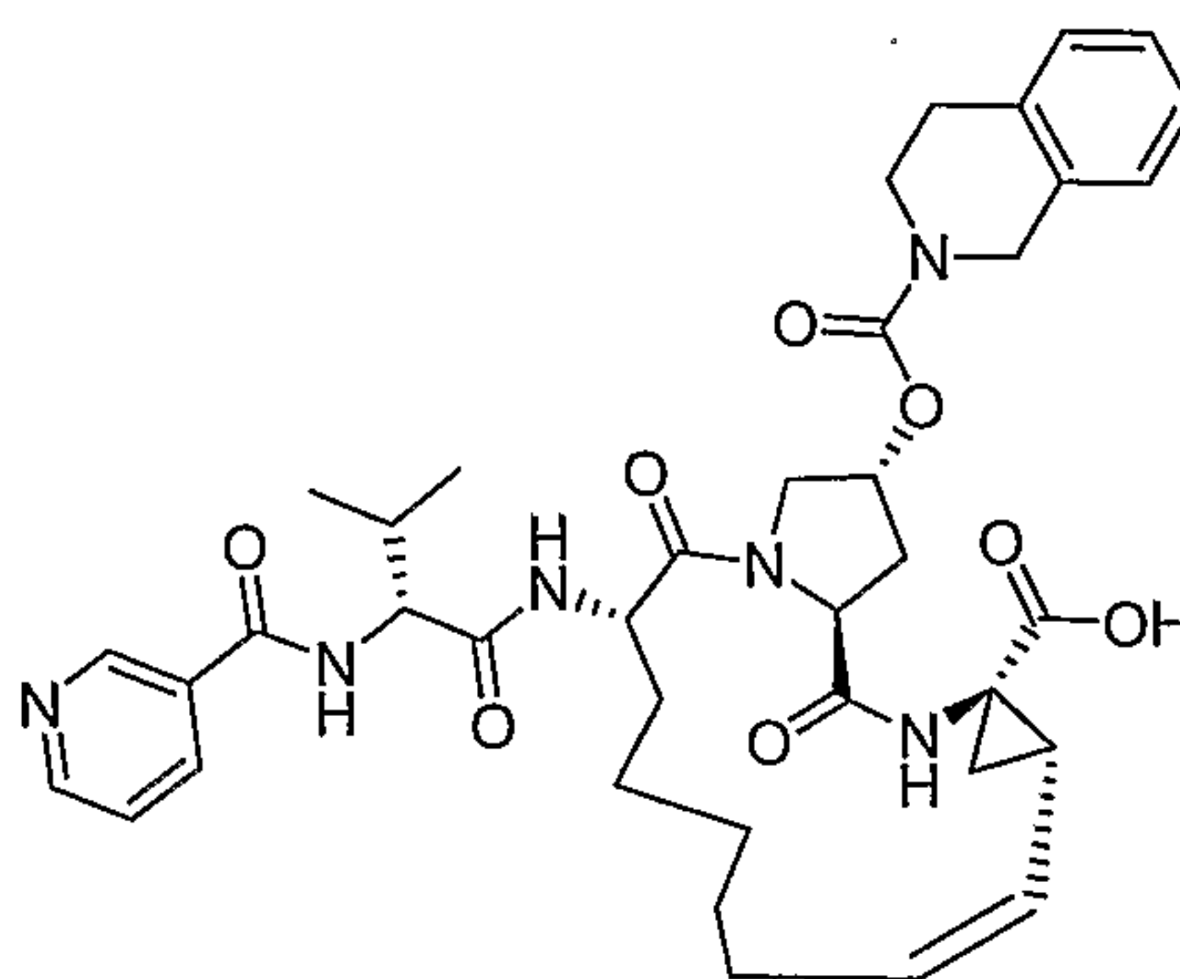
Compound AR00304073
