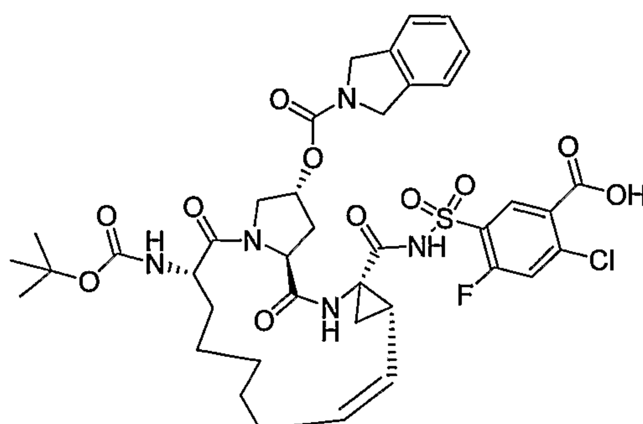
Compound AR00365426
