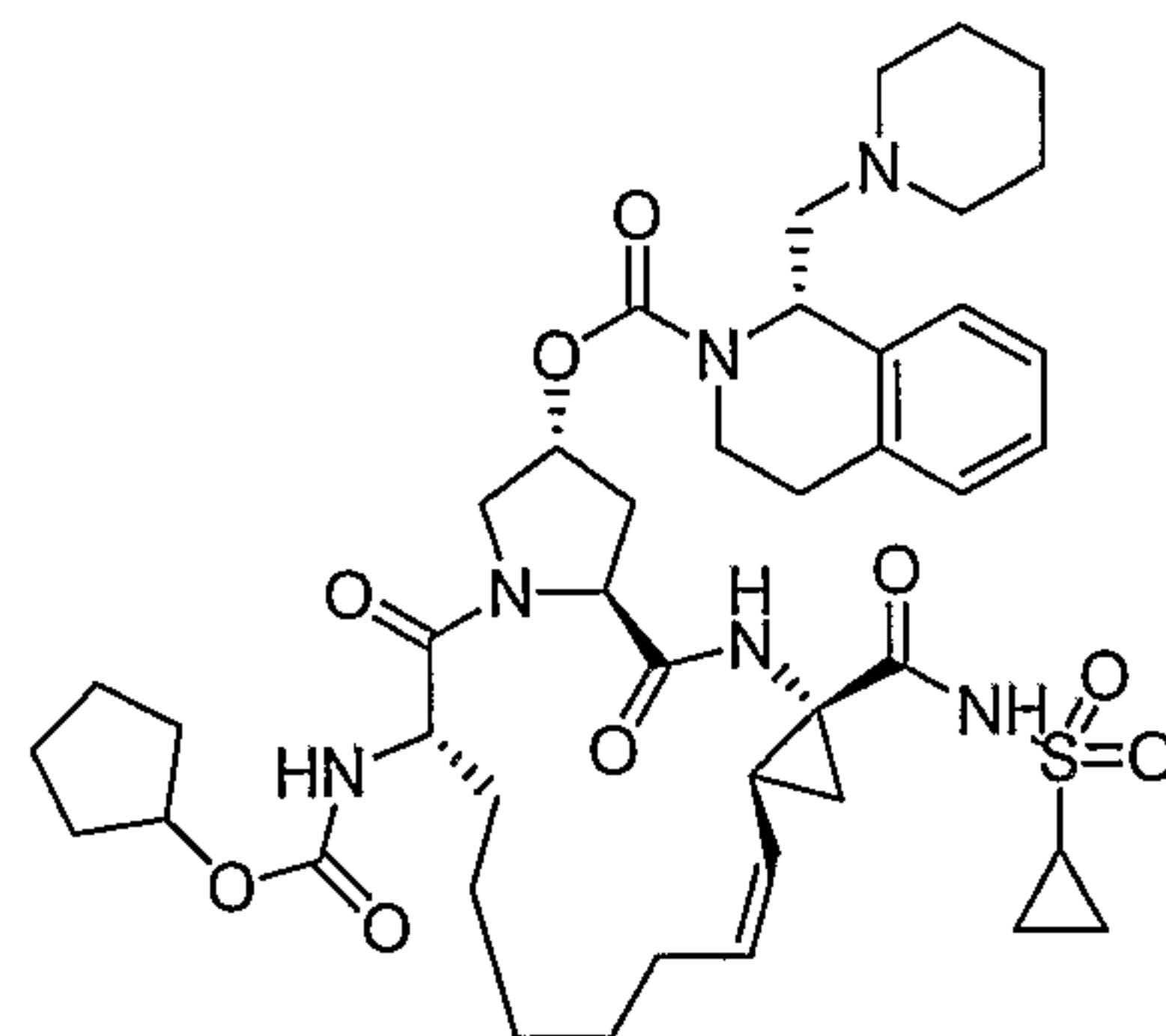
Compound AR00320557
