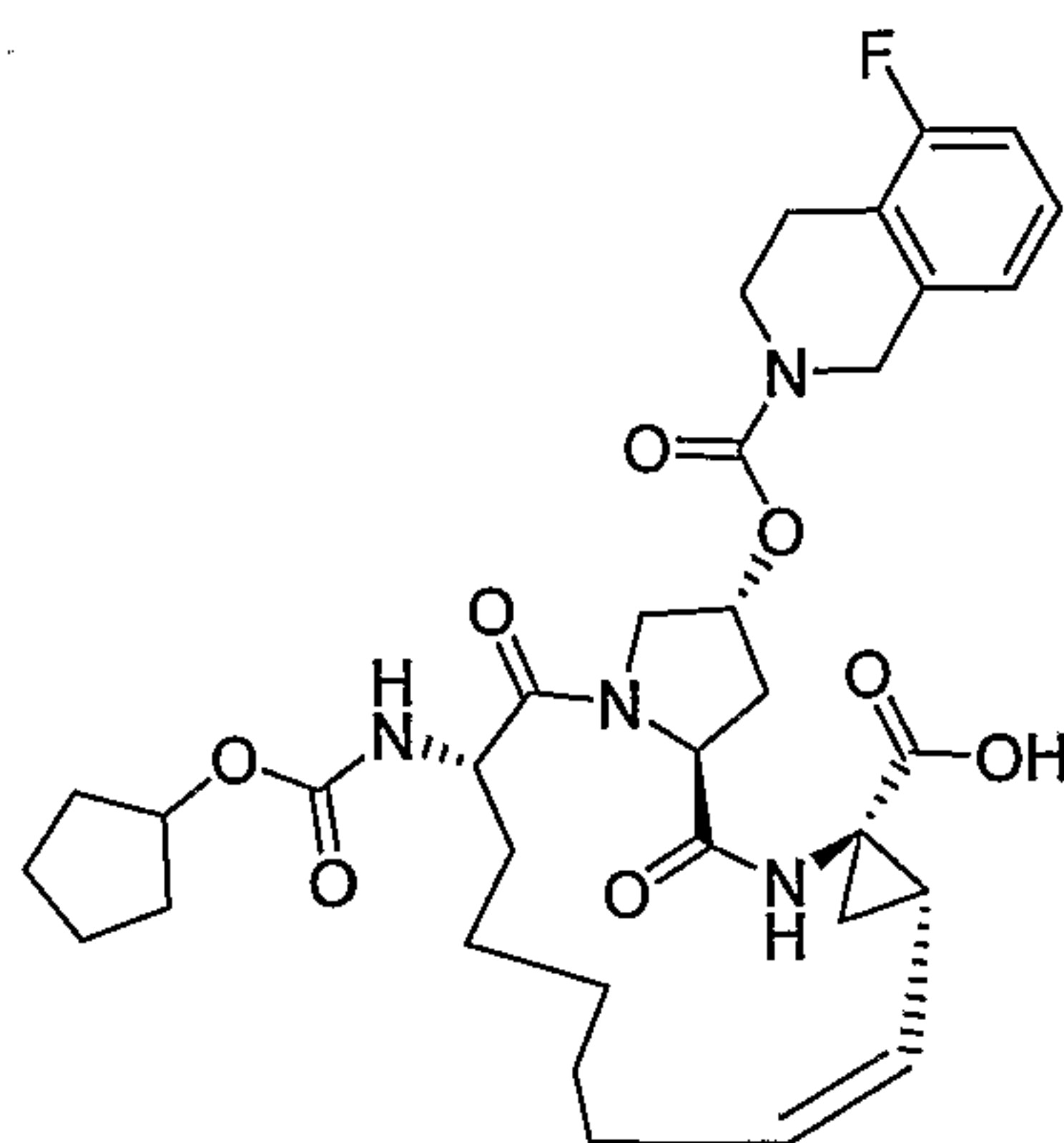
Compound AR00304074
