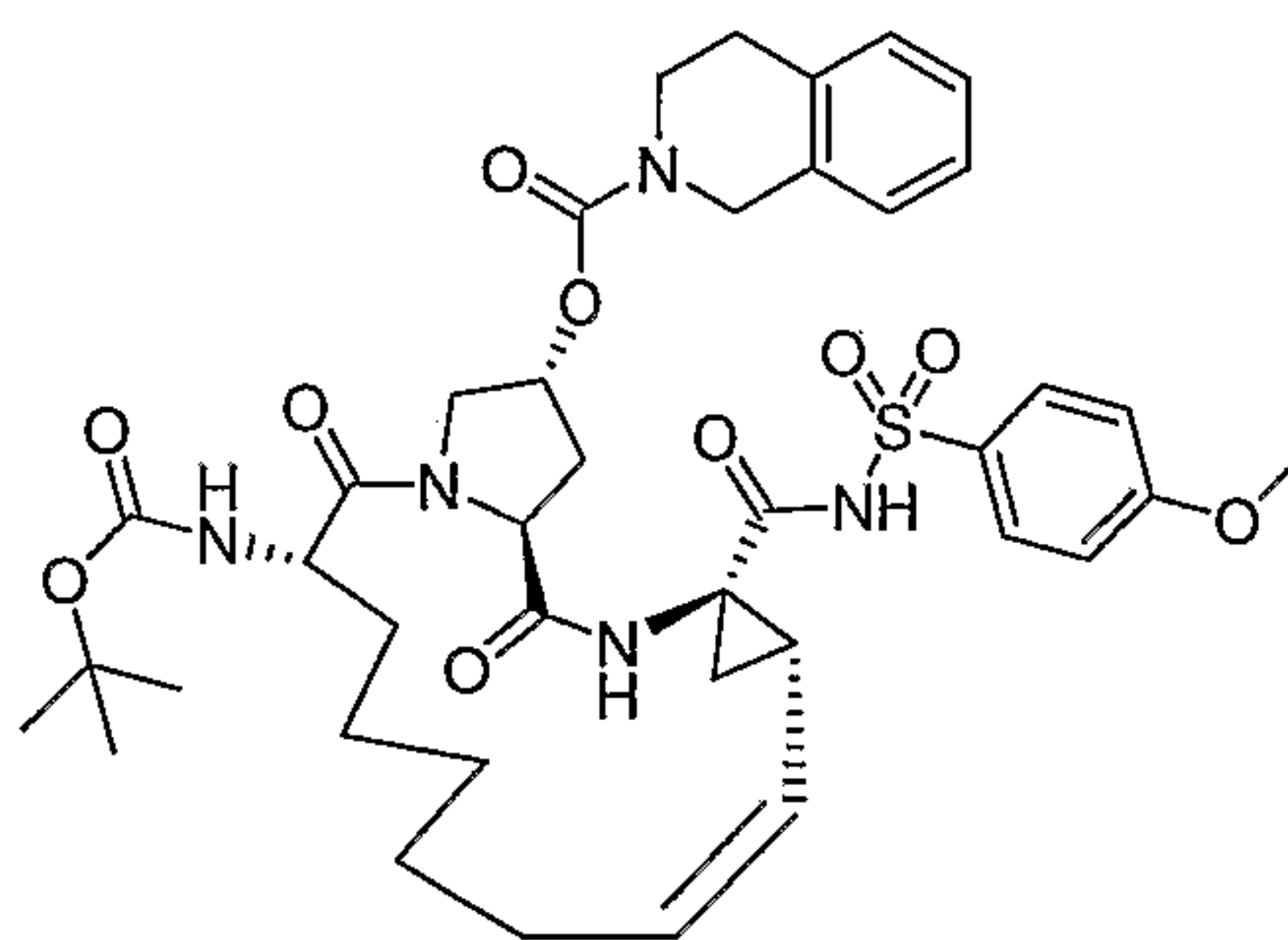
Compound AR00320548
