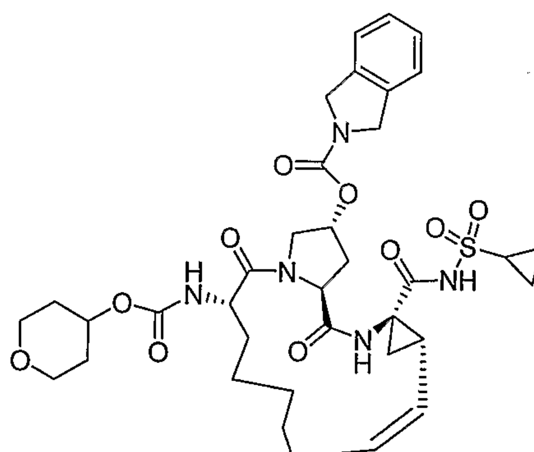
Compound AR00320081
