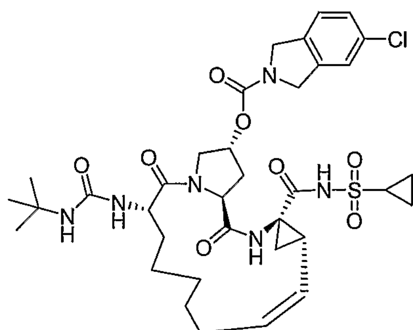
Compound AR00320446
