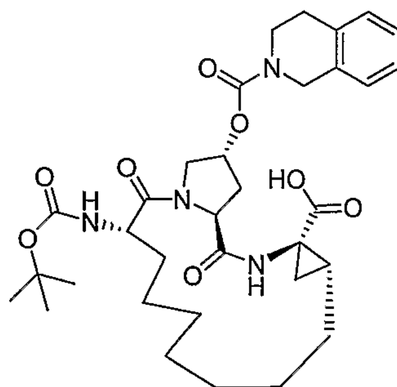
Compound AR00312023
