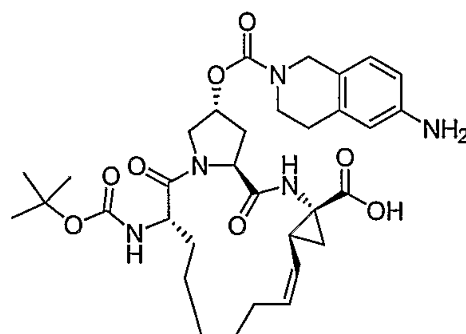
Compound AR00314578
