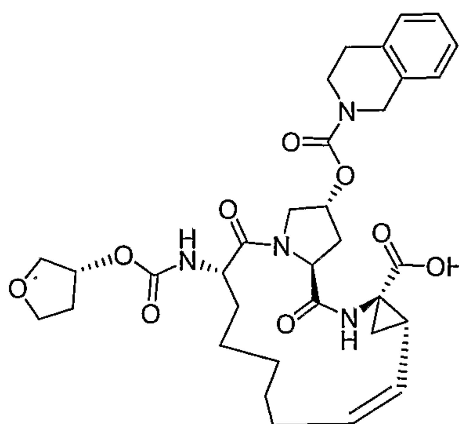
Compound AR00304127
