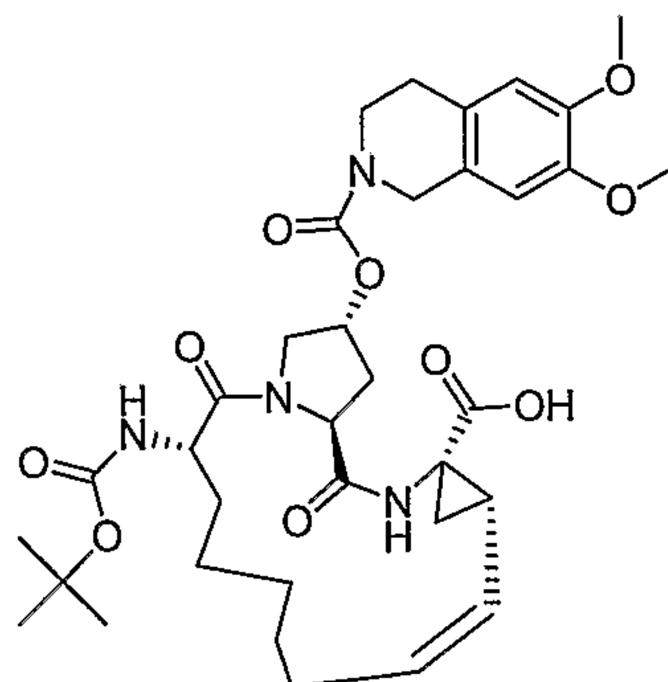
Compound AR00226824
