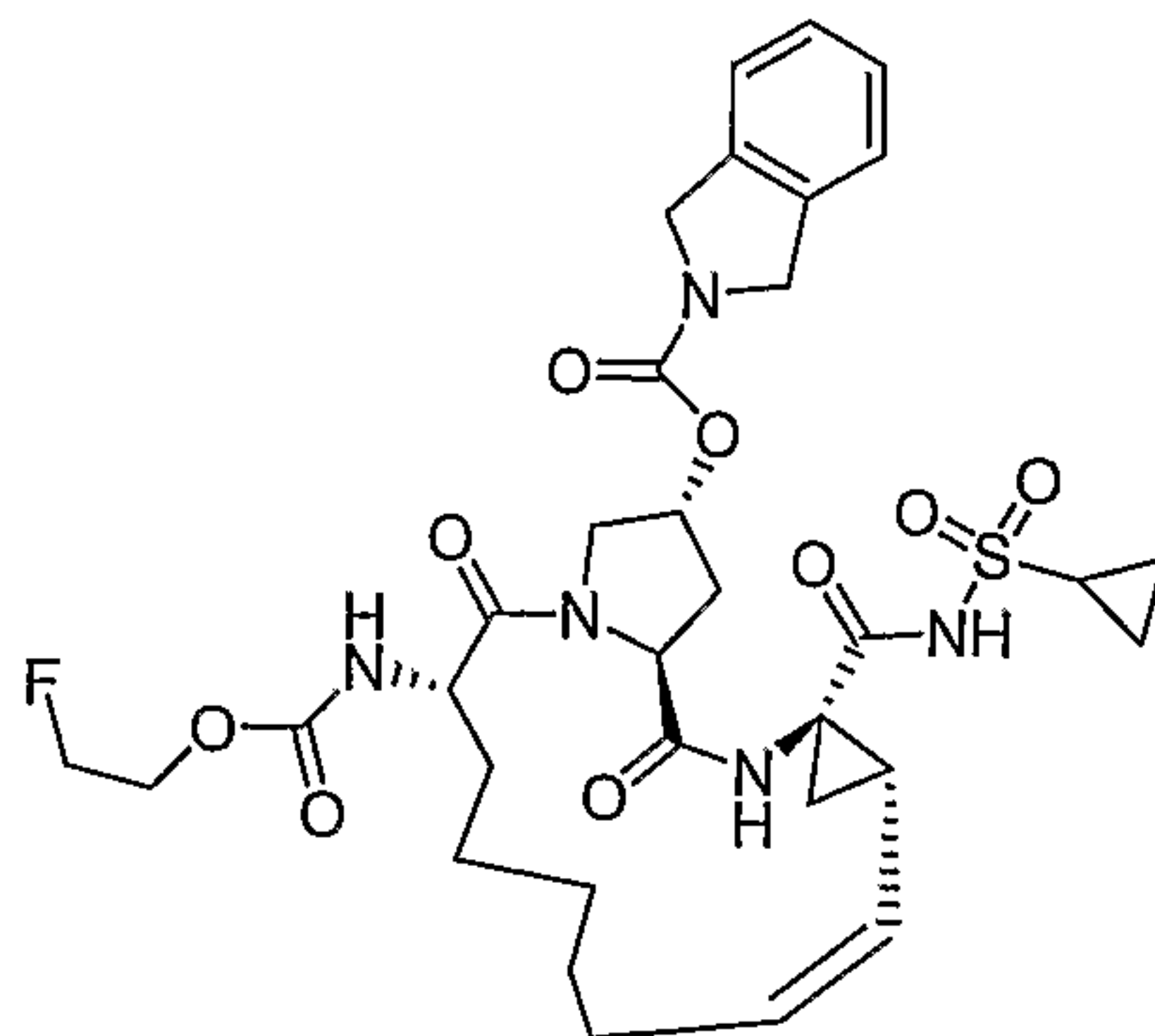
Compound AR00320073
