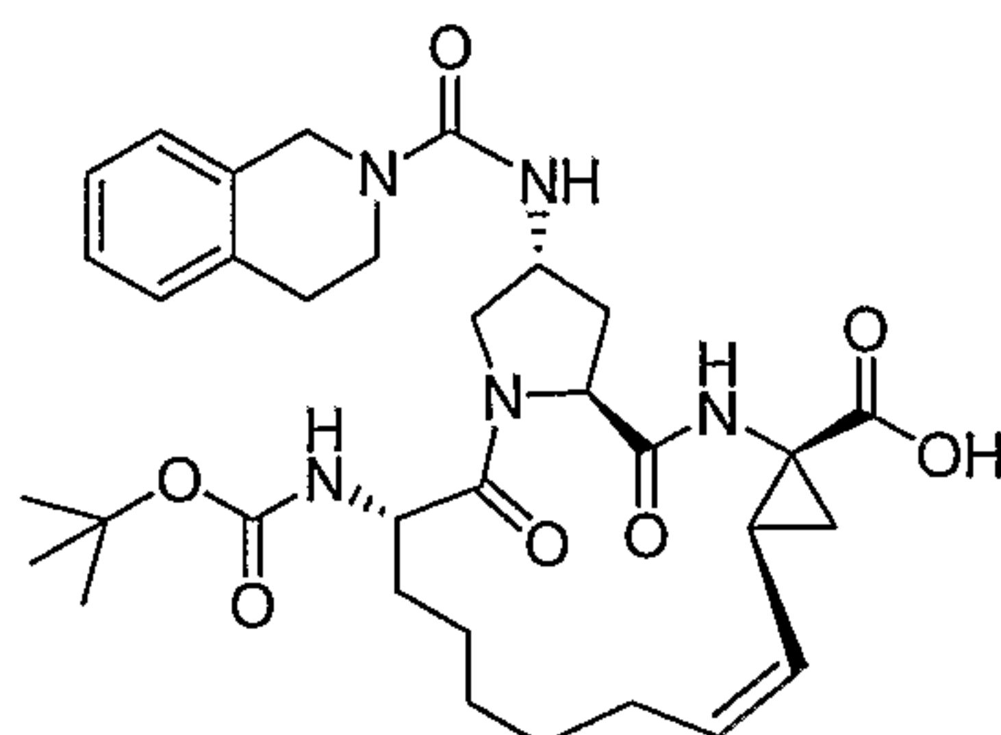
Compound AR00287262
