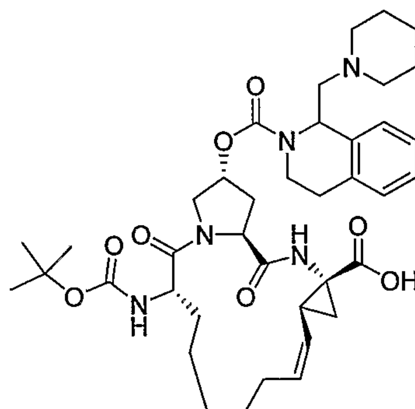
Compound AR00301383
