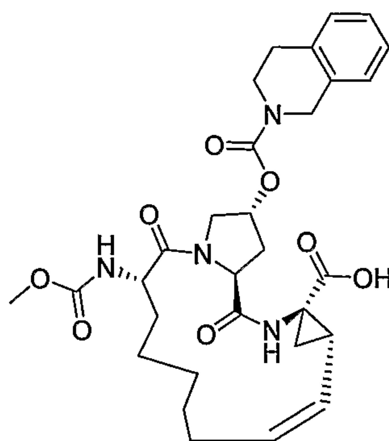
Compound AR00294376
