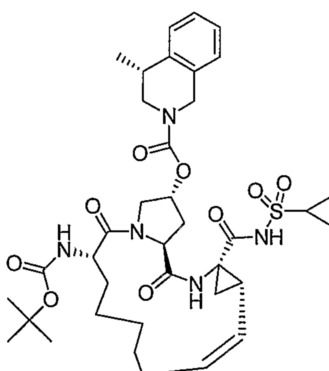
Compound AR00333462
