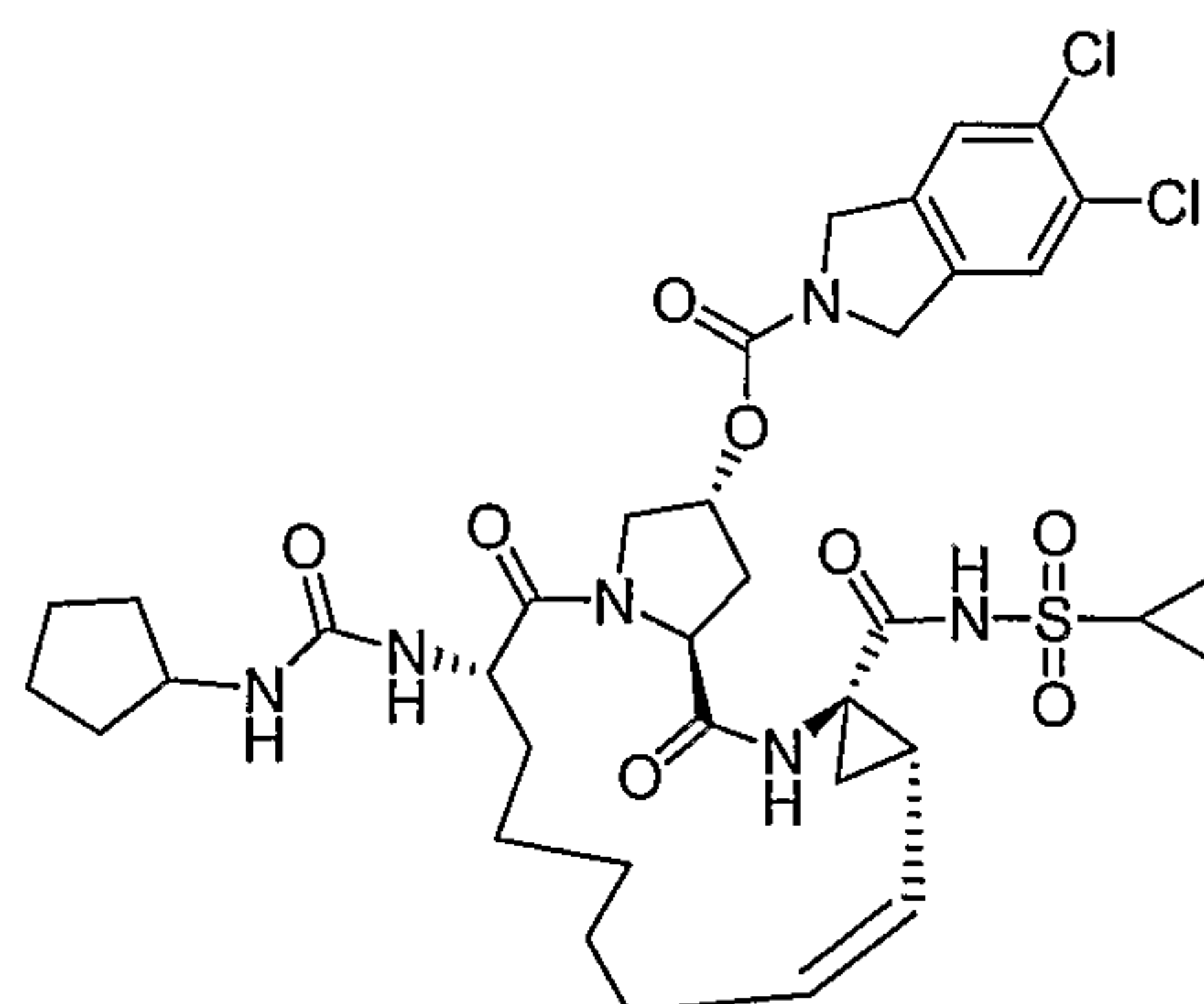
Compound AR00320575
