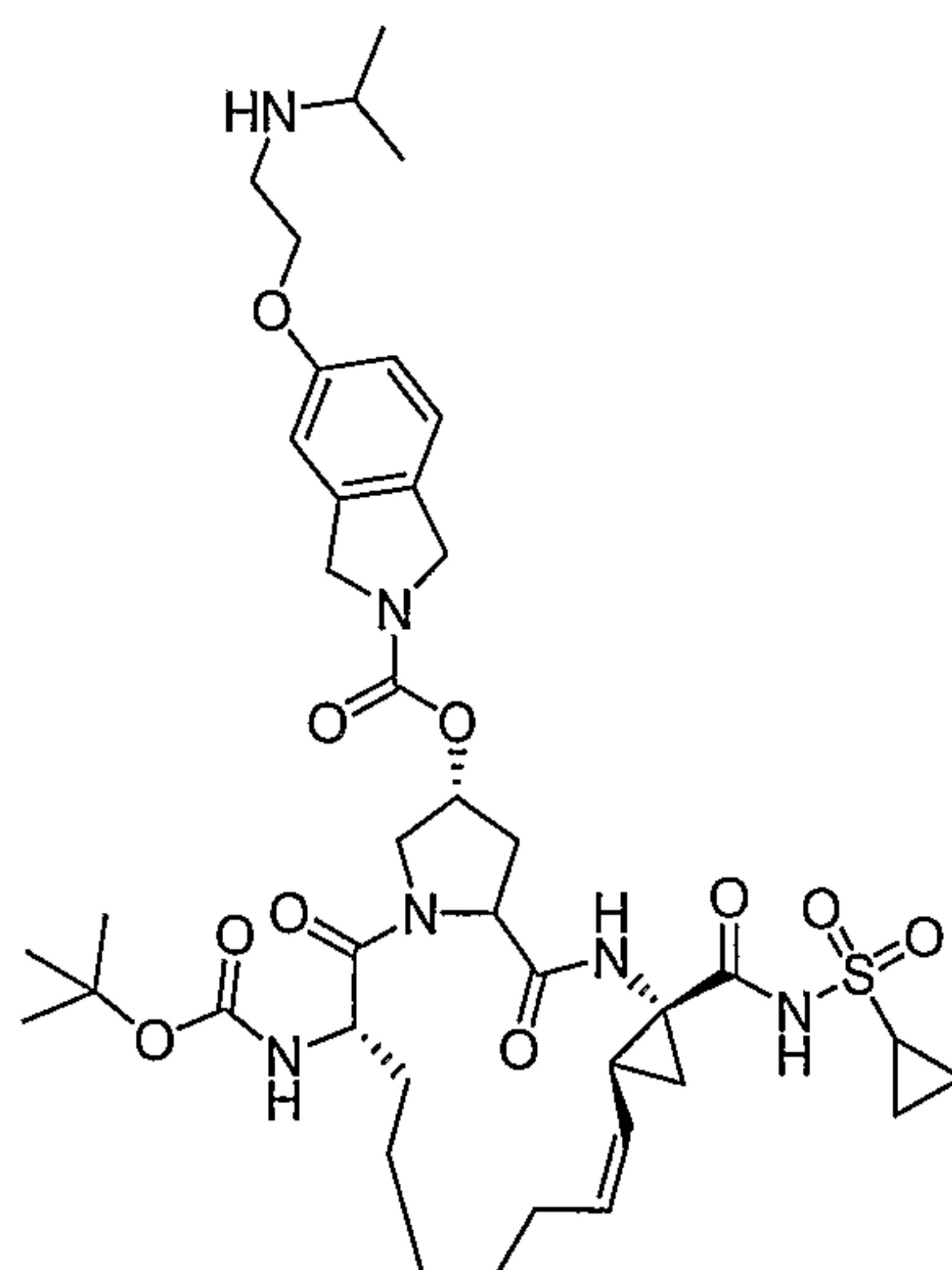
Compound AR00345094
