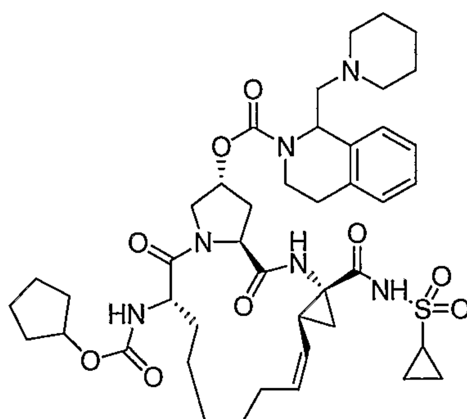
Compound AR00320506
