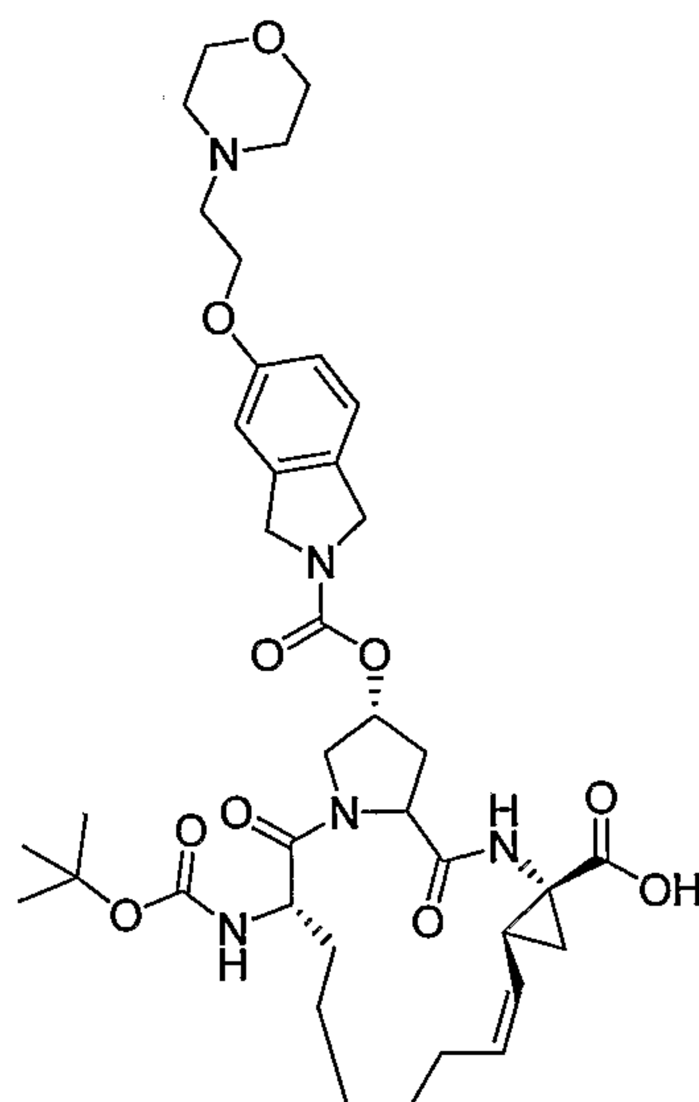
Compound AR00371946
