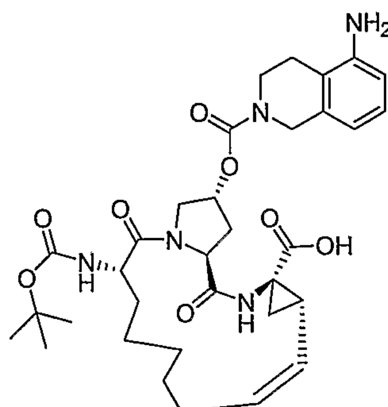
Compound AR00301745
