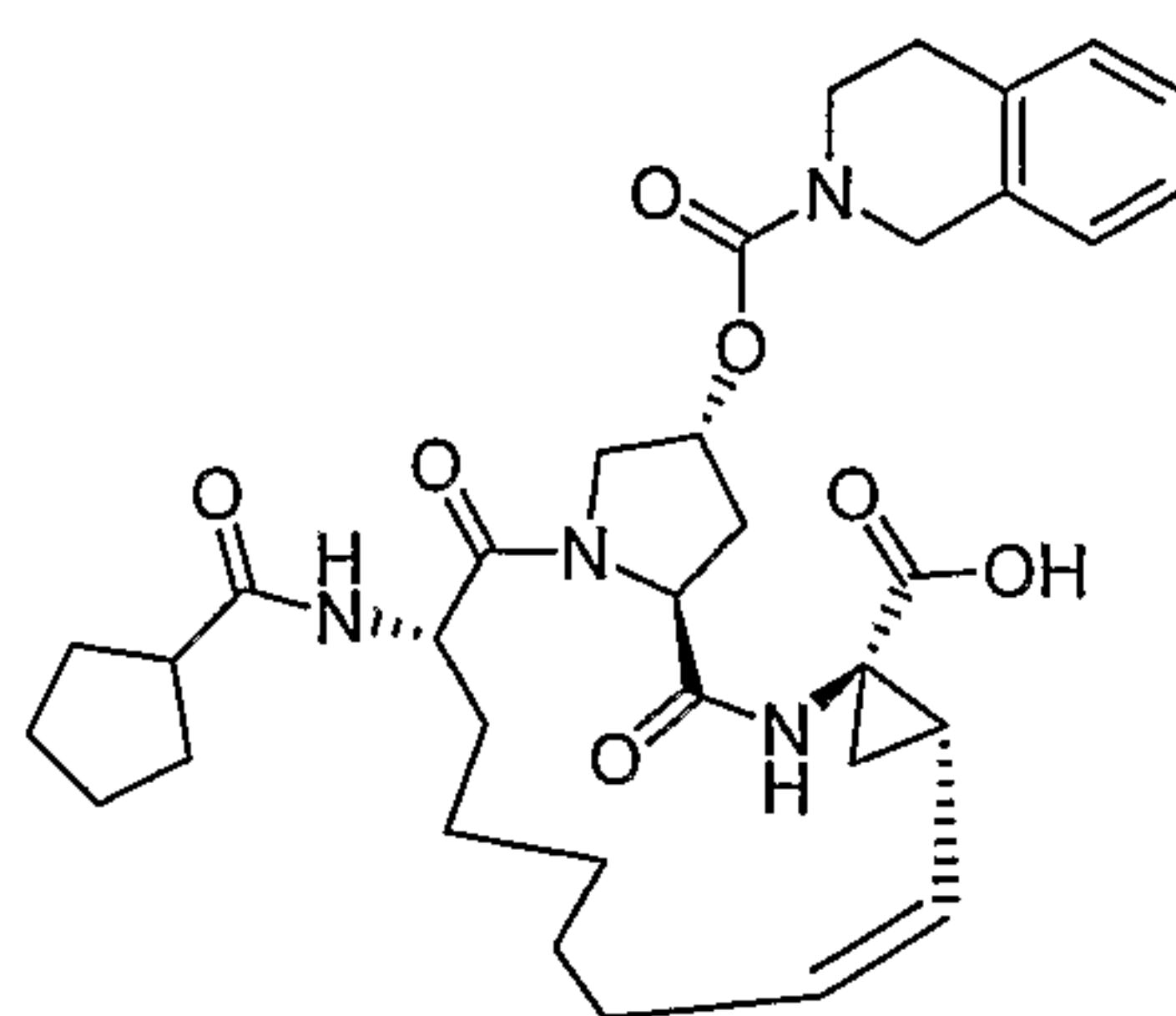
AR00248689
