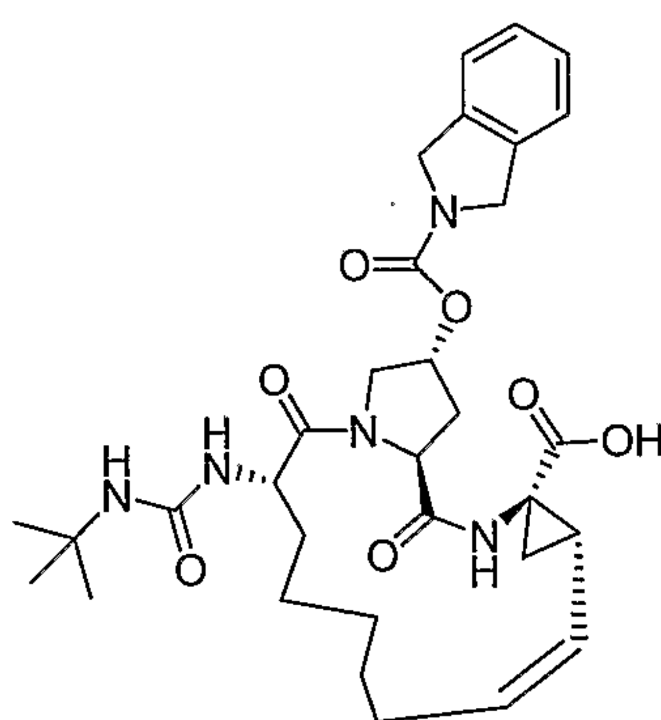
Compound AR00320078
