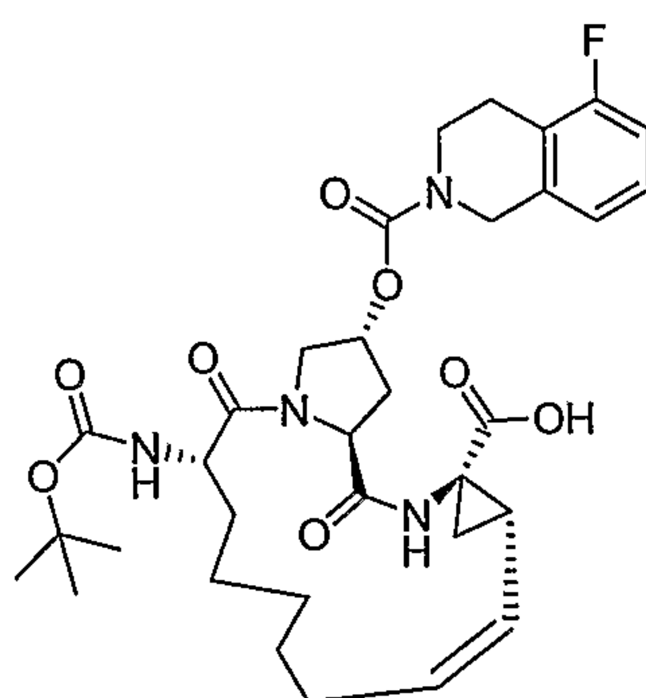
Compound AR00294384
