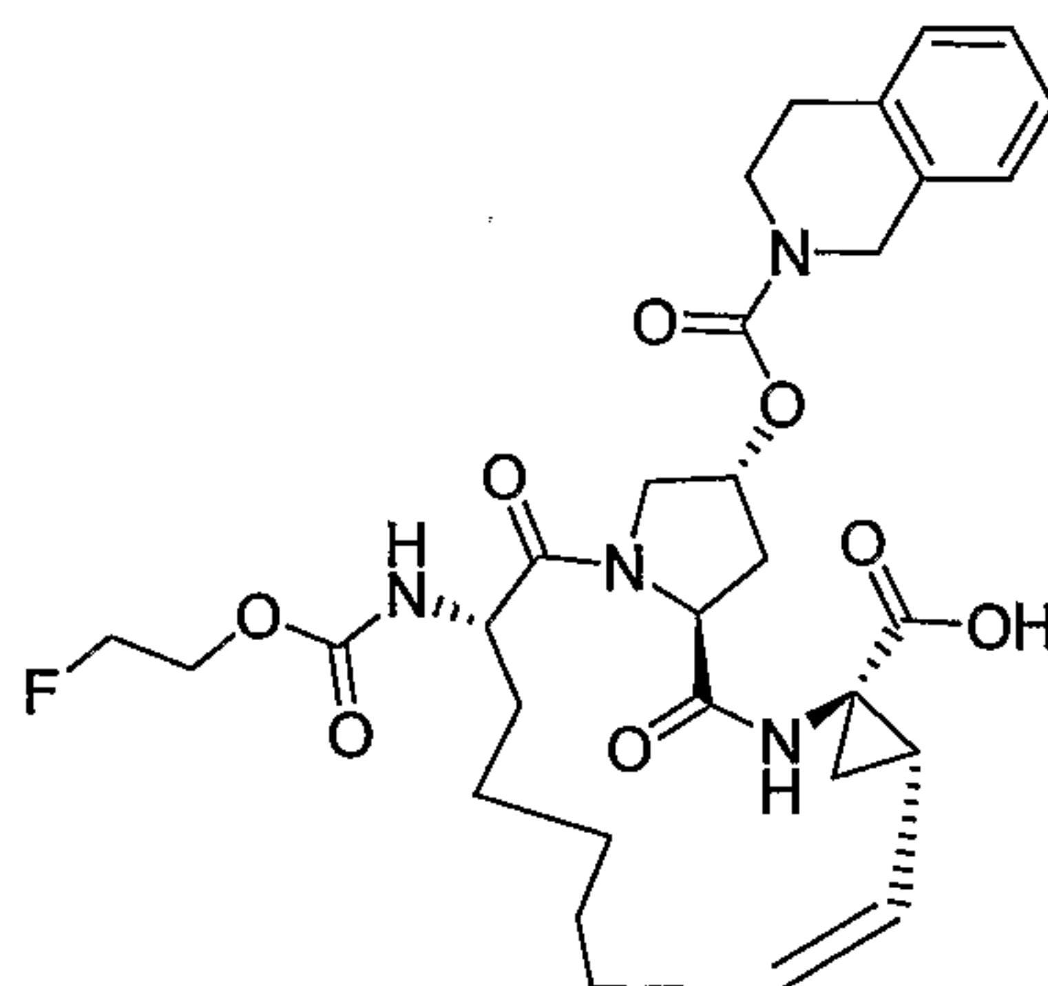
Compound AR00304125
