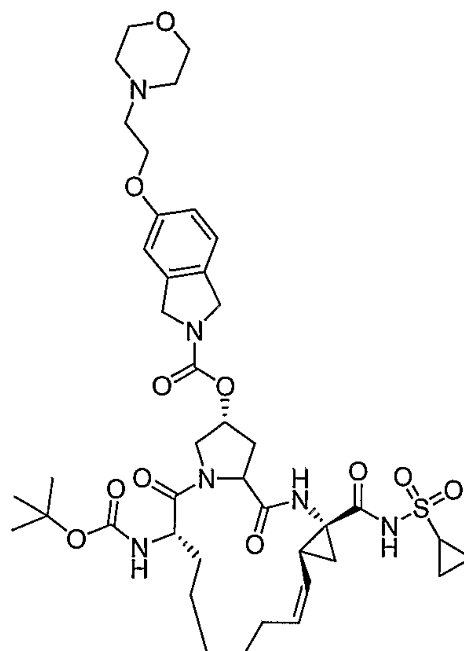
Compound AR00345090
