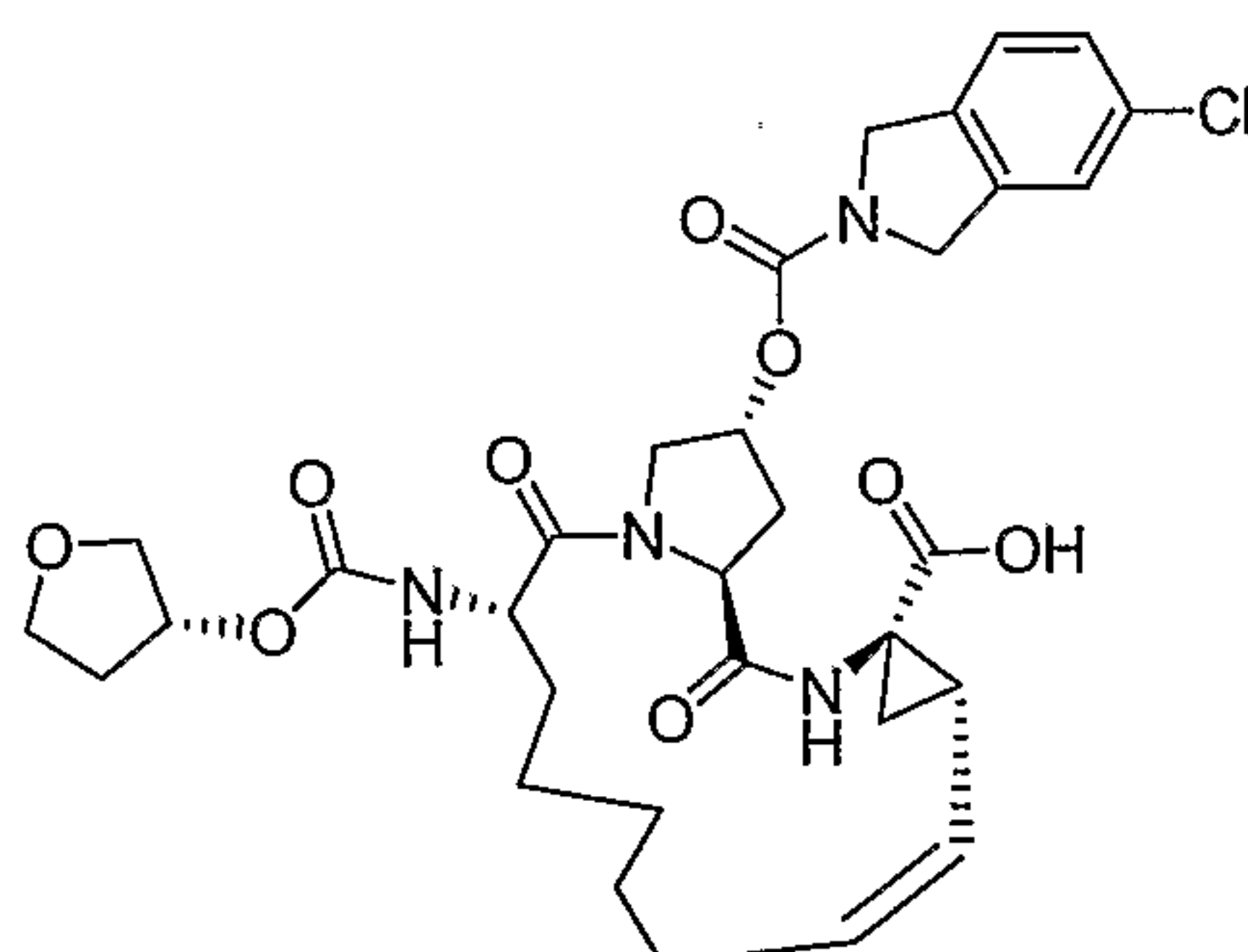
Compound AR00320448
