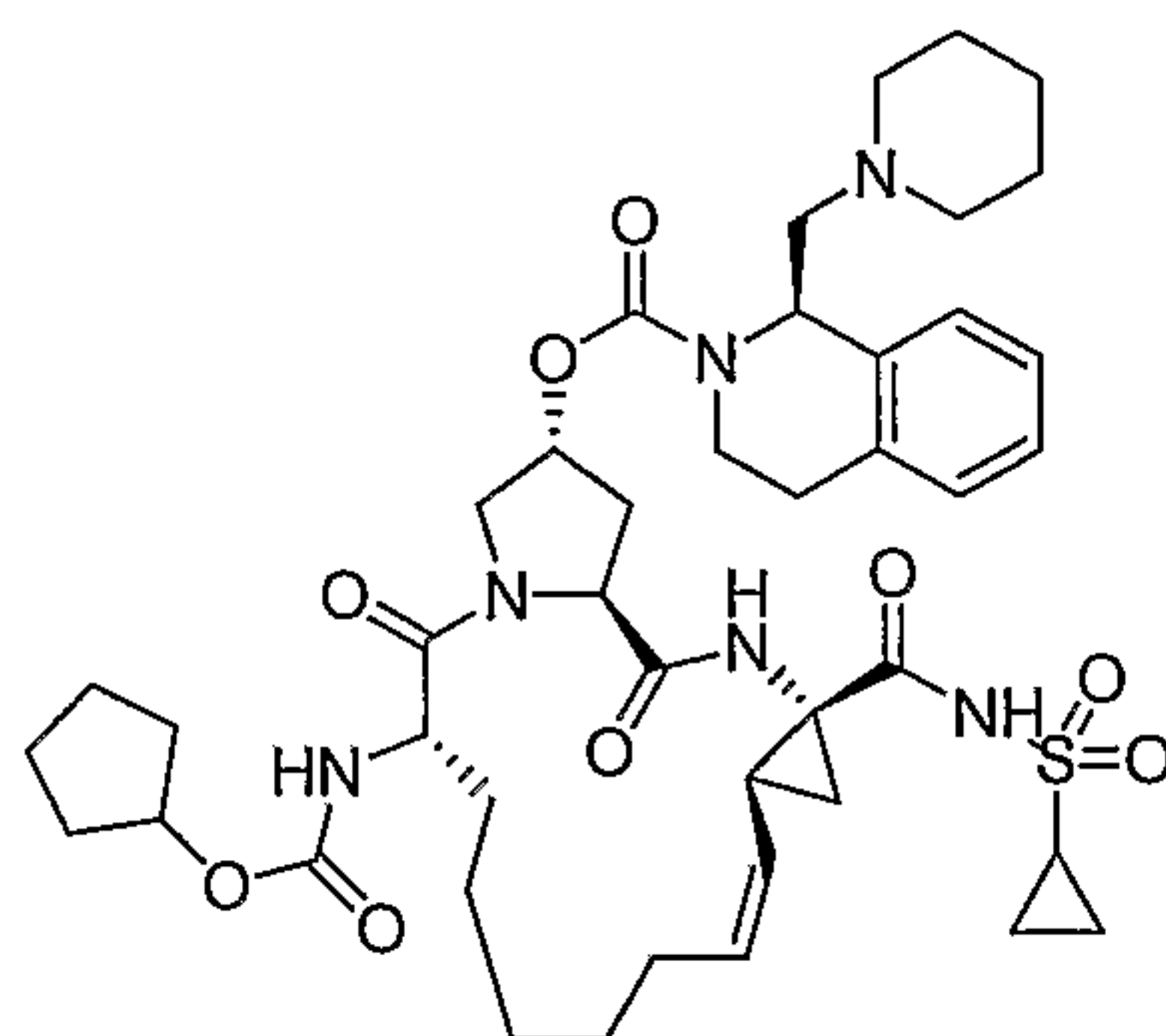
Compound AR00320556
