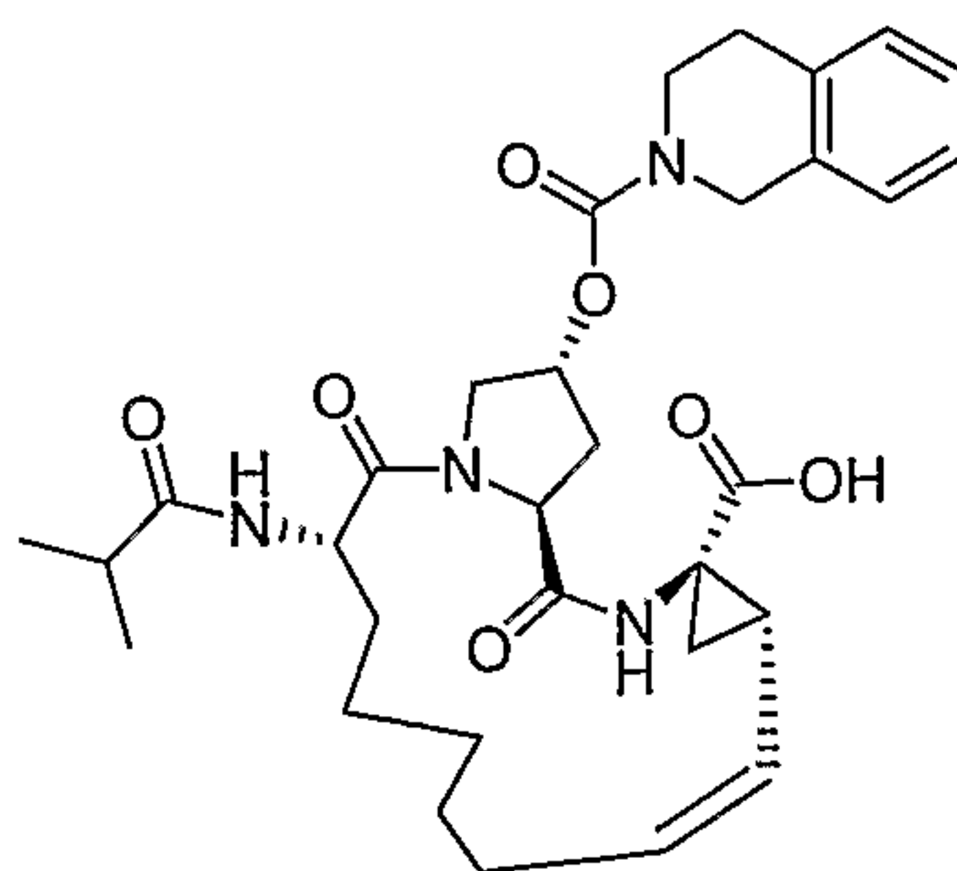
Compound AR00248688
