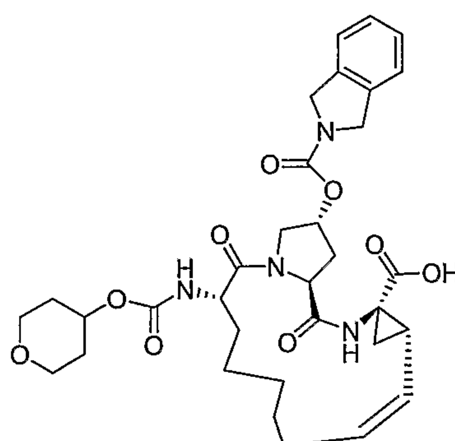
Compound AR00320077
