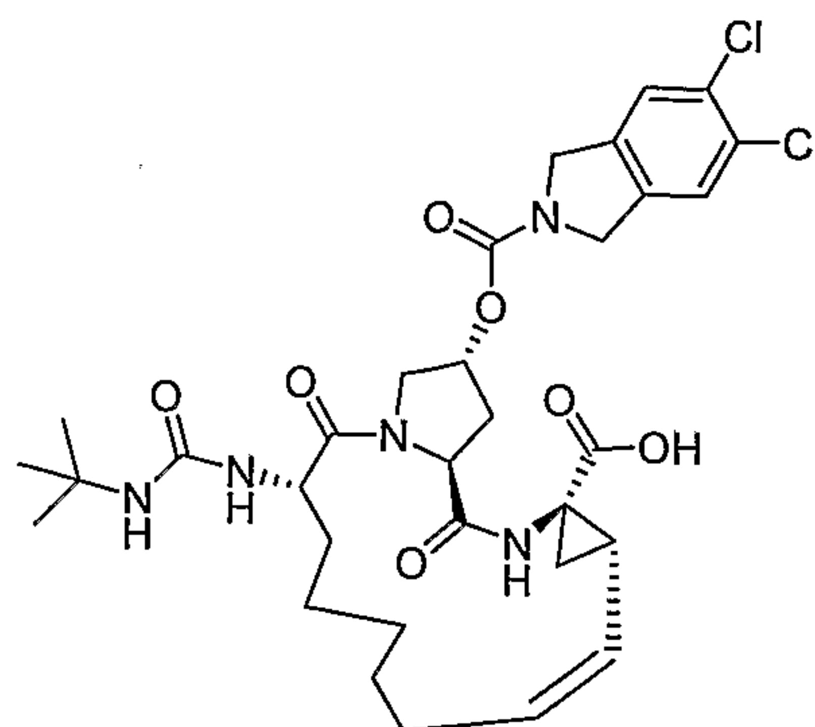
Compound AR00320450
