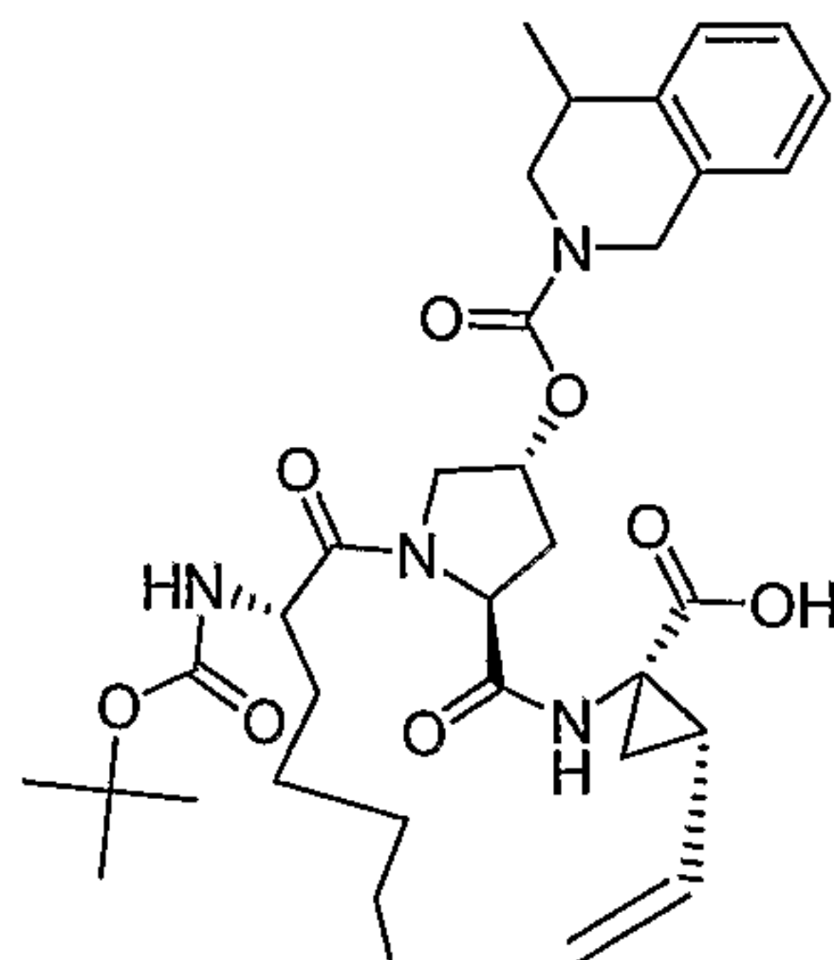
Compound AR00304067
