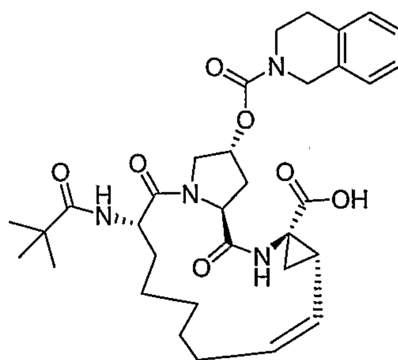
Compound AR00248687
