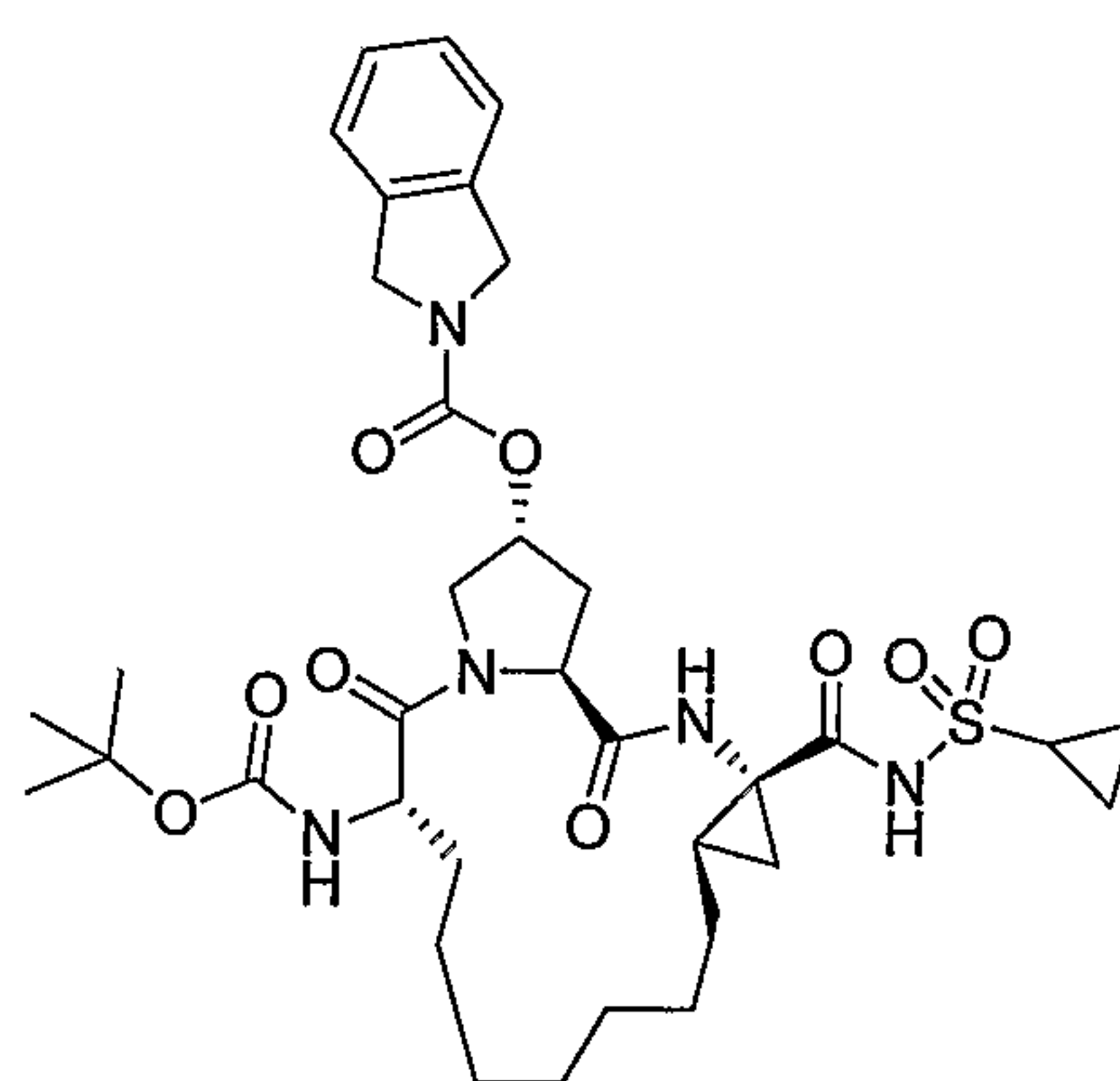
Compound AR00333833
