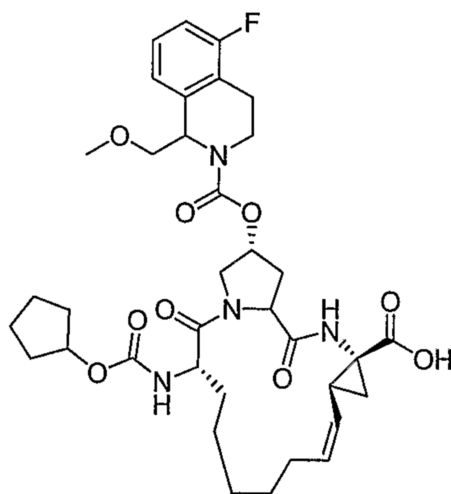
Compound AR00365381
