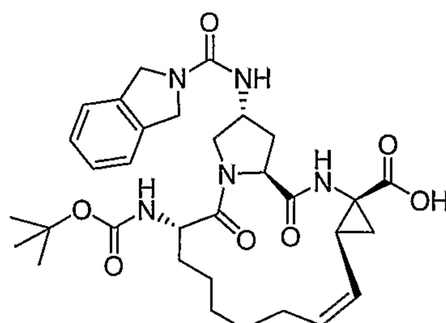
Compound AR00298980
