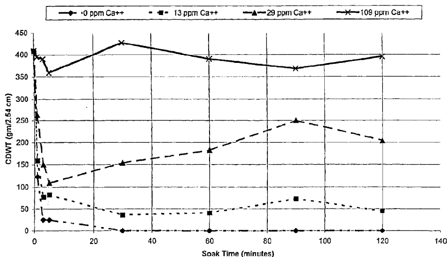
CDWT versus Soak Time in Calcium Ion Solutions - Basesheet with 85% Lion SSB-3b Ion-Sensitive Binder and 15% Dur-O-Set RB Cobinder - Wetted with a Solution Containing 0.9% NaCl
