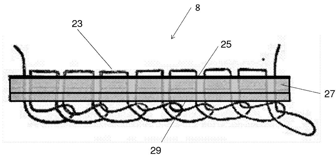
Fig 3: Single needle single thread chain stitch cross sectional view
