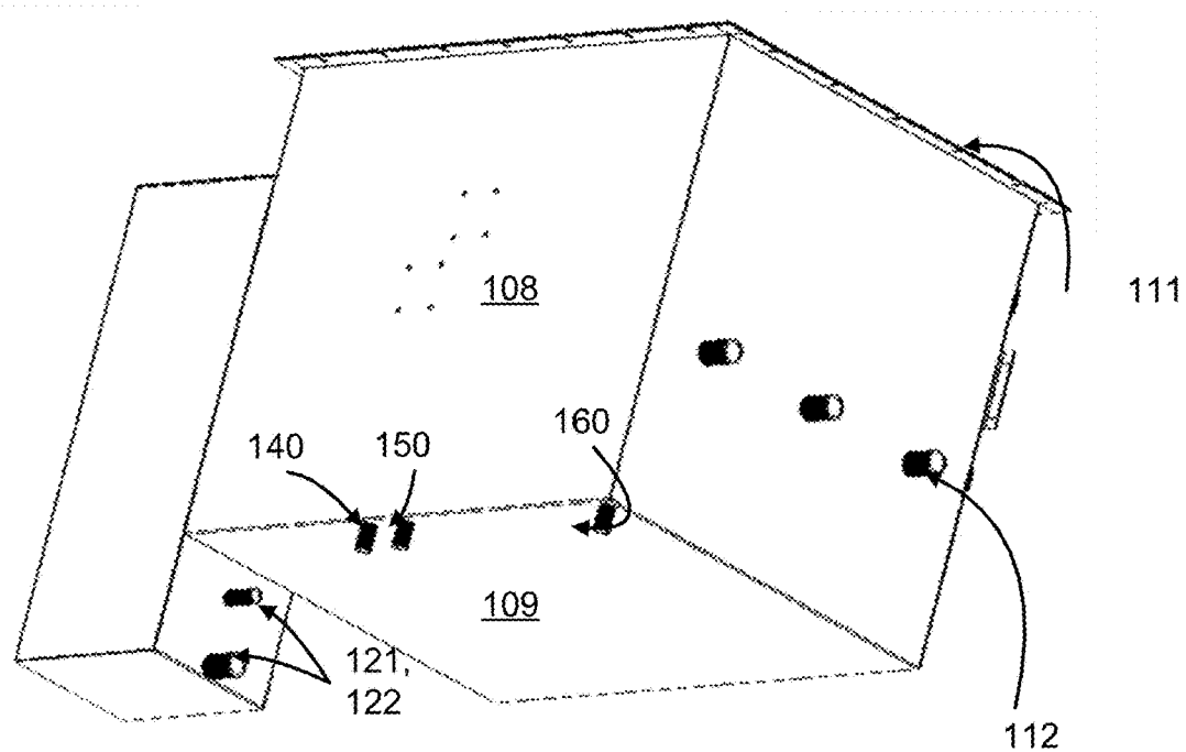
FIGURE 7C Tank – Rear Isometric View
