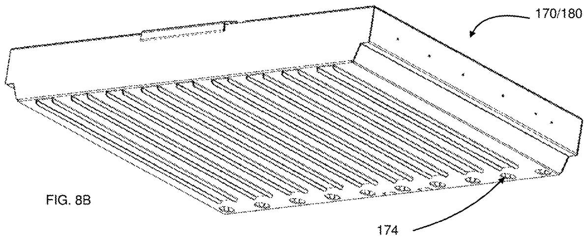
FIGURE 8 Drawers – Top and Bottom Views
