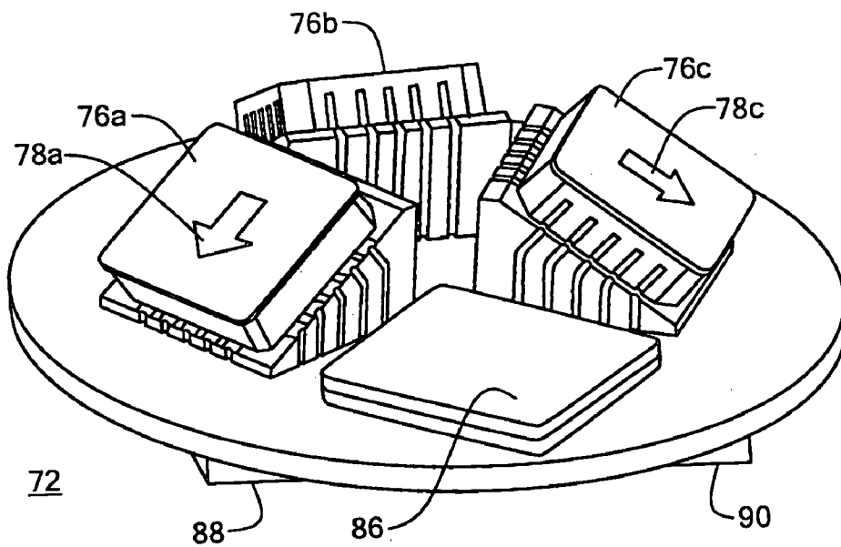
Gyro Board Assembly
