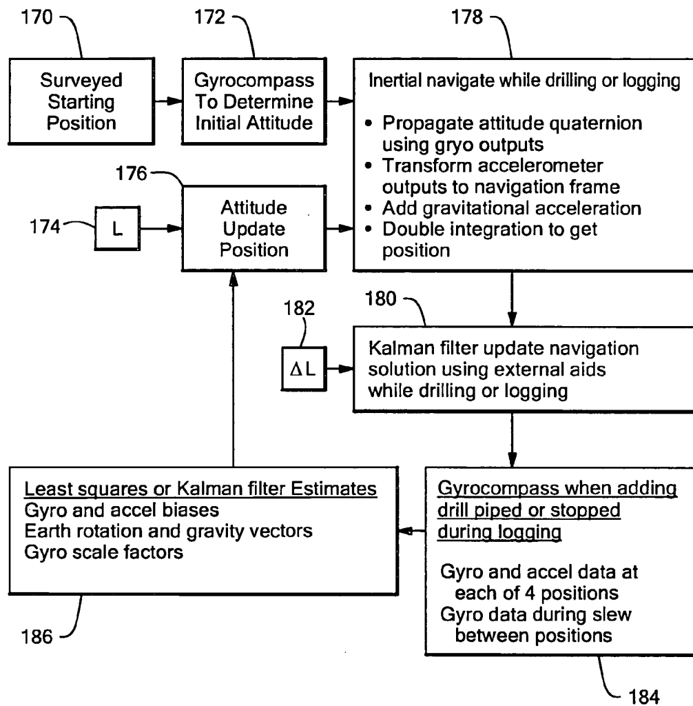
INERTIAL NAVIGATION WHILE DRILLING OR LOGGING
