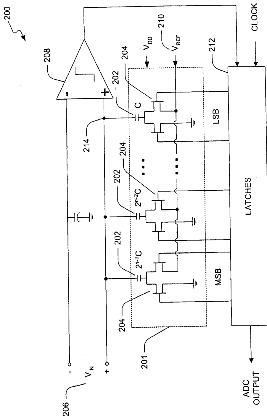
FIG. 2 (PRIOR ART)
