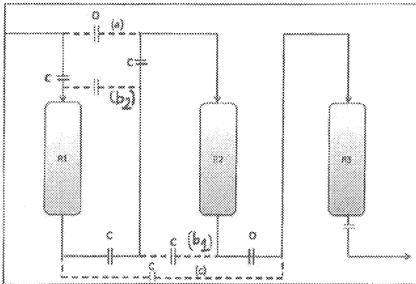
Figure 1: fixed additional connections during the changing of the catalyst of R1.
