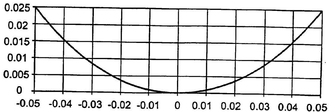
COSH Dimple Profile a=20, r=0.05, d=0.025, vr=0.51
