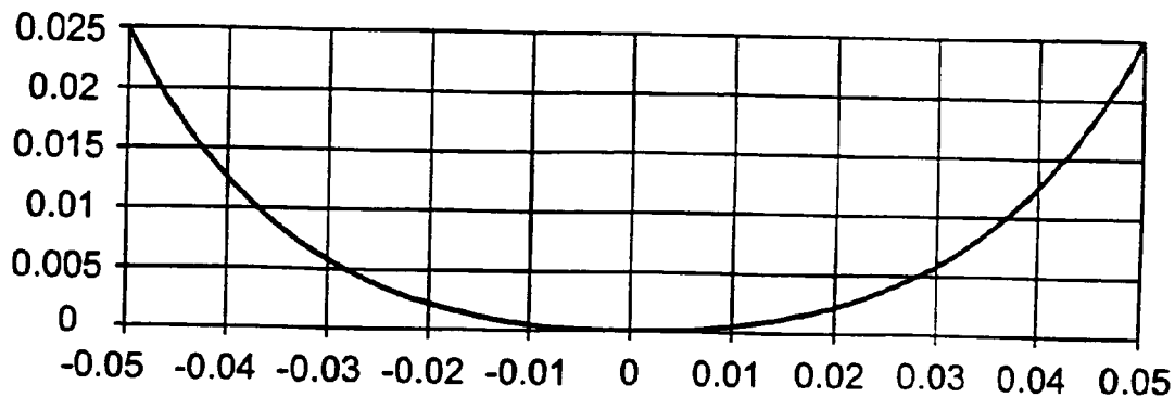
COSH Dimple Profile a=60, r=0.05, d=0.025, v_r=0.60
