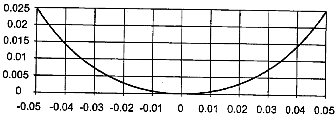
COSH Dimple Profile a=40, r=0.05, d=0.025, vr=0.55
