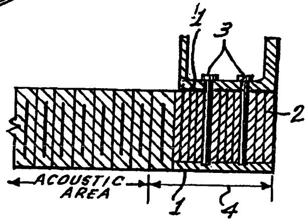
Fig. 2. (PRIOR ART)
