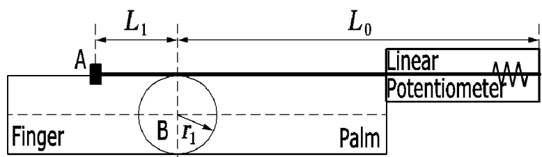
(b) Initial position of the finger
