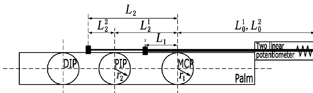
(a) Schematic of the proposed system(multi-joint case)
