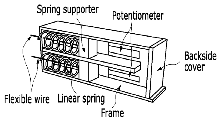
(a) Cross section of the sensing module
