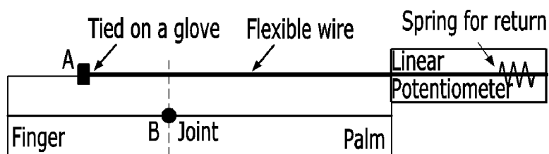
(a) Schematic of the proposed system
