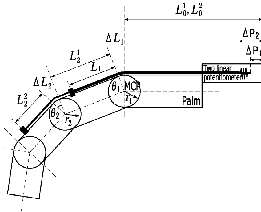
(b) Flexed finger
