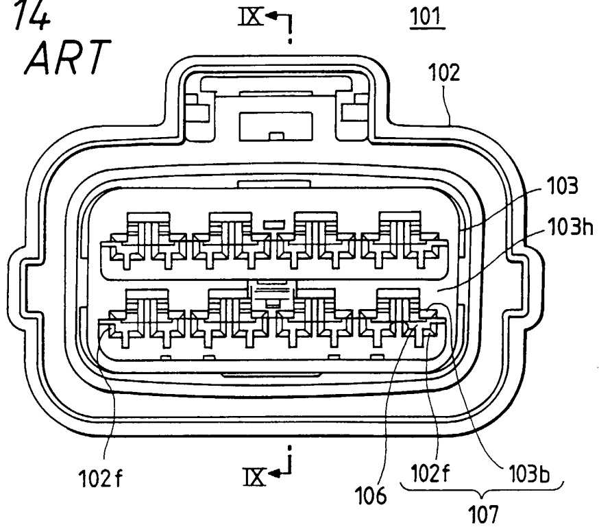
FIG. 15 PRIOR ART
