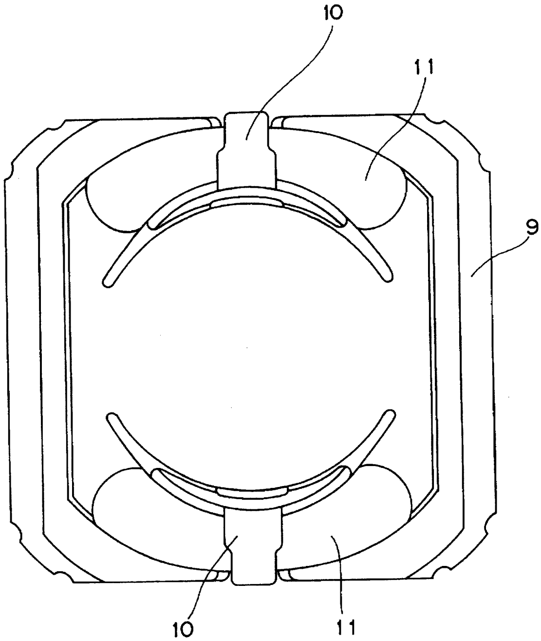
Fig. 7 PRIOR ART
