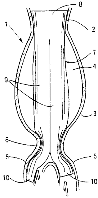
FIG. 1 PRIOR ART
