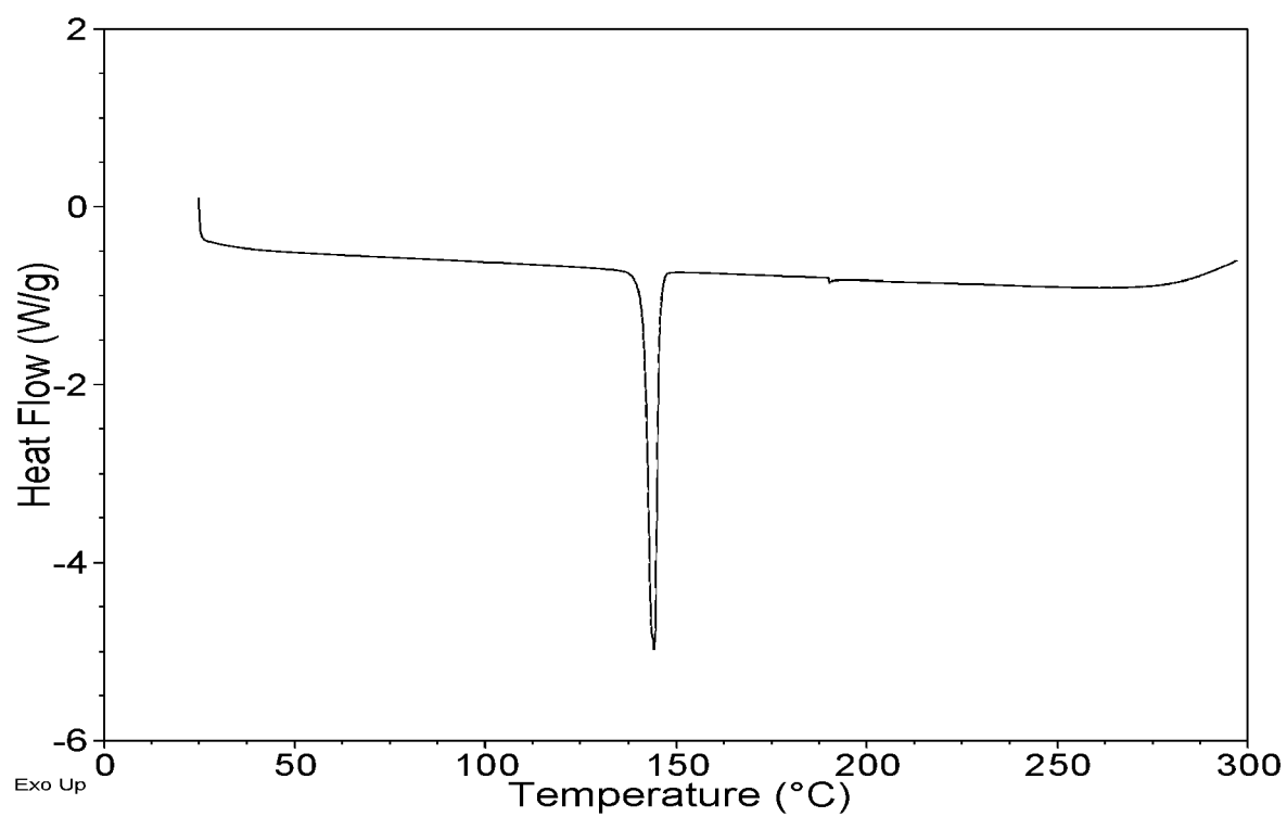
Figure 2: DSC Thermogram of Form A of 7-Fluoro-1-isopropyl-3-methyl-8-[6-[3-(1-piperidyl)propoxy]-3-pyridyl]imidazo[4,5-c]quinolin-2-one
