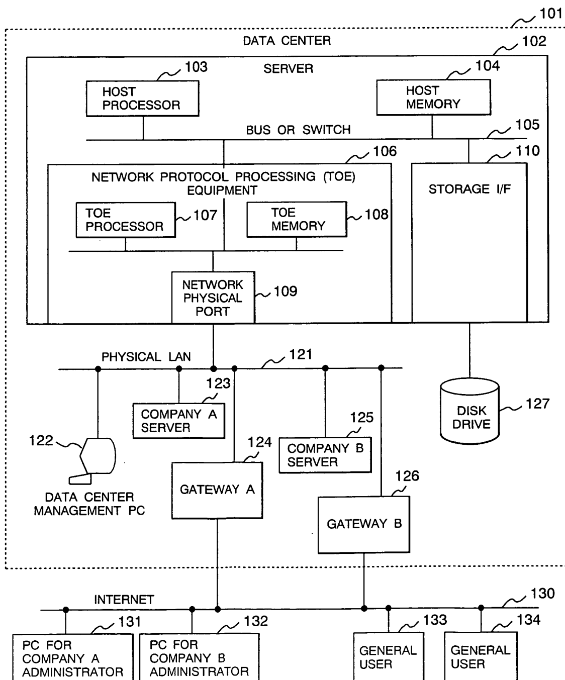
PHYSICAL NETWORK CONFIGURATION DIAGRAM
