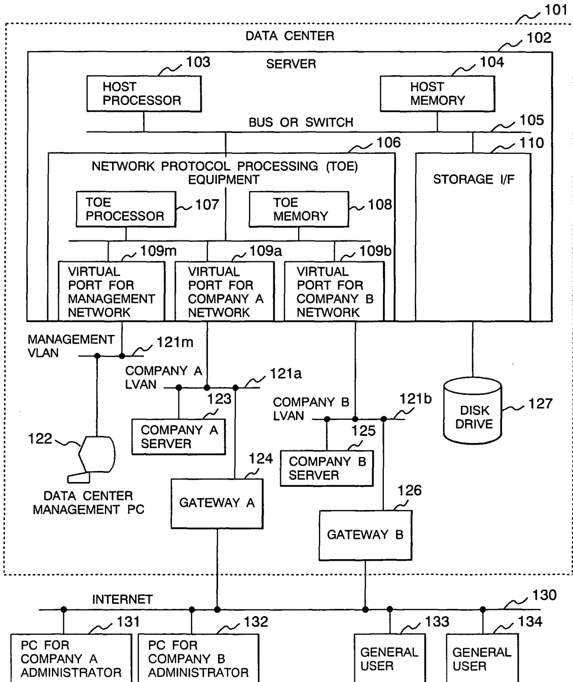
LOGICAL NETWORK CONFIGURATION DIAGRAM
