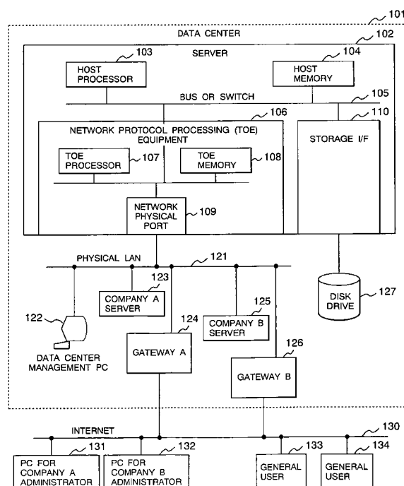
PHYSICAL NETWORK CONFIGURATION DIAGRAM
