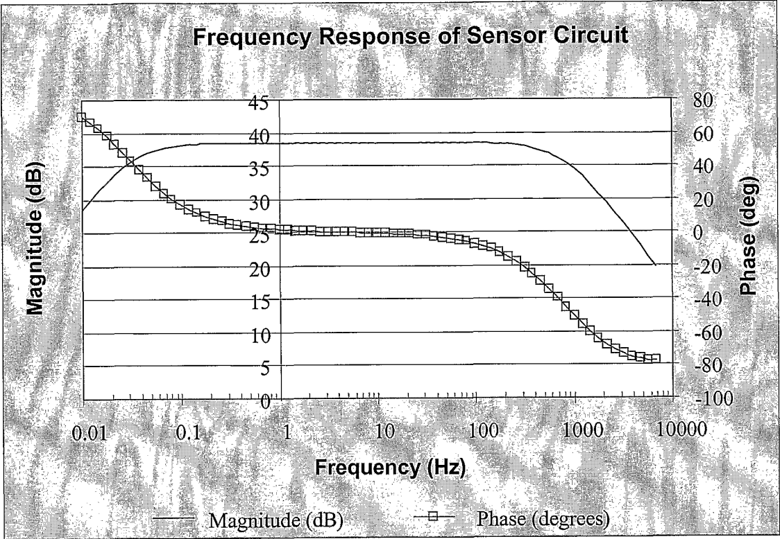
Figure 6: Frequency response of sensor
