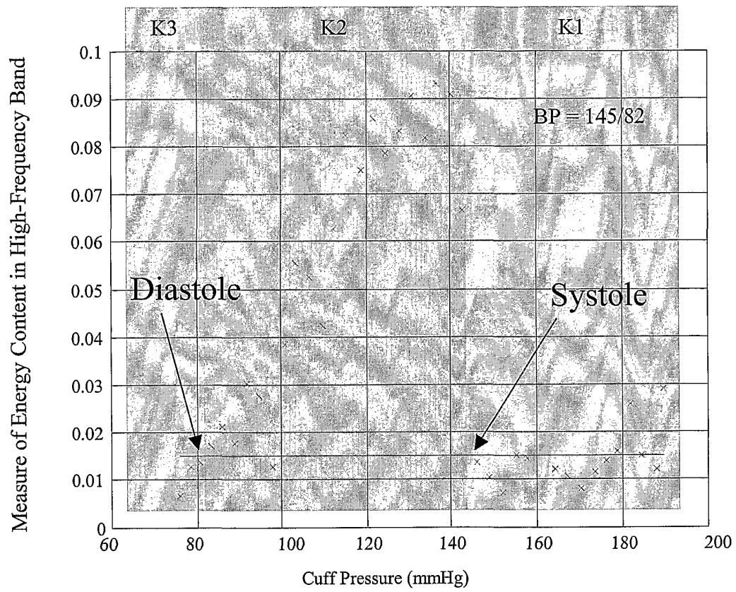
Figure 8: High frequency content of recorded beats
