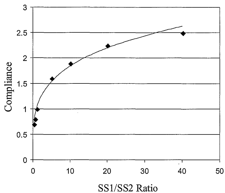
Figure 19: Relationship between SS1/SS2 and compliance.
