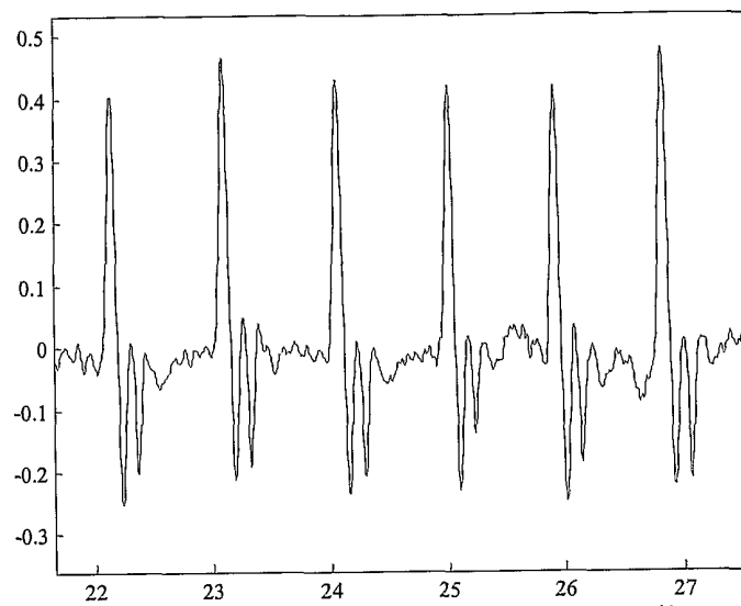
Figure 21: Effect of normal respiration on suprasystolic waveforms.
