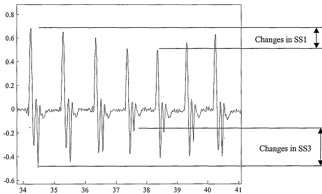
Figure 22: Changes in suprasystolic signal due to labored breathing.
