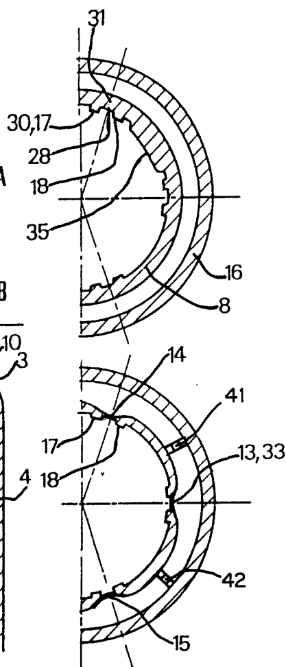
FIG. 4 HALF-SECTION BB
