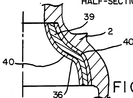
FIG. 4 HALF-SECTION BB
