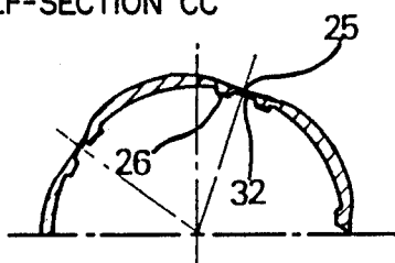
FIG. 3 HALF-SECTION CC
