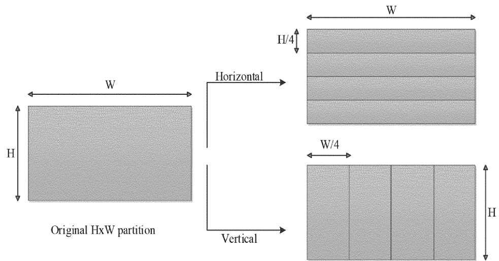
FIG. 8: Example of division of all blocks except 4 \times 8 , 8 \times 4 and 4 \times 4
