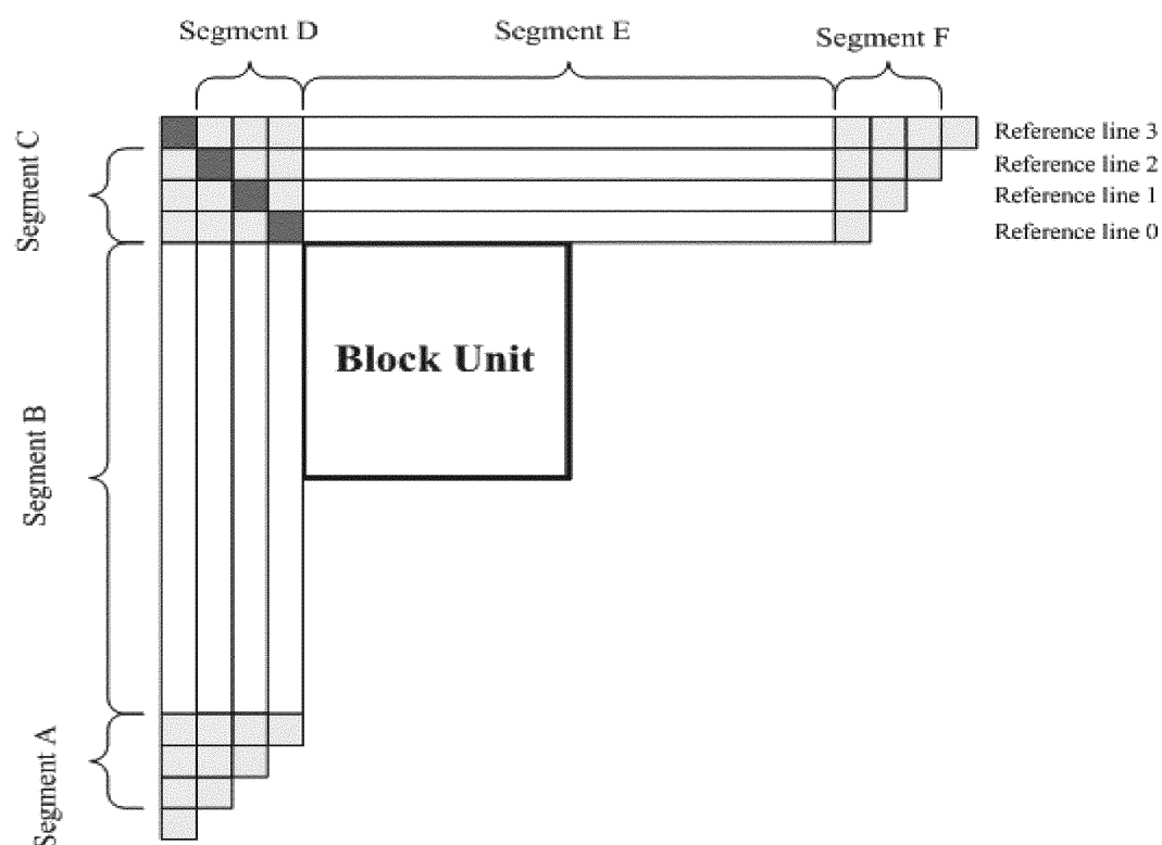
FIG. 6, Multiple reference line coding tool, indication of neighboring reference line. When reference line index equals to 0, the closest neighboring reference line to current block is used.
