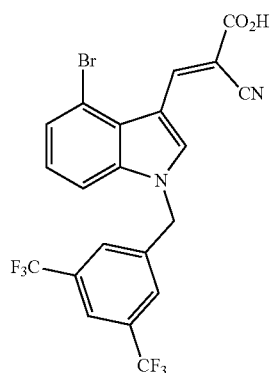
(E)-3-(1-(3,5-Bis(trifluoromethyl)benzyl)-4-bromo-1H-indol-3-yl)-2-cyanoacrylic Acid (JXL051)
