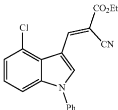
Ethyl (E)-3-(4-chloro-1-phenyl-1H-indol-3-yl)-2-cyanoacrylate (JXL093)
