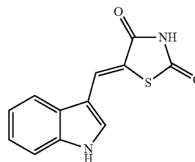
(Z)-5-((1H-Indol-3-yl)methylene)thiazolidine-2,4-dione (JXL075)
