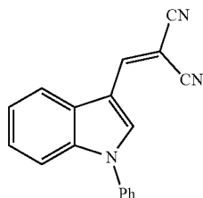
2-((1-Phenyl-1H-indol-3-yl)methylene)malononitrile (JXL021)
