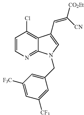
Ethyl (E)-3-(1-(3,5-bis(trifluoromethyl)benzyl)-4-chloro-1H-pyrrolo[2,3-b]pyridin-3-yl)-2-cyanoacrylate (JXL087)
