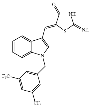
(Z)-5-((1-(3,5-Bis(trifluoromethyl)benzyl)-1H-indol-3-yl)methylene)-2-iminothiazolidin-4-one (JXL067)
