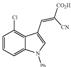
(E)-3-(4-Chloro-1-phenyl-1H-indol-3-yl)-2-cyanoacrylic acid (JXL035)
