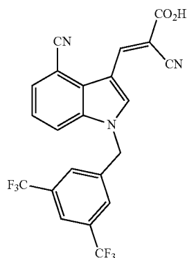
(E)-3-(1-(3,5-Bis(trifluoromethyl)benzyl)-4-cyano-1H-indol-3-yl)-2-cyanoacrylic Acid (JXL055)
