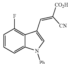
(E)-2-Cyano-3-(4-fluoro-1-phenyl-1H-indol-3-yl) acrylic Acid (JXL026)
