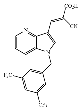
(E)-3-(1-(3,5-Bis(trifluoromethyl)benzyl)-1H-pyrrolo[3,2-b]pyridin-3-yl)-2-cyanoacrylic Acid (JXL072)
