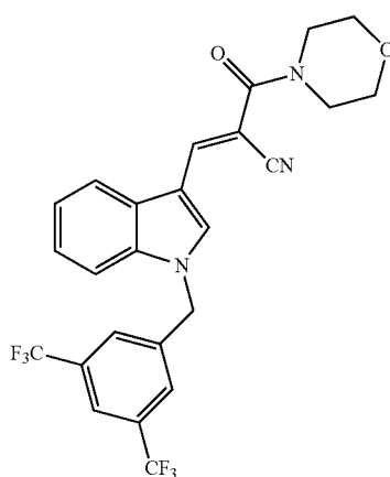
(E)-3-(1-(3,5-Bis(trifluoromethyl)benzyl)-1H-indol-3-yl)-2-(morpholine-4-carbonyl)acrylonitrile (JXL081)
