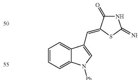
(Z)-2-imino-5-((1-phenyl-1H-indol-3-yl)methylene)thiazolidin-4-one (JXL023)
