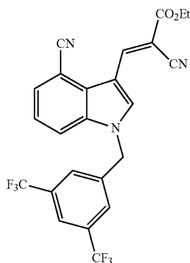
Ethyl (E)-3-(1-(3,5-bis(trifluoromethyl)benzyl)-4-cyano-1H-indol-3-yl)-2-cyanoacrylate (JXL090)
