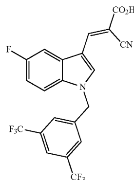
(E)-3-(1-(3,5-Bis(trifluoromethyl)benzyl)-5-fluoro-1H-indol-3-yl)-2-cyanoacrylic Acid (JXL038)
