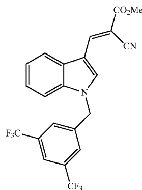
Methyl (E)-3-(1-(3,5-bis(trifluoromethyl)benzyl)-1H-indol-3-yl)-2-cyanoacrylate (JXL078)
