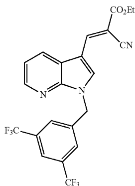
Ethyl (E)-3-(1-(3,5-bis(trifluoromethyl)benzyl)-1H-pyrrolo[2,3-b]pyridin-3-yl)-2-cyanoacrylate (JXL082)
