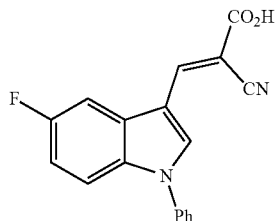
(E)-2-Cyano-3-(5-fluoro-1-phenyl-1H-indol-3-yl)acrylic Acid (JXL029)
