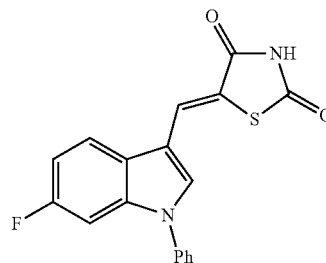
(Z)-5-((6-Fluoro-1-phenyl-1H-indol-3-yl)methylene)thiazolidine-2,4-dione (JXL071)
