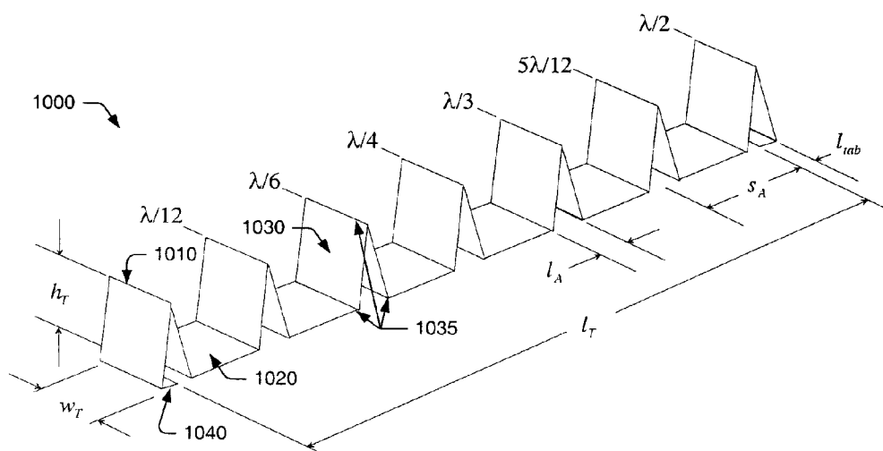
FIG. 10B FOLDED PATTERN
