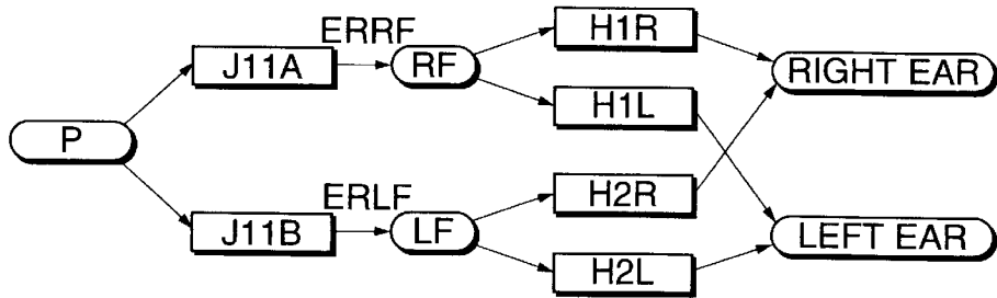
FIG.8B PRIMARY REFLECTED SOUND(ii)
