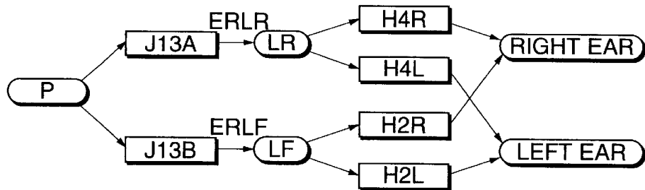
FIG.8D PRIMARY REFLECTED SOUND(iv)
