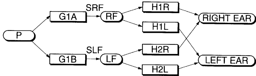
FIG.5A WHEN IMAGINARY SOUND SOURCE P IS POSITIONED BETWEEN RF AND LF
