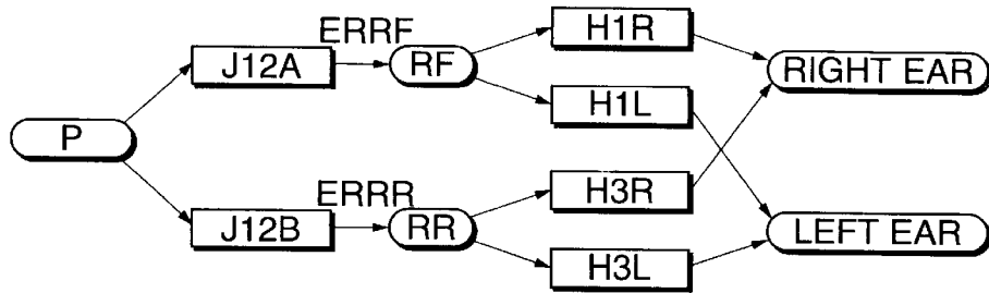
FIG.8C PRIMARY REFLECTED SOUND(iii)
