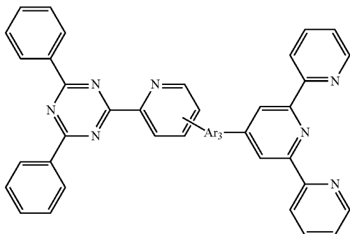
[Chemical Formula 4]
