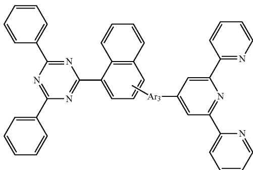
[Chemical Formula 5]
