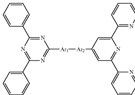
[Chemical Formula 1]
