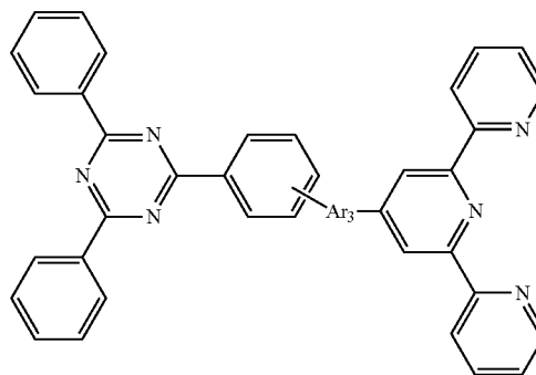
[Chemical Formula 3]
