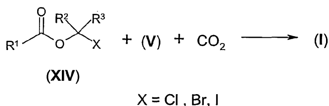
Scheme 6
