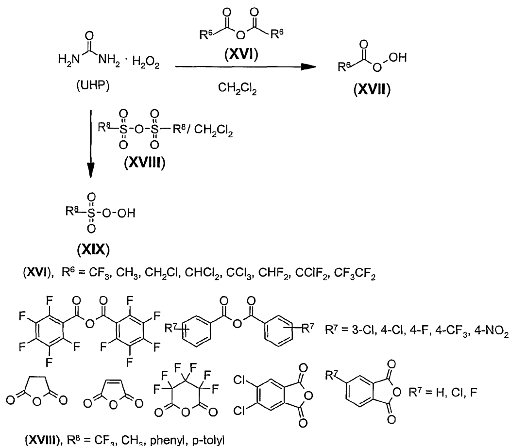
Scheme 8
