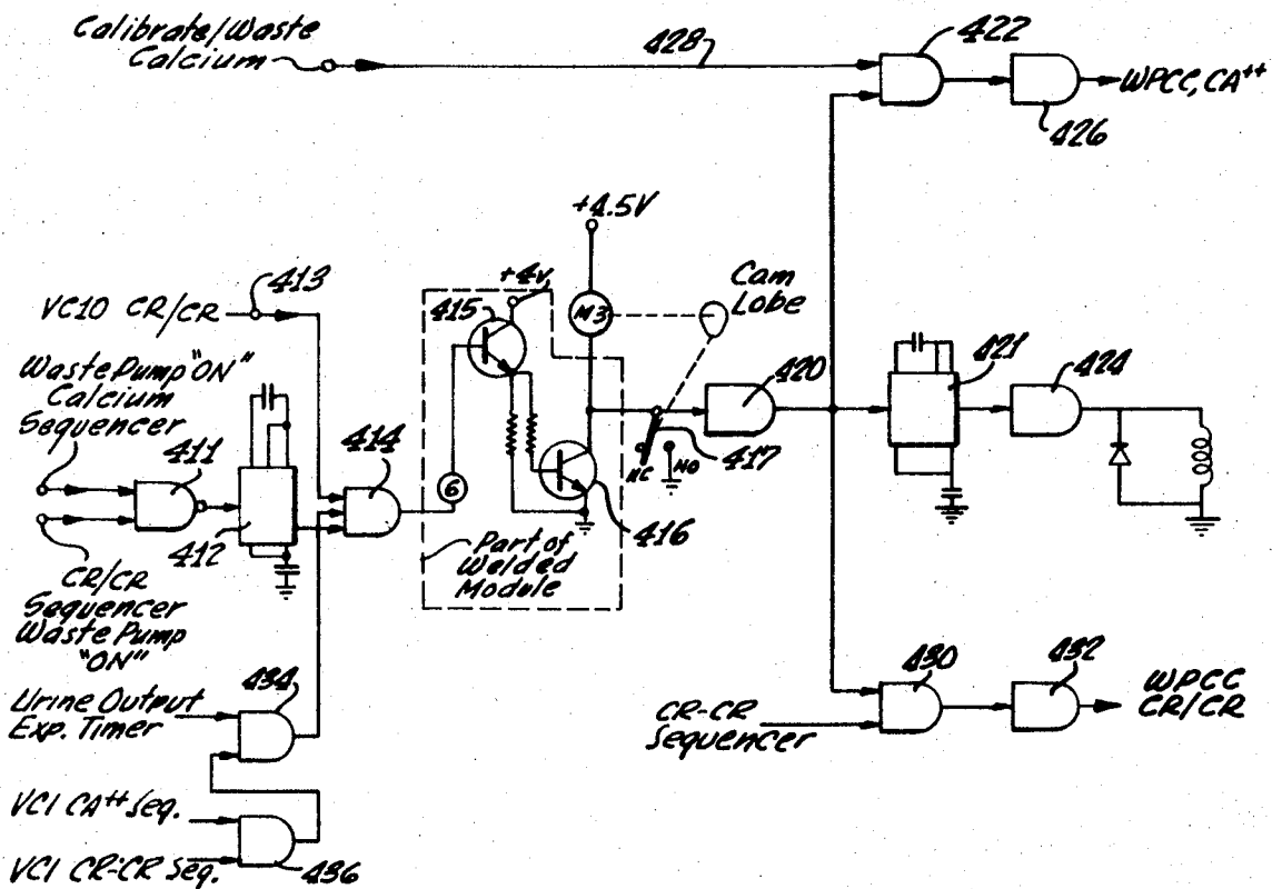
Fig. 15. (Waste Pump Circuit-408)
