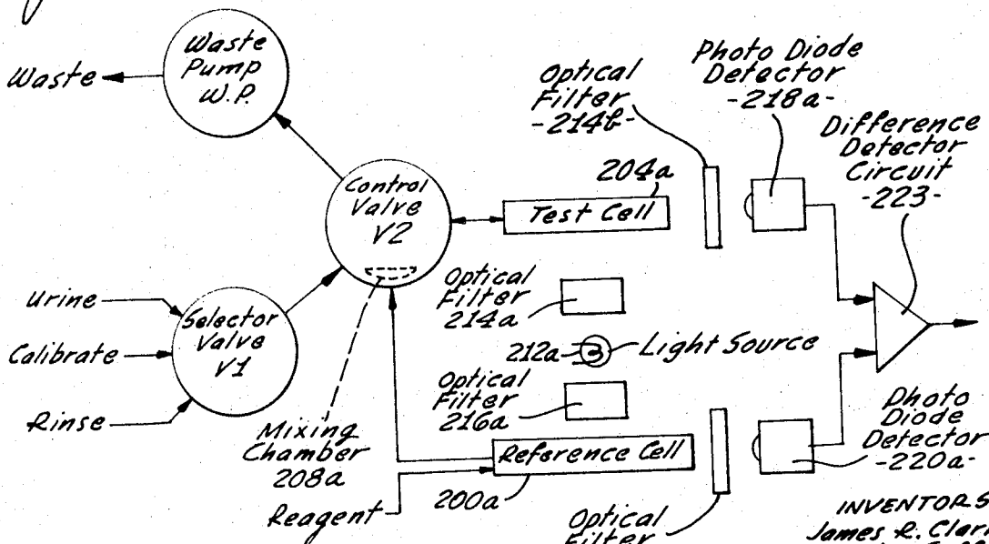
Fig. 4. (Functional Schematic of Present Embodiment (Calcium))
