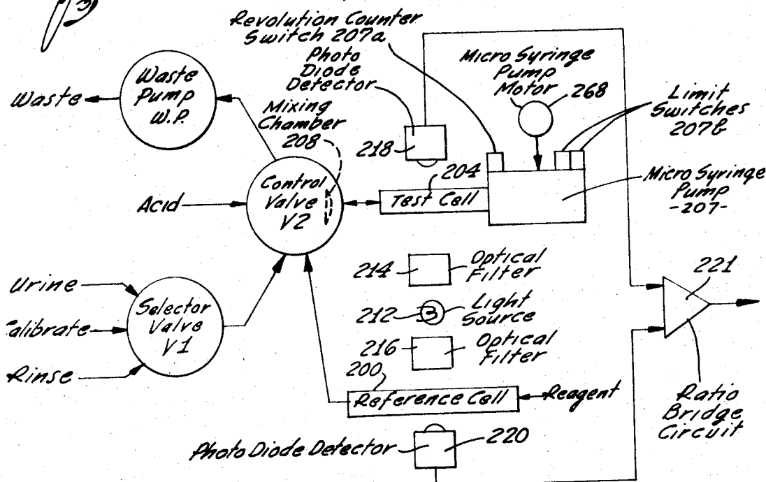
Fig. 4. (Functional Schematic of Present Embodiment (Calcium))
