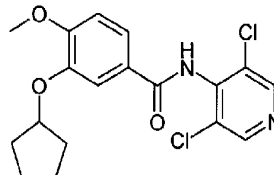
piclamilast
