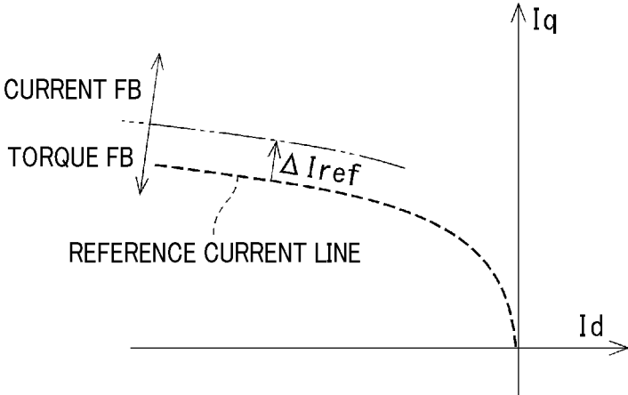
DEVIATION FROM REFERENCE CURRENT LINE
