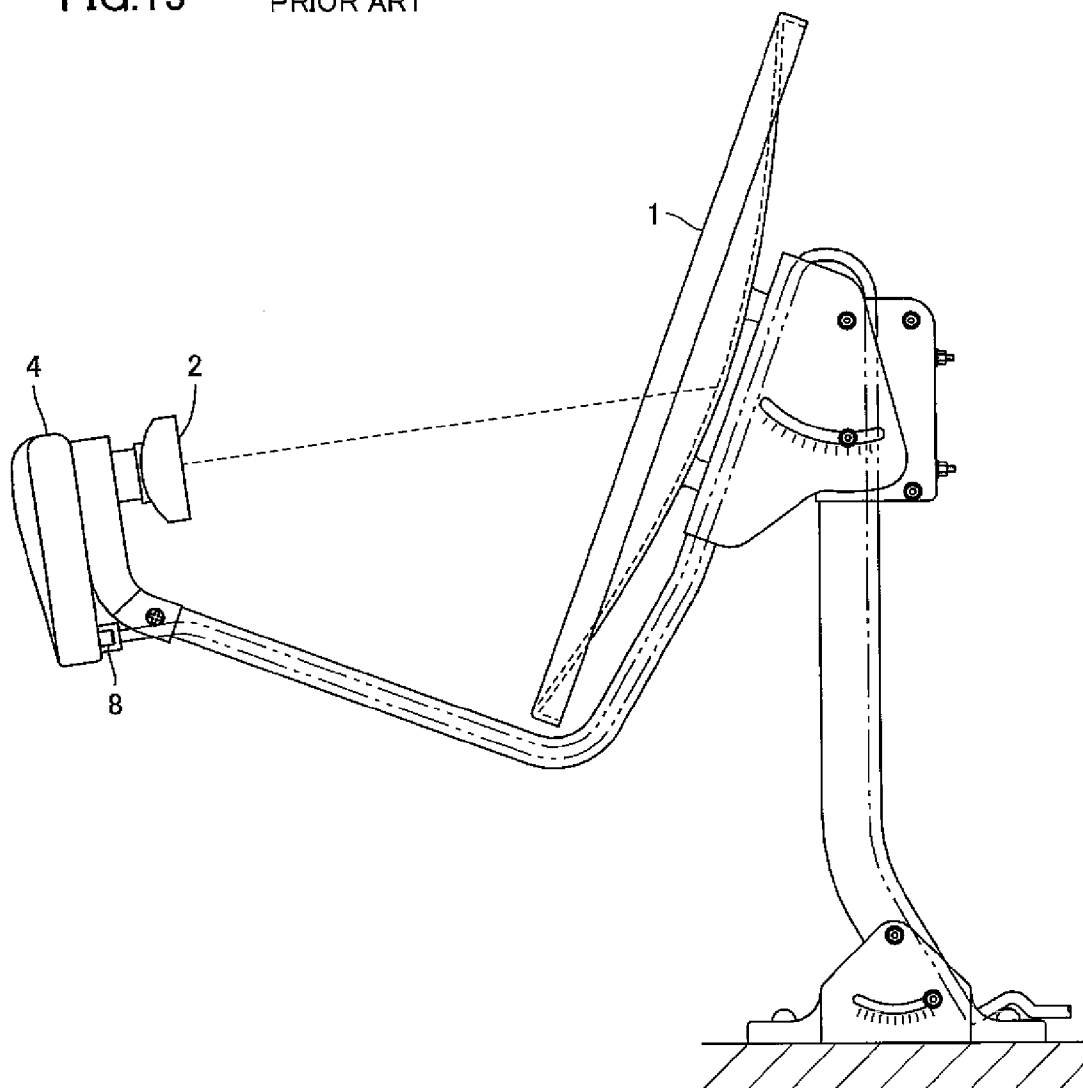
FIG.15 PRIOR ART
