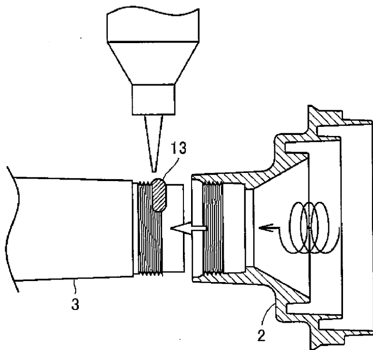
FIG.20 PRIOR ART
