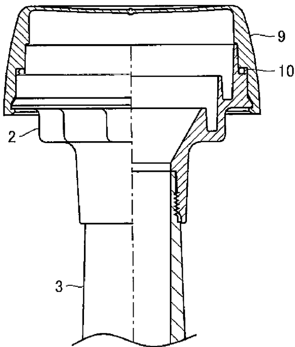
FIG.21 PRIOR ART
