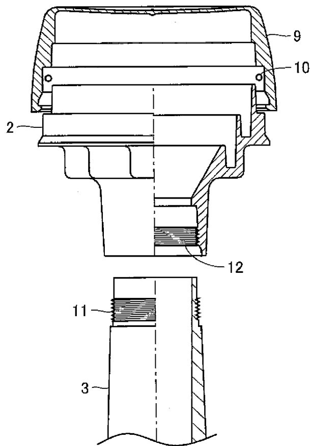
FIG.19 PRIOR ART
