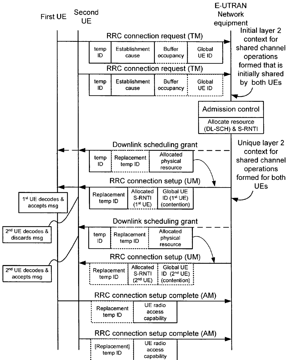
Scheduled downlink connection &amp; conflict resolution procedure
