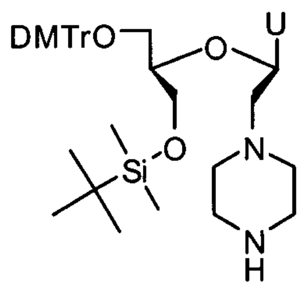
3'-O-tert-butyldimethylsilyl-2'-deoxy-5'-O-(4,4'-dimethoxytrityl)-2'-piperazino-2',3'-secouridine (108)
