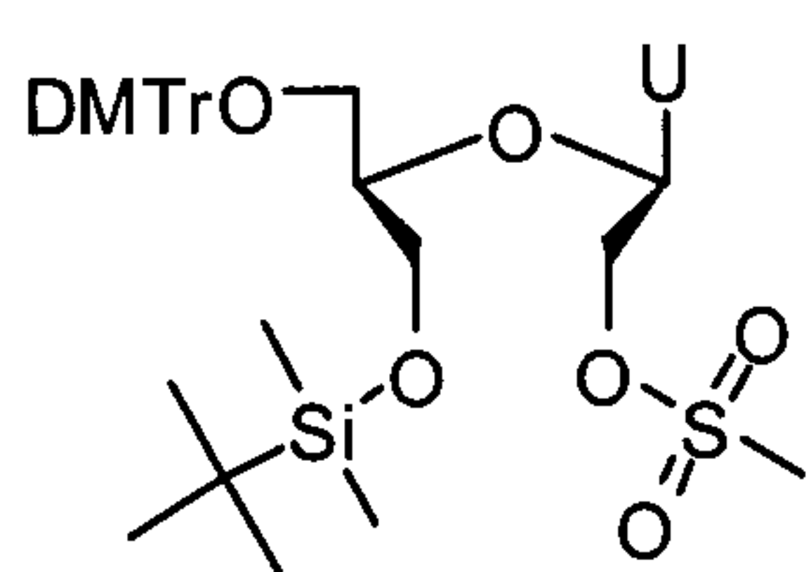
3'-O-tert-Butyldimethylsilyl-5'-O-(4,4'-dimethoxytrityl)-2'-O-methanesulfonyl-2',3'-secouridine (107)
