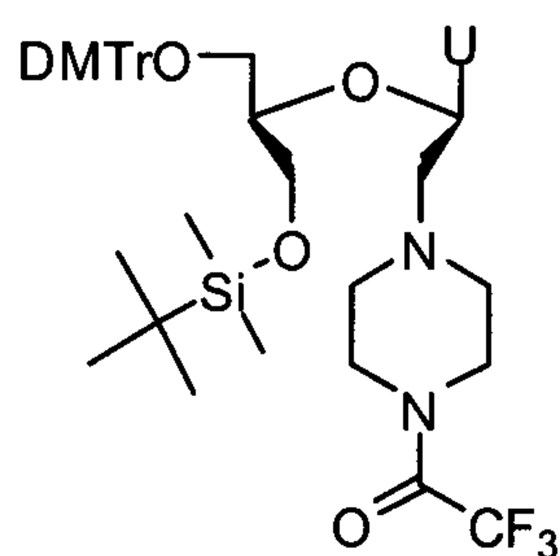
3'-O-tert-Butyldimethylsilyl-2'-deoxy-5'-O-(4,4'-dimethoxytrityl)-2'-(4-N-trifluoroacetyl)piperazino-2',3'-secouridine (109)
