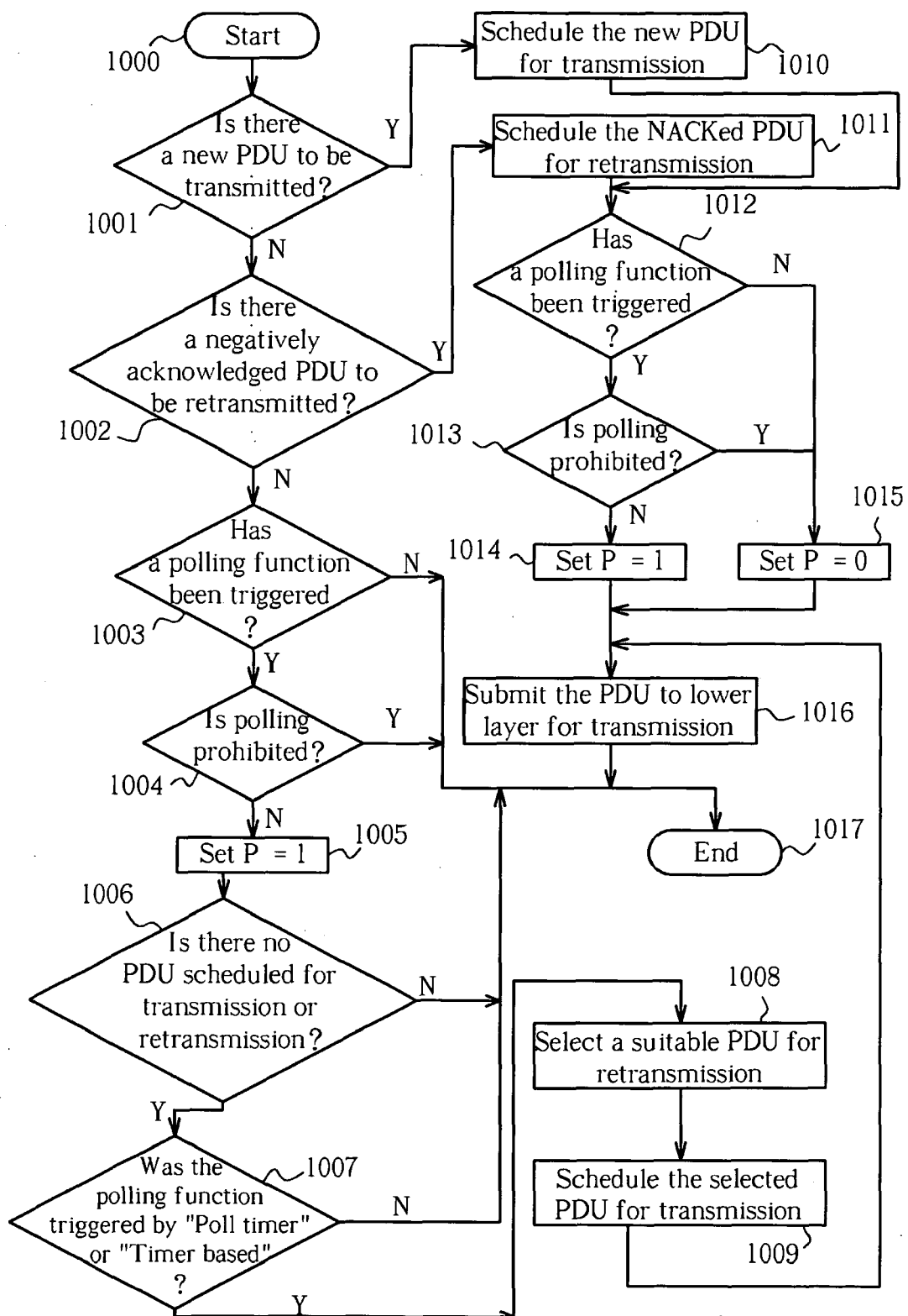
FIG. 4 PRIOR ART
