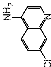
7-Chloro-4-aminoquinoline
