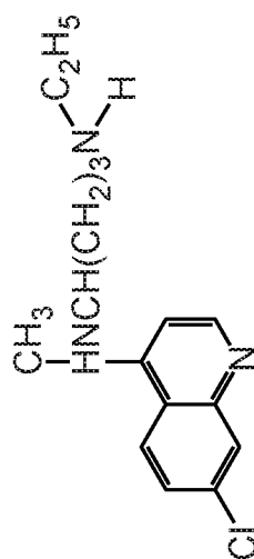
Desethyl-chloroquine
