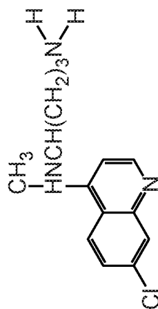
Bisesethyl-chloroquine
