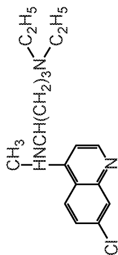
Chloroquine
