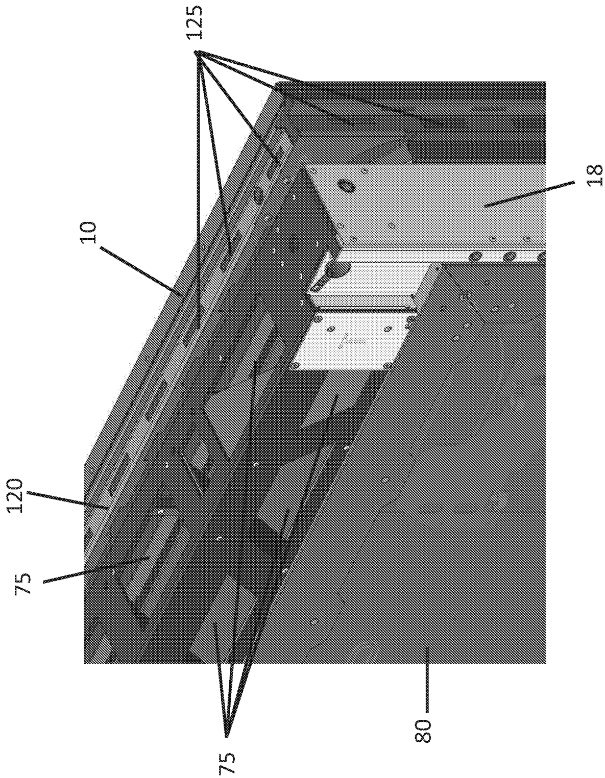
Figure 15
