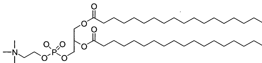
DSPC structure
