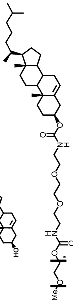
Cholesterol-PEG
