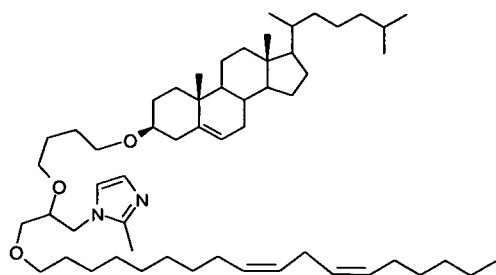
CLin-2MeIm
