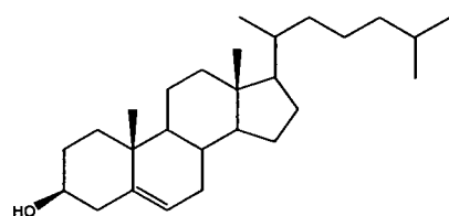
Cholesterol structure
