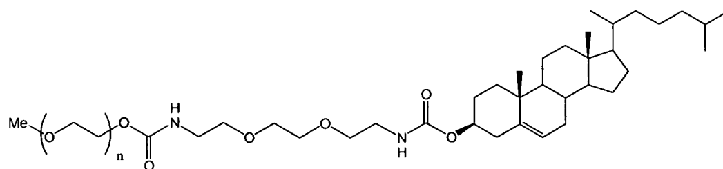
2KPEG-Cholesterol structure
