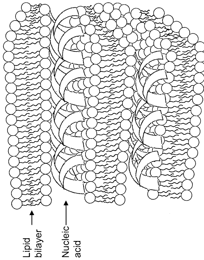
Lamellar Structure
