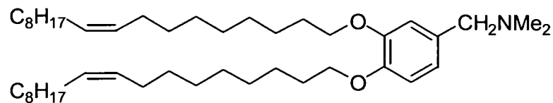
DMLBA structure
