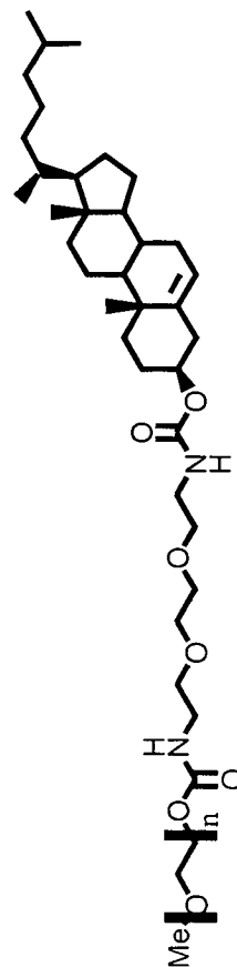
2KPEG-Chol (2%)
