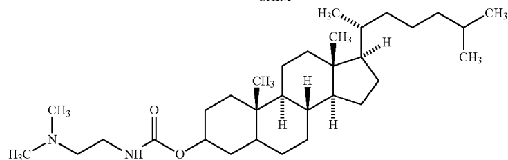
DC-CHOL
