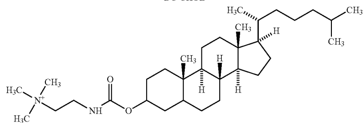
TC-CHOL
