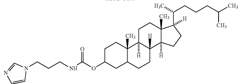
CHIM
