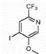
N-(1-(2-hydroxy-2-methylpropyl)-3-(5-methyl-2-(trifluoromethyl)pyridin-4-yl)-1H-pyrazol-4-yl)pyrazolo[1,5-a]pyrimidine-3-carboxamide
