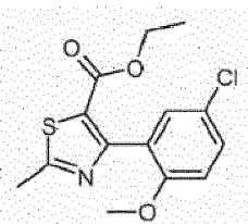
ethyl 4-(5-chloro-2-methoxyphenyl)-2-methylthiazole-5-carboxylate
