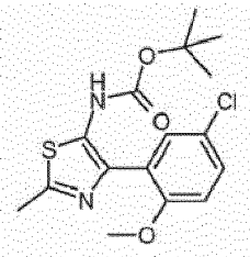
tert-butyl 4-(5-chloro-2-methoxyphenyl)-2-methylthiazol-5-ylcarbamate
