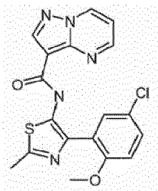
N-(4-(5-chloro-2-methoxyphenyl)-2-methylthiazol-5-yl)pyrazolo[1,5-a]pyrimidine-3-carboxamide
