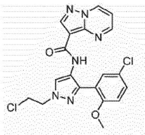
N-(3-(5-Chloro-2-methoxyphenyl)-1-(2-chloroethyl)-1H-pyrazol-4-yl)pyrazolo[1,5-a]pyrimidine-3-carboxamide
