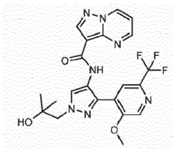
N-(1-(2-hydroxy-2-methylpropyl)-3-(5-methoxy-2-(trifluoromethyl)pyridin-4-yl)-1H-pyrazol-4-yl)pyrazolo[1,5-a]pyrimidine-3-carboxamide
