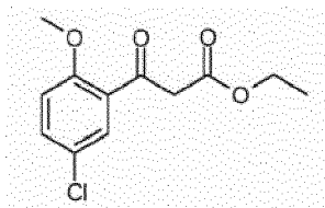
ethyl 3-(5-chloro-2-methoxyphenyl)-3-oxopropanoate
