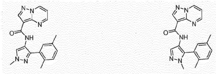
N-(3-(2,5-dimethylphenyl)-1-methyl-1H-pyrazol-4-yl)pyrazolo[1,5-a]pyrimidine-3-carboxamide
