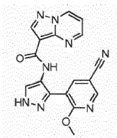
N-(3-(5-Cyano-2-methoxypyridin-3-yl)-1H-pyrazol-4-yl)pyrazolo[1,5-a]pyrimidine-3-carboxamide
