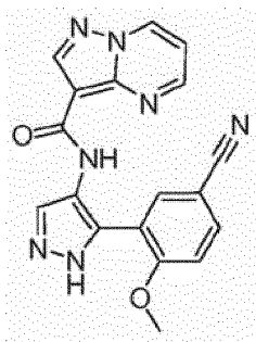
N-(5-(5-cyano-2-methoxyphenyl)-1H-pyrazol-4-yl)pyrazolo[1,5-a]pyrimidine-3-carboxamide
