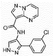
N-(3-(3-chlorophenyl)-1H-pyrazol-4-yl)pyrazolo[1,5-a]pyrimidine-3-carboxamide
