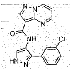
N-(3-(3-chlorophenyl)-1H-pyrazol-4-yl)pyrazolo[1,5-a]pyrimidine-3-carboxamide
