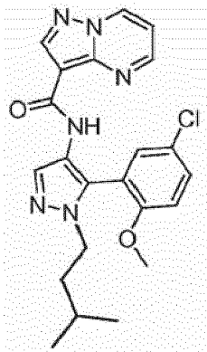
N-(5-(5-chloro-2-methoxyphenyl)-1-isopentyl-1H-pyrazol-yl)pyrazolo[1,5-a]pyrimidine-3-carboxamide
