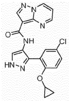
N-(3-(5-chloro)-2-cyclopropoxyphenyl)-1H-pyrazol-4-yl)pyrazolo[1,5-a]pyrimidine-3-carboxamide
