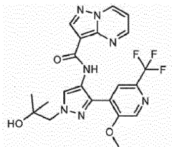
N-(1-(2-hydroxy-2-methylpropyl)-3-(5-methyl-2-(trifluoromethyl)pyridin-4-yl)-1H-pyrazol-4-yl)pyrazolo[1,5-a]pyrimidine-3-carboxamide
