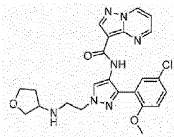
N-(3-(5-Chloro-2-methoxyphenyl)-1-(2-(tetrahydrofuran-3-ylamino)ethyl)-1H-pyrazol-4-yl)pyrazolo[1,5-a]pyrimidine-3-carboxamide
