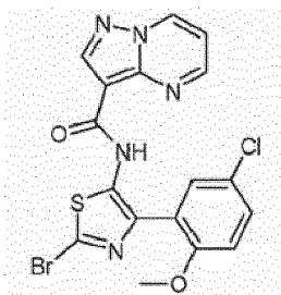
N-(2-bromo-4-(5-chloro-2-methoxyphenyl)thiazol-5-yl)pyrazolo[1,5-a]pyrimidine-3-carboxamide
