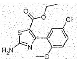
ethyl 2-amino-4-(5-chloro-2-methoxyphenyl)thiazole-5-carboxylate
