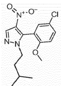
N-(5-(5-chloro-2-methoxyphenyl)-1-isopentyl-4-nitro-1H-pyrazole
