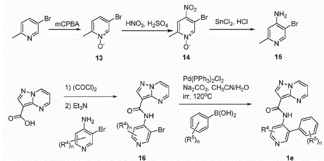
Reaction Scheme 4
