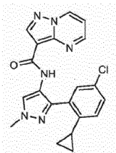
N-(3-(5-chloro-2-cyclopropylphenyl)-1-methyl-1H-pyrazol-4-yl)pyrazolo[1,5-a]pyrimidine-3-carboxamide
