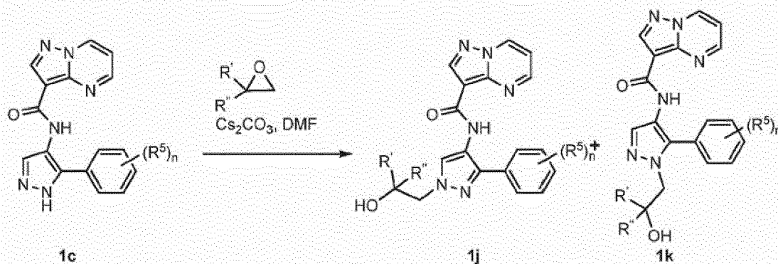
Reaction Scheme 10
