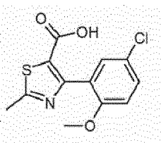
4-(5-chloro-2-methoxyphenyl)-2-methylthiazole-5-carboxylic acid
