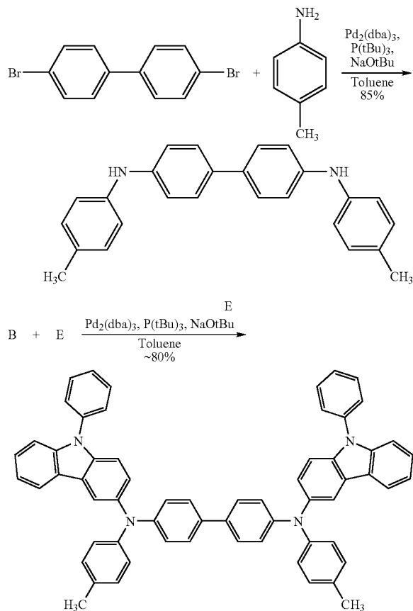
Reaction Scheme 3
