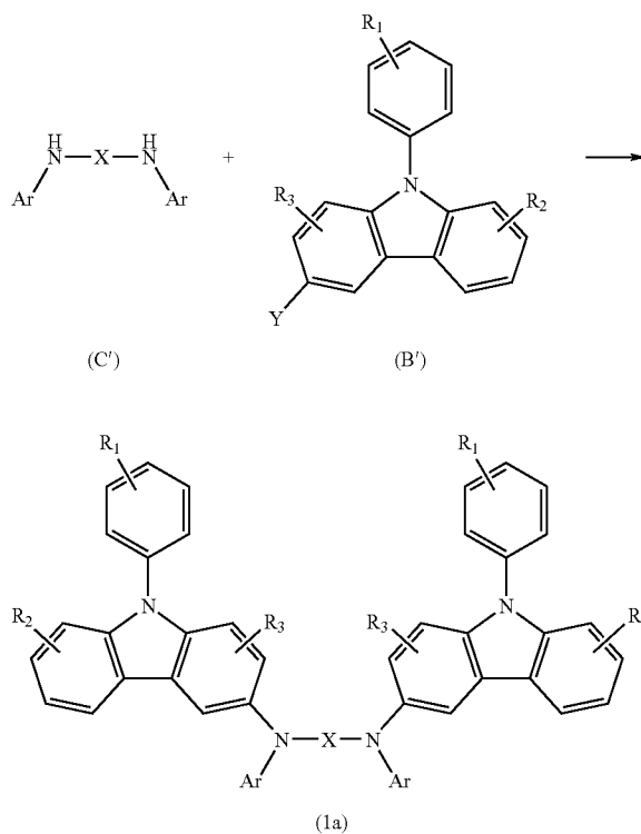
Reaction Scheme 1
