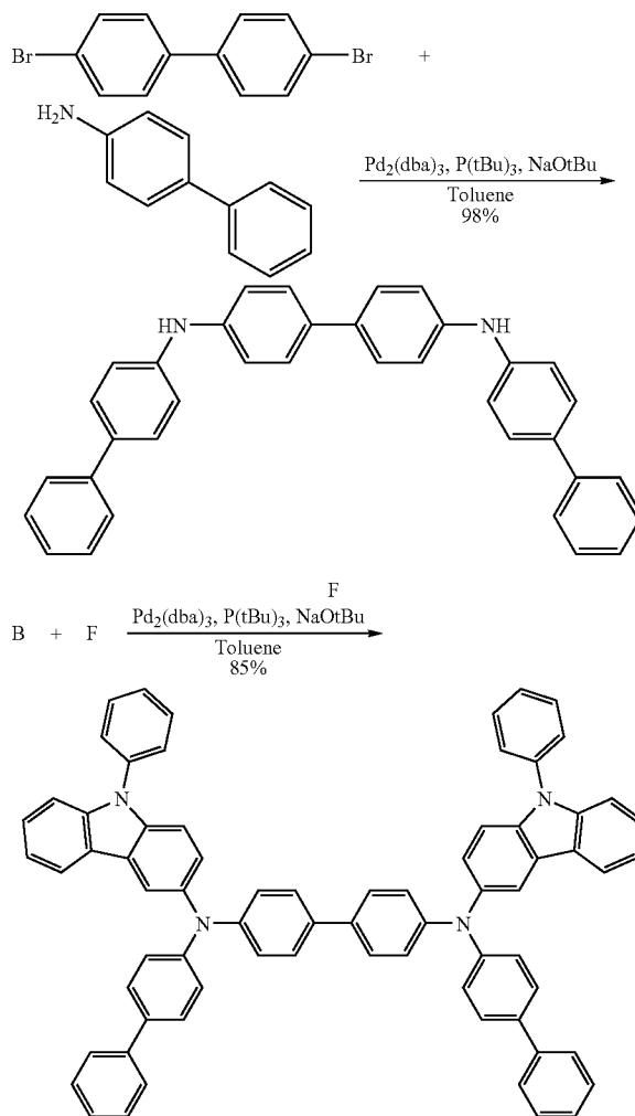
Reaction Scheme 5
