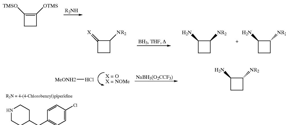
Scheme 1. Synthesis of Cyclobutamines-Ring A = Phenyl.
