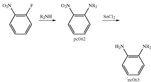
Scheme 5. Synthesis of Aniline - Ring A = Phenyl.
