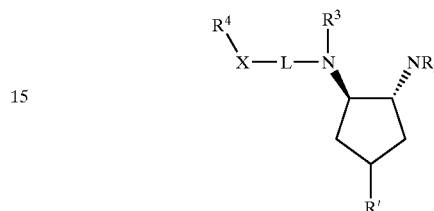
Scheme 6. Synthesis of Cycloalkyl Derivatives.
