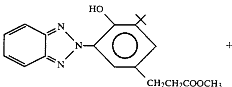
methyl-3-(3-(2H-benzotriazol 2-yl))-5-tert-butyl-4-hydroxyphenyl)propionate
