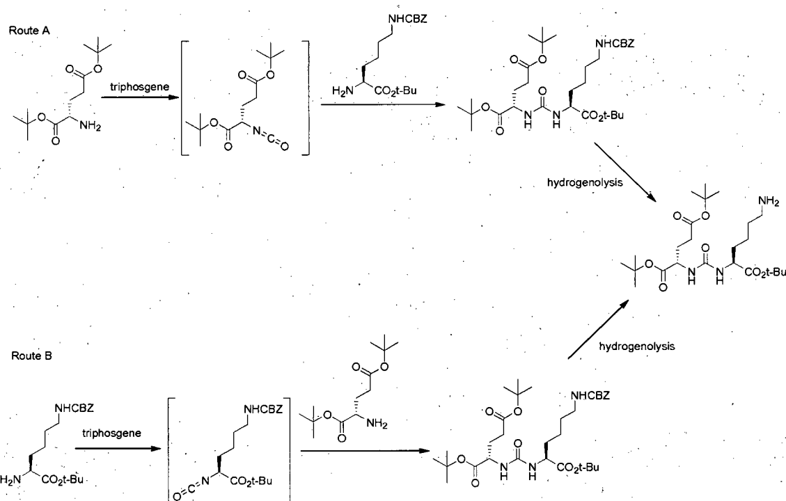
Scheme 2.
