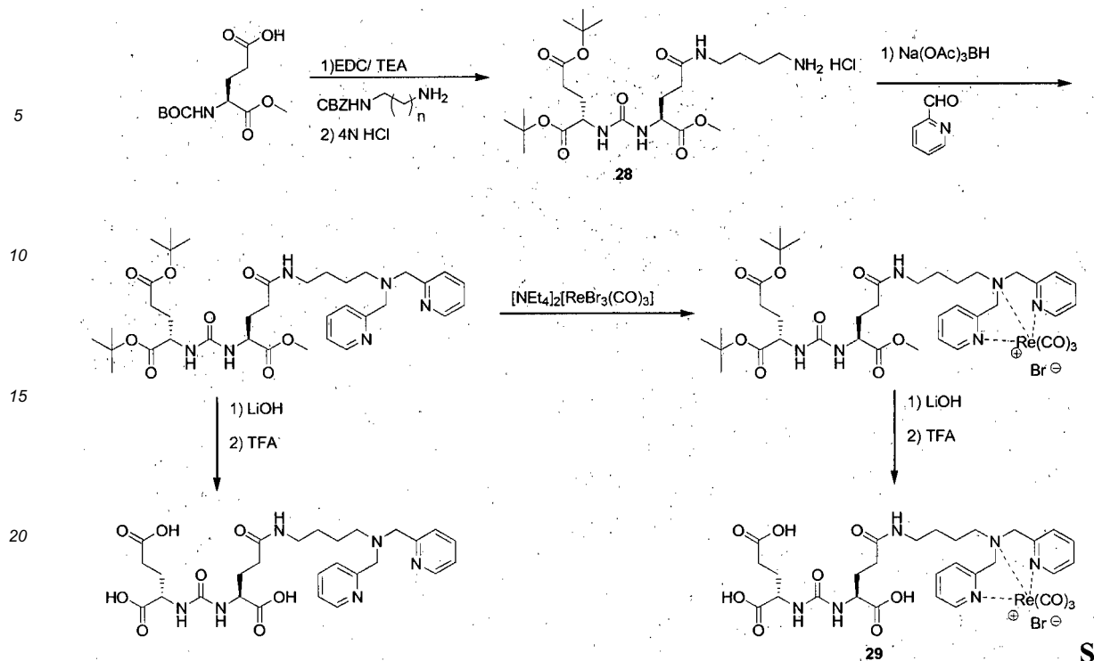
Scheme 4.
