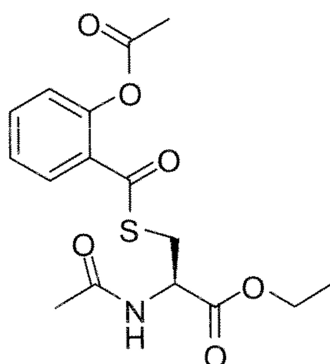
(R)-ethyl 2-acetamido-3-(2-acetoxybenzoylthio)propanoate
