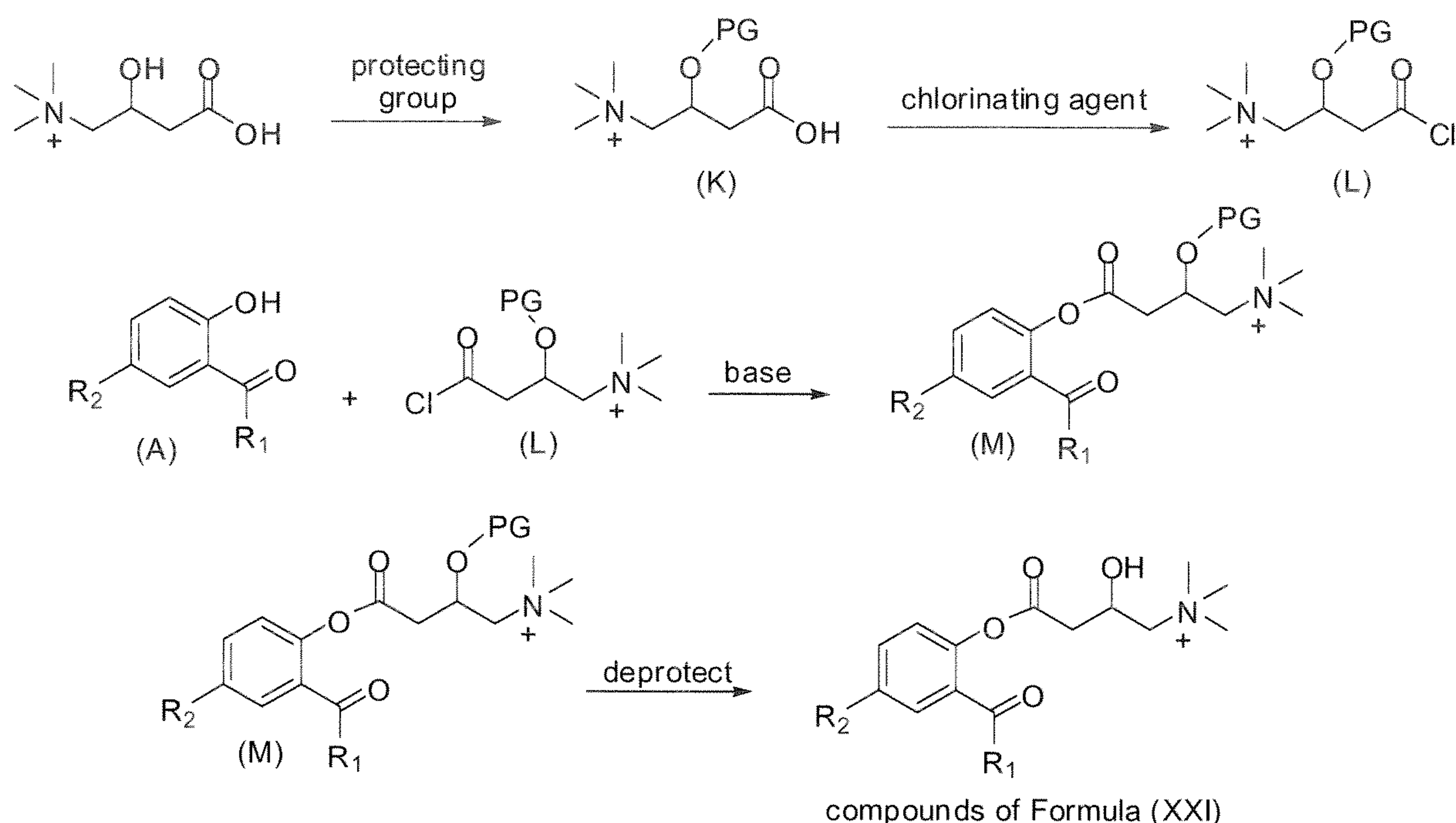
Scheme 10
