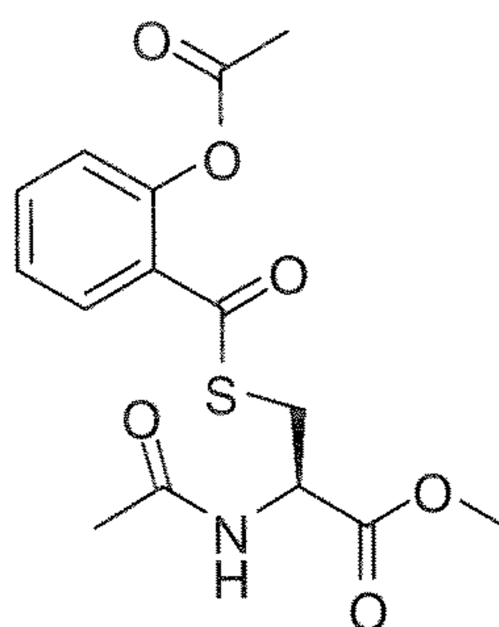
(R)-methyl 2-acetamido-3-(2-acetoxybenzoylthio)propanoate
