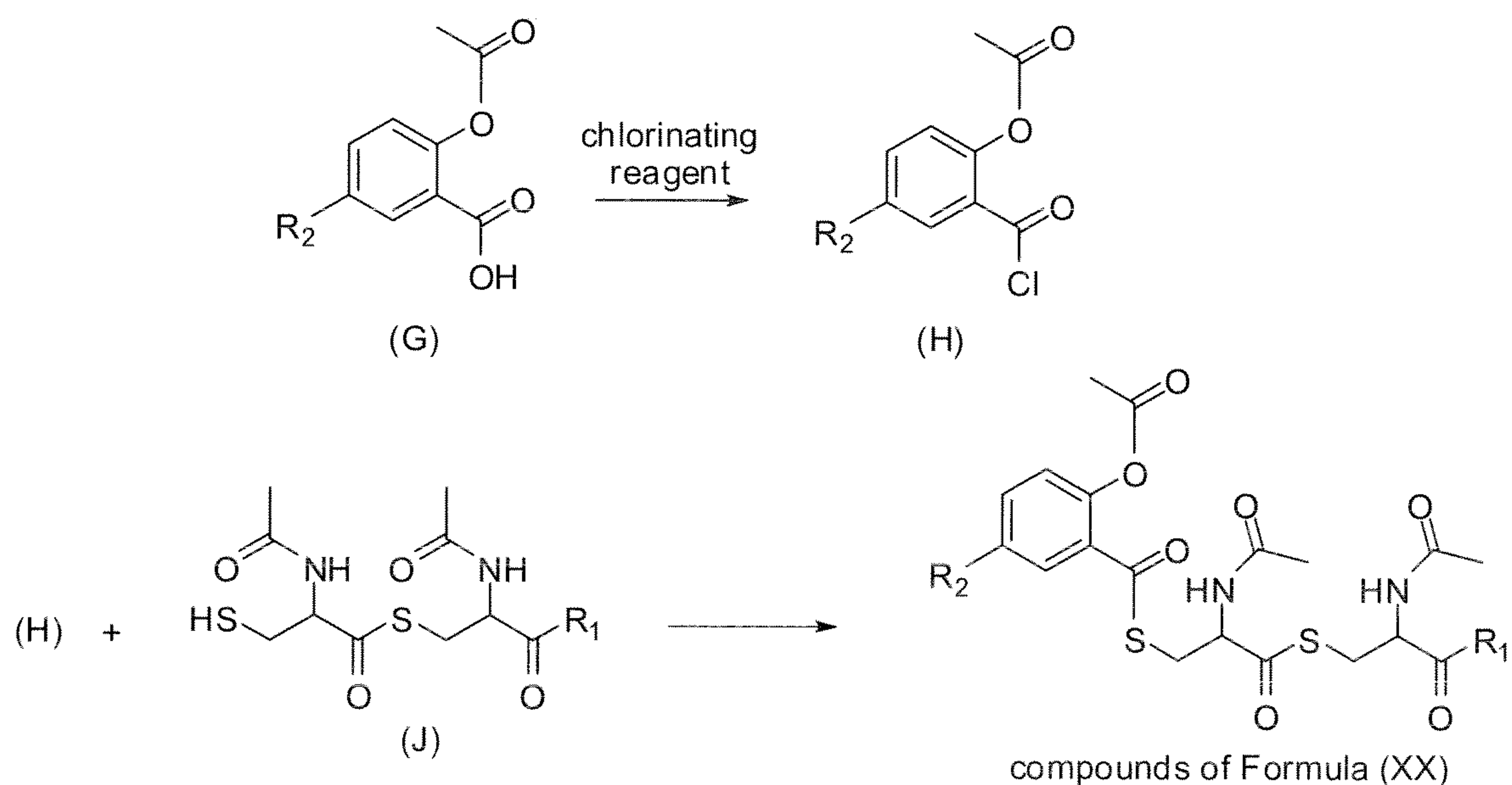
Scheme 9
