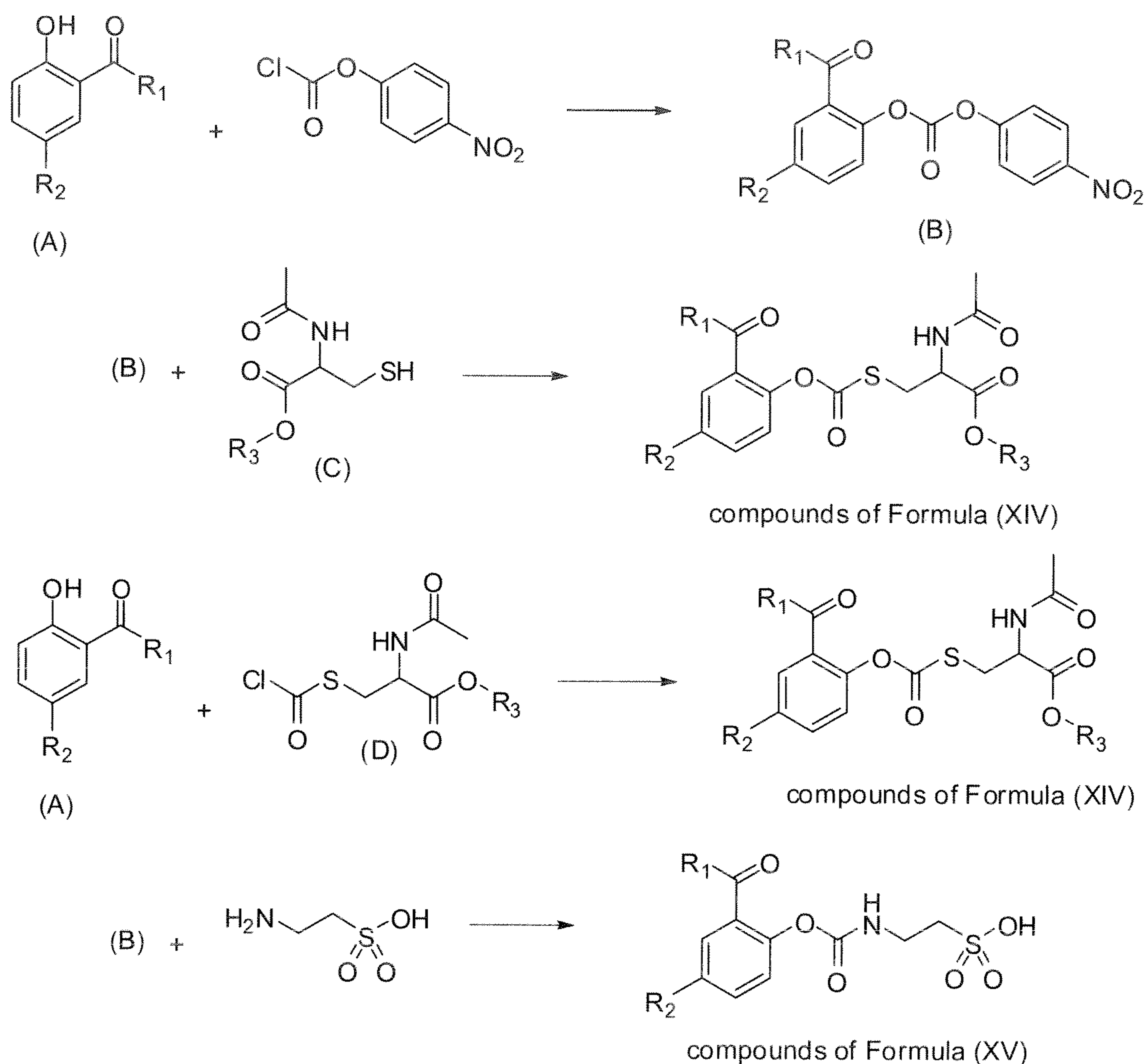
Scheme 6
