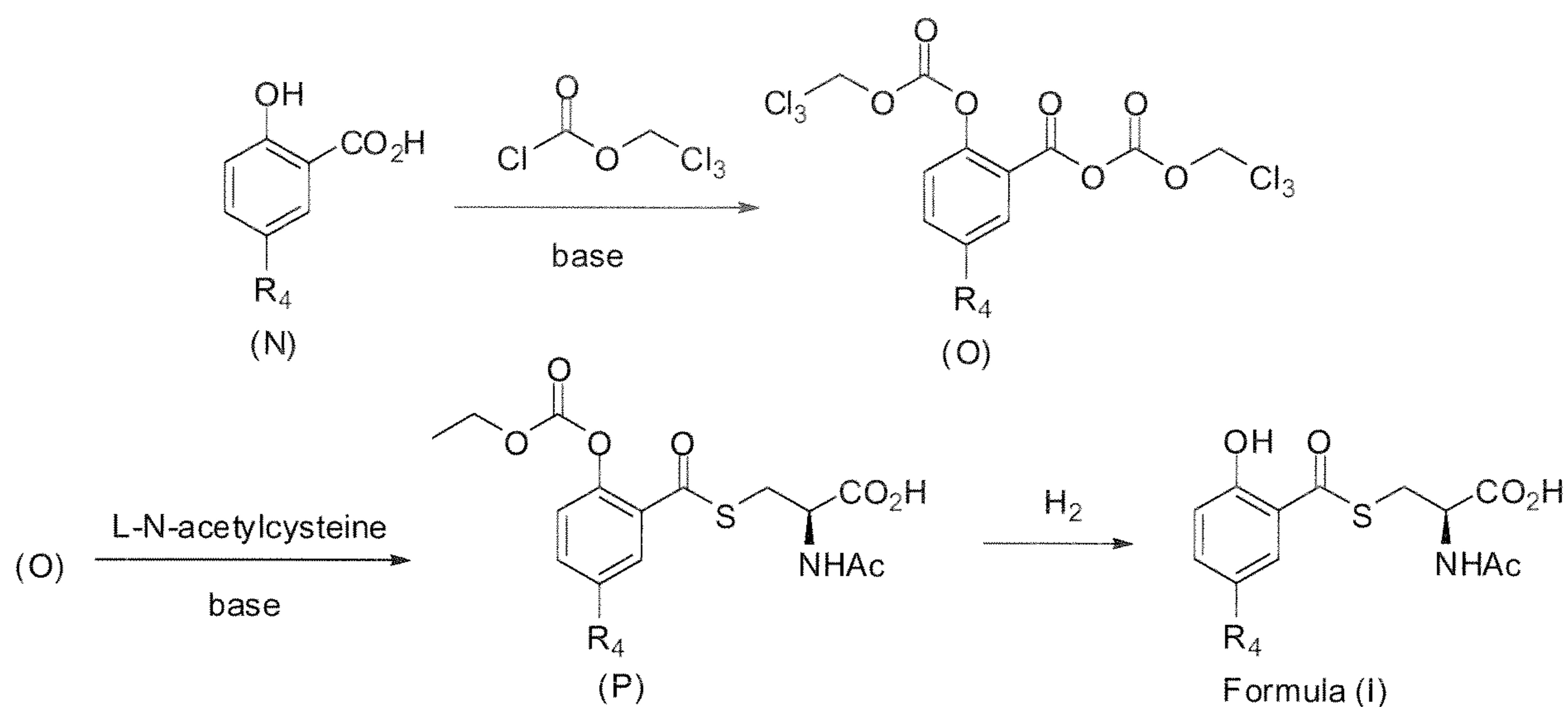
Scheme 11
