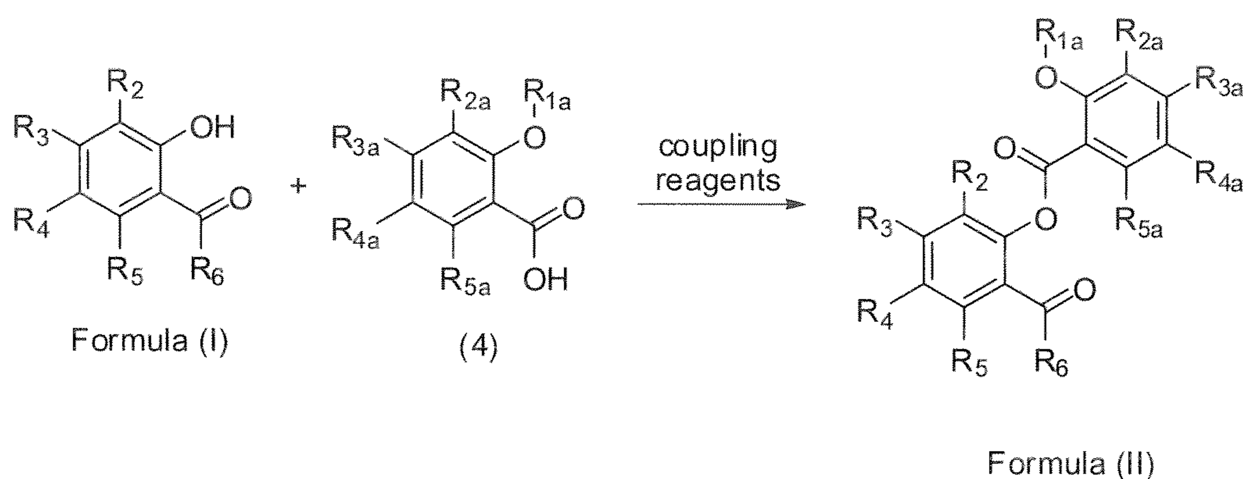
Scheme 3
