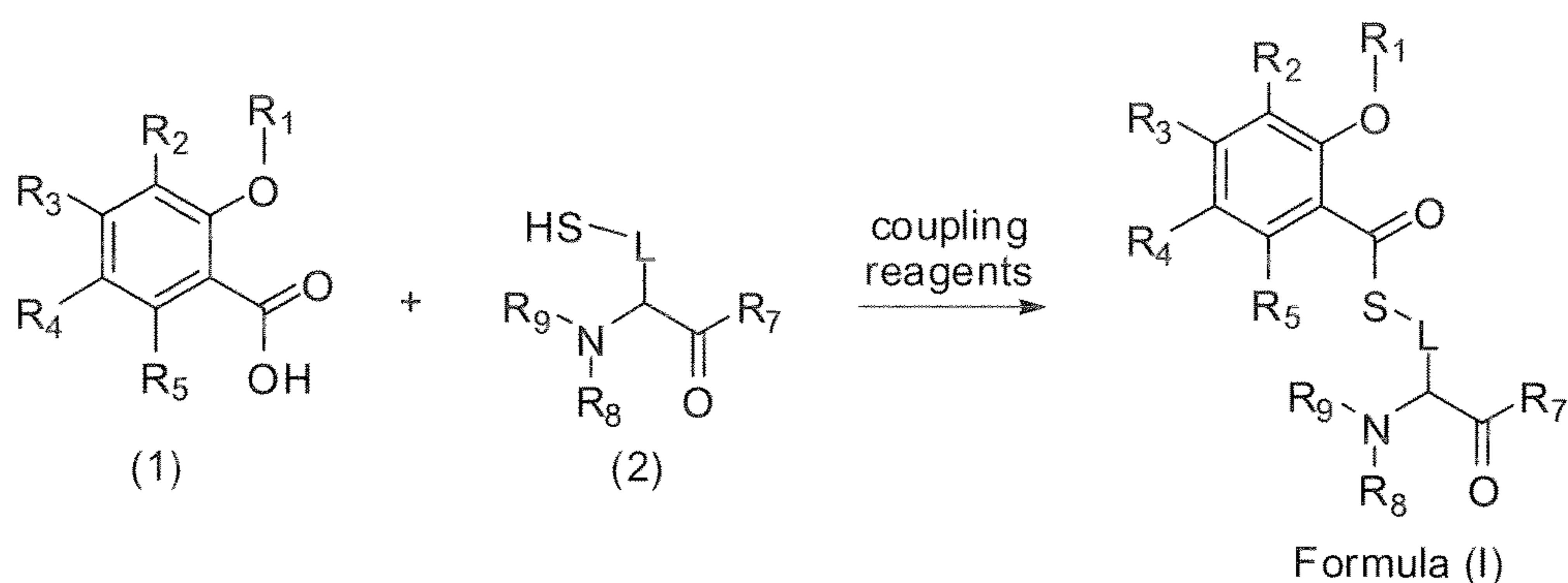
Scheme 1
