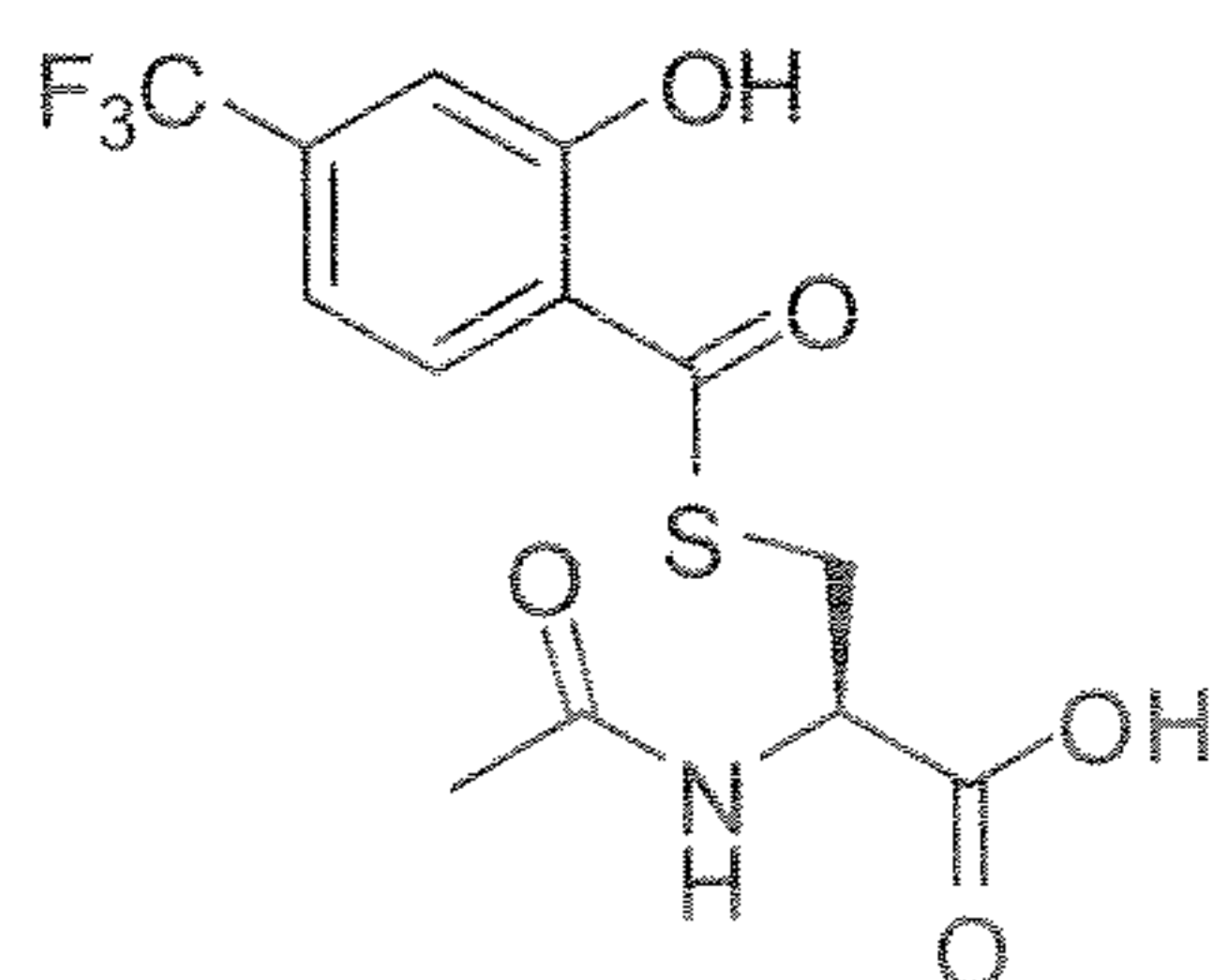
(R)-2-acetamido-3-(2-hydroxy-4-(trifluoromethyl)benzoylthio)propanoic acid
