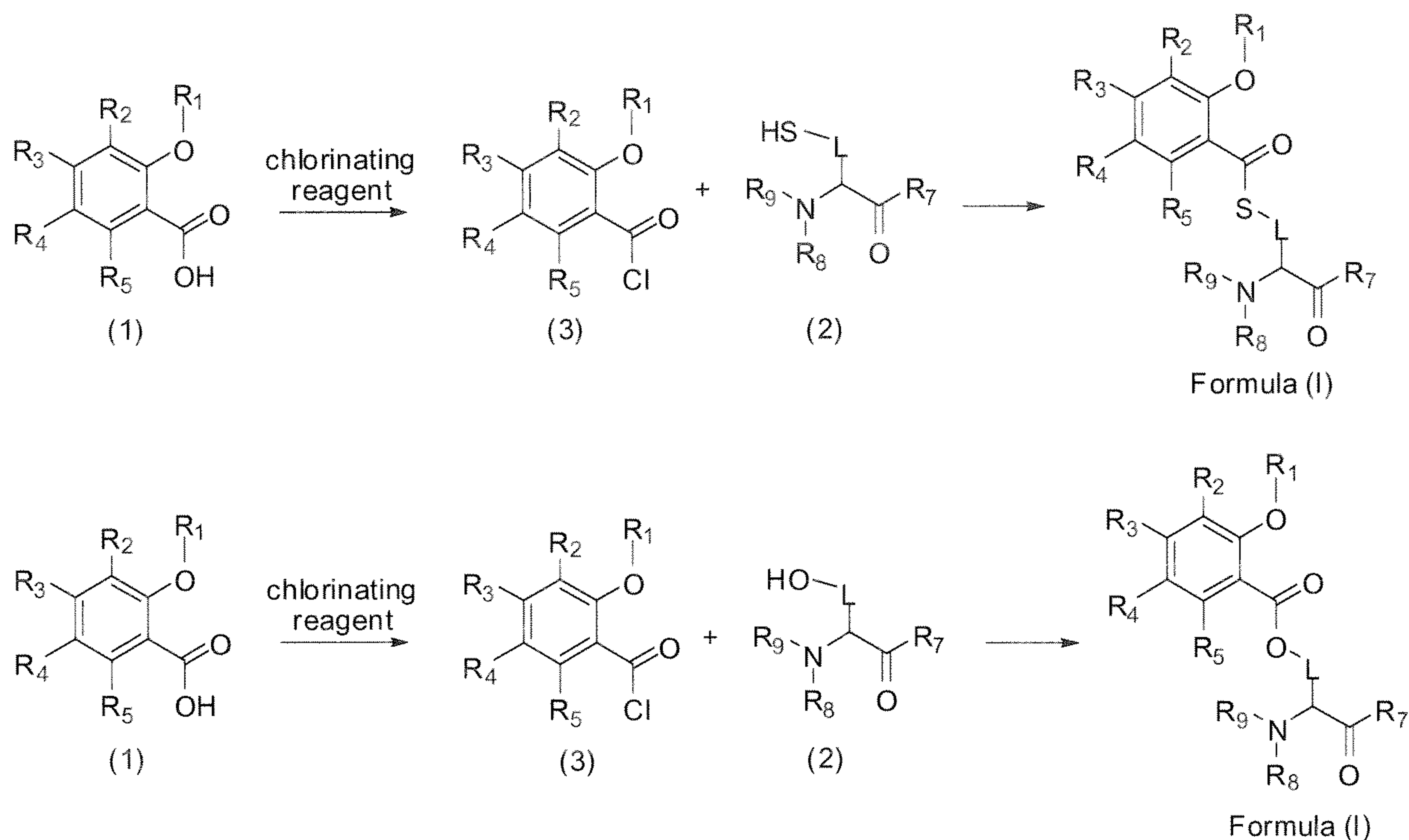
Scheme 2
