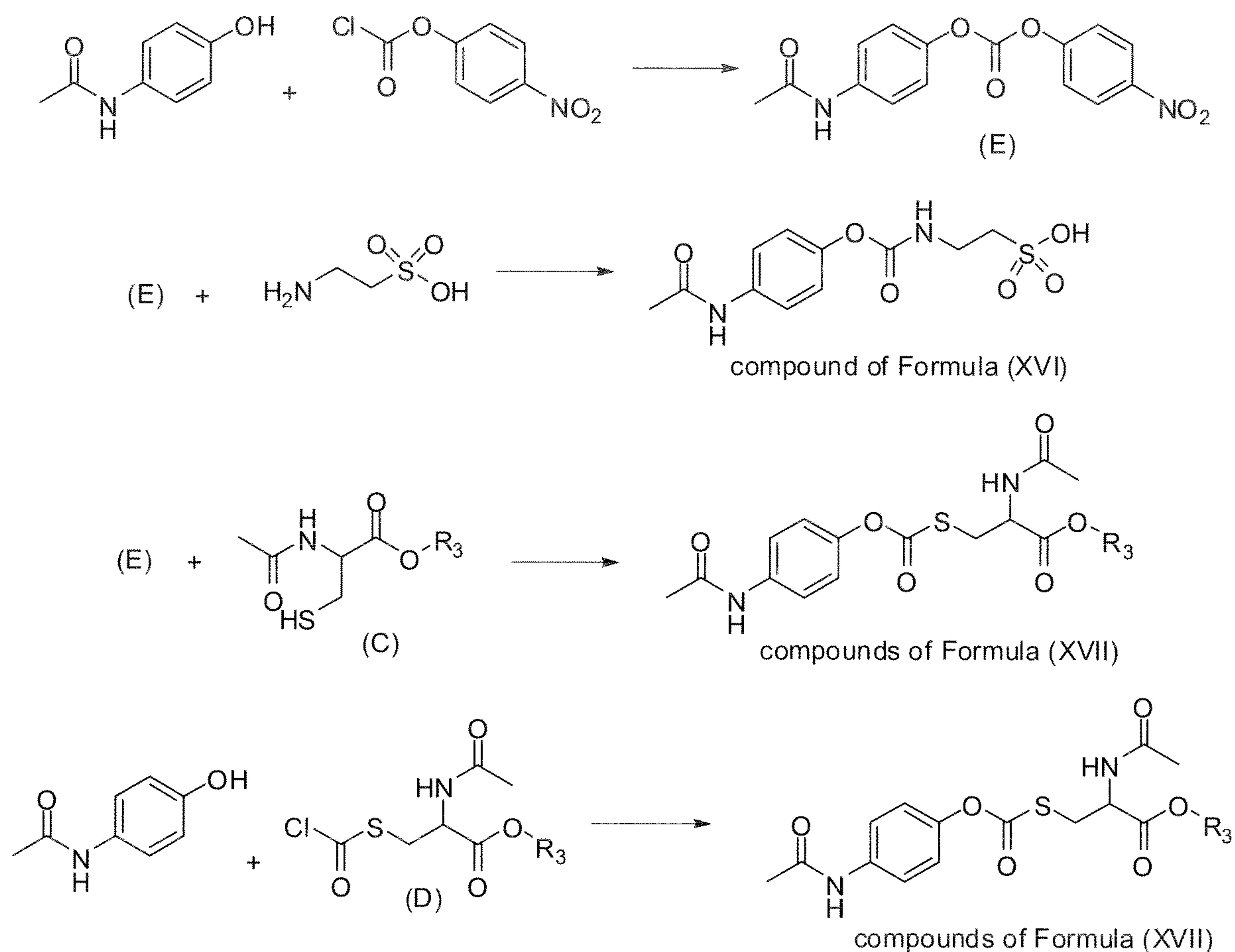
Scheme 7
