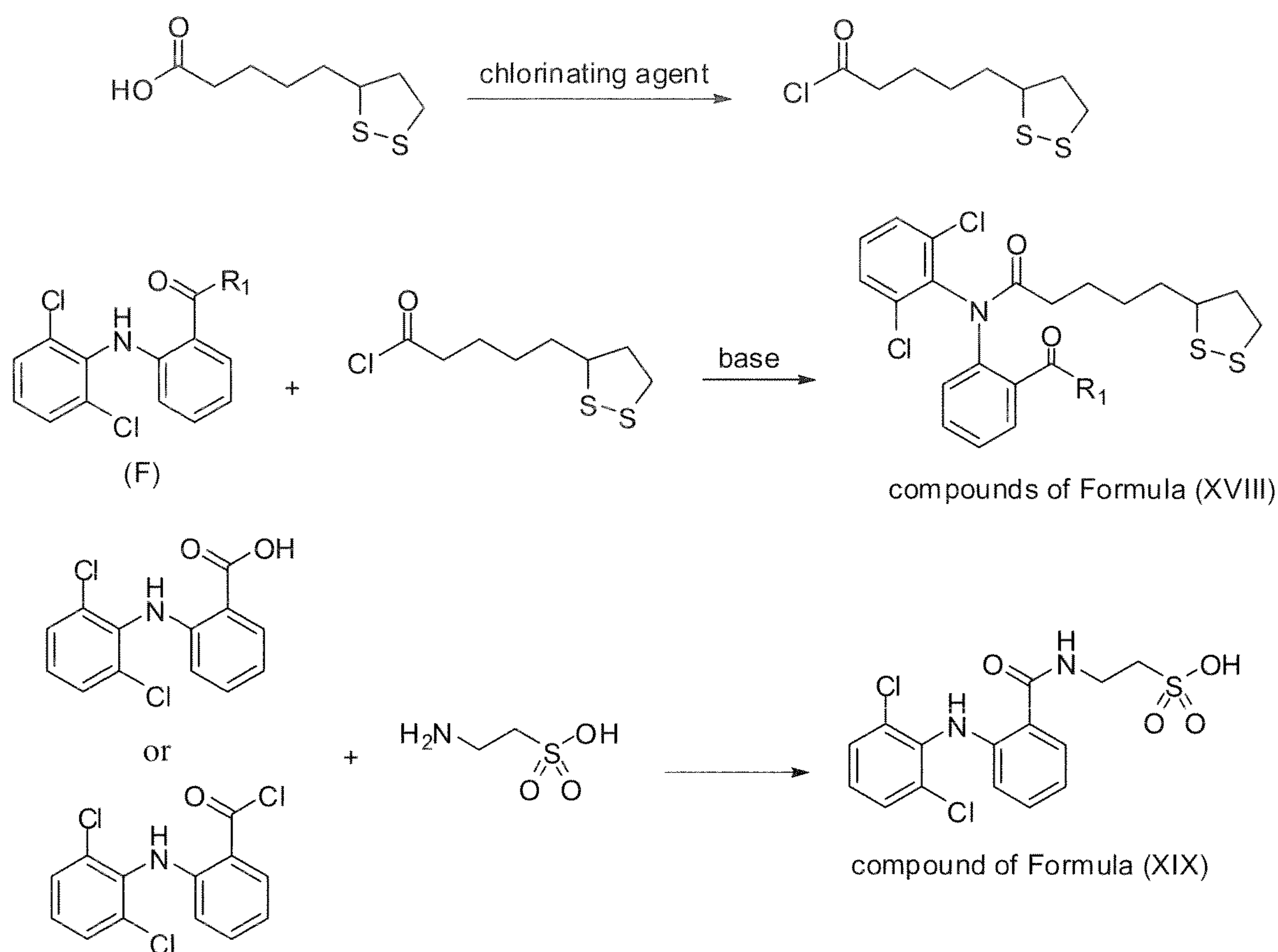
Scheme 8
