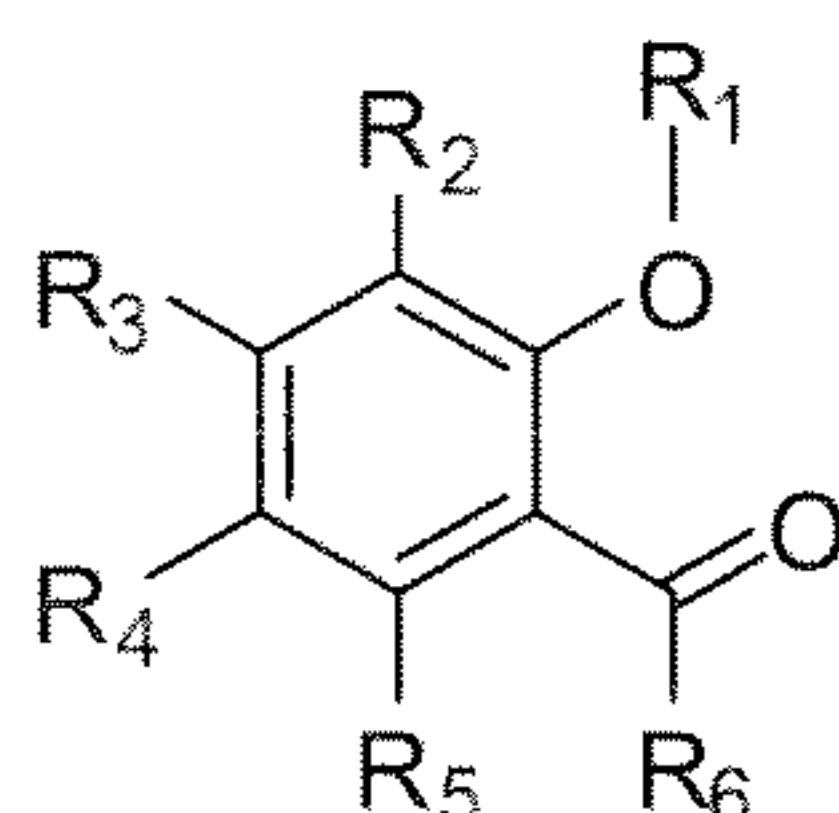
(I)
