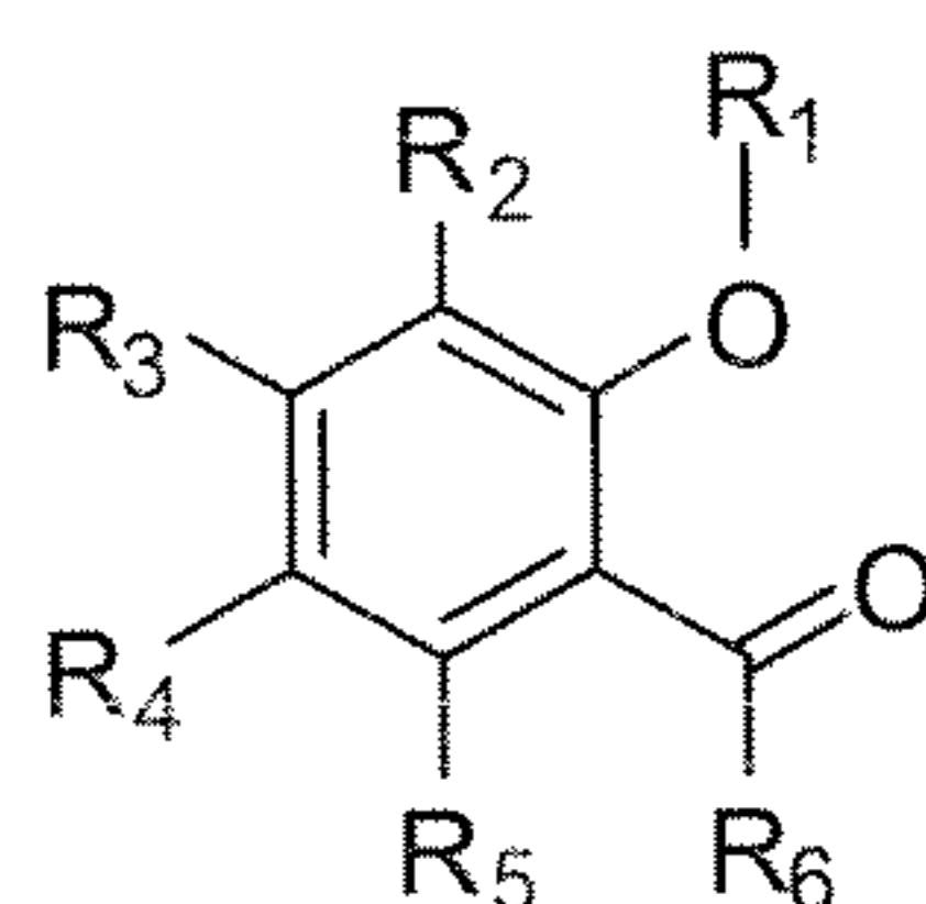
(I)
