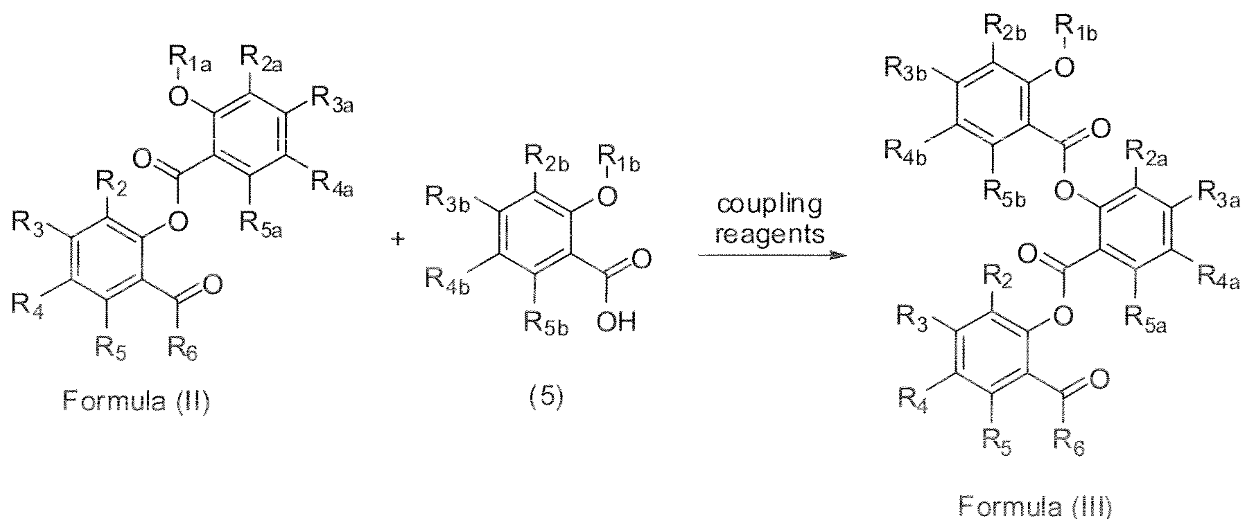
Scheme 4
