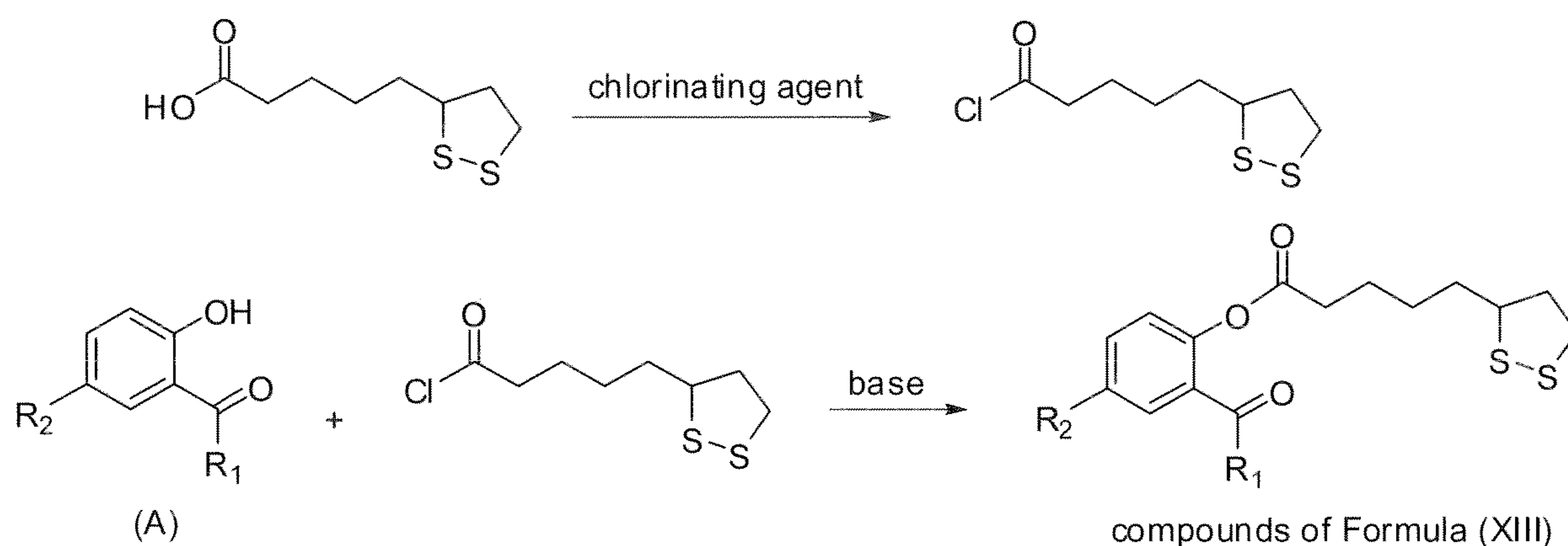
Scheme 5
