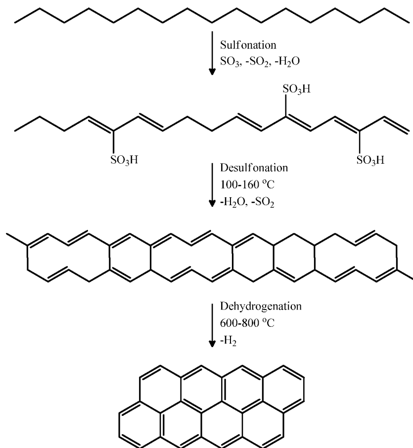
Scheme 1. The generic chemical process of a hydrocarbon reacting with SO 3 generating a polyacetylene-like polymer with sulfonic acid groups, a subsequent thermal step cross-linking the individual polymer chains, and dehydrogenation at elevated temperatures resulting in the desired carbonized polymer.
