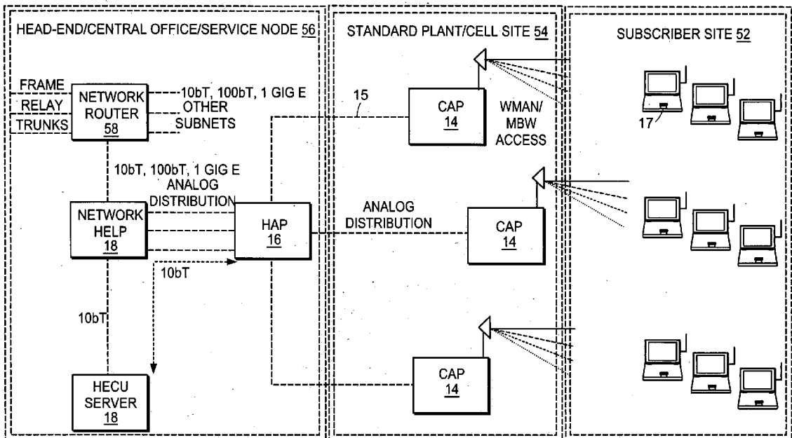
FUNCTIONAL LAN NETWORK 10
